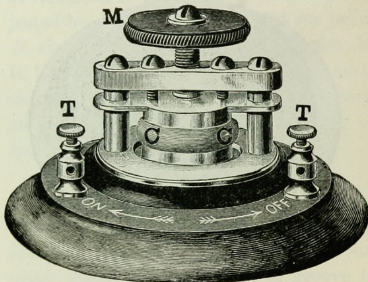
FIG. 120.—CARBON PRESSURE RHEOSTAT.
