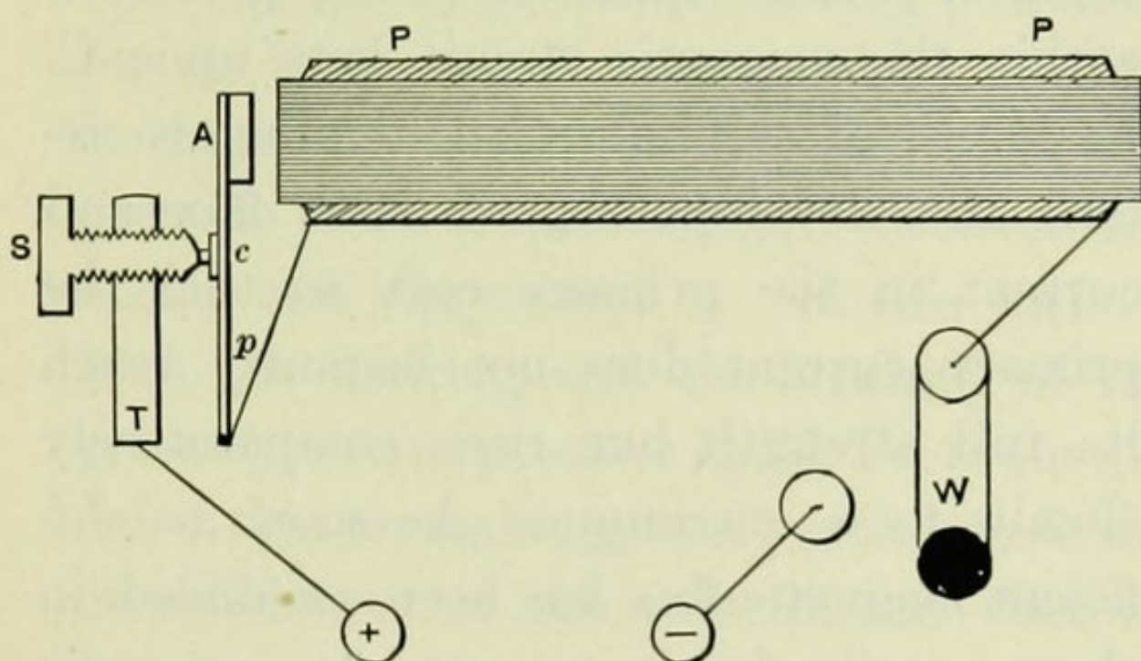
FIG. 96.—PRIMARY CONNECTIONS OF MEDICAL INDUCTION COIL.
