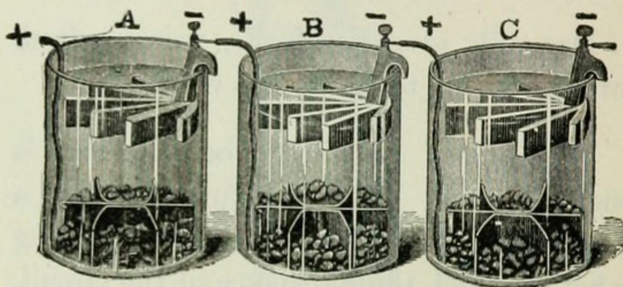
FIG. 17.—SERIES CONNECTION OF THREE DANIELL GRAVITY CELLS.
