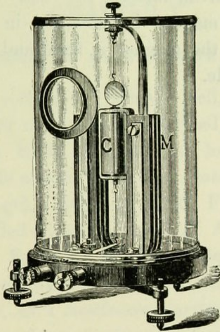
FIG. 38.—D'ARSONVAL GALVANOMETER.
