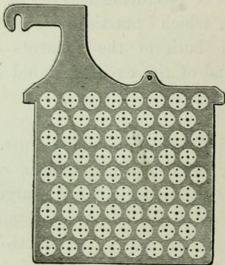
FIG. 21.—PLATE OF CHLORIDE STORAGE BATTERY.
