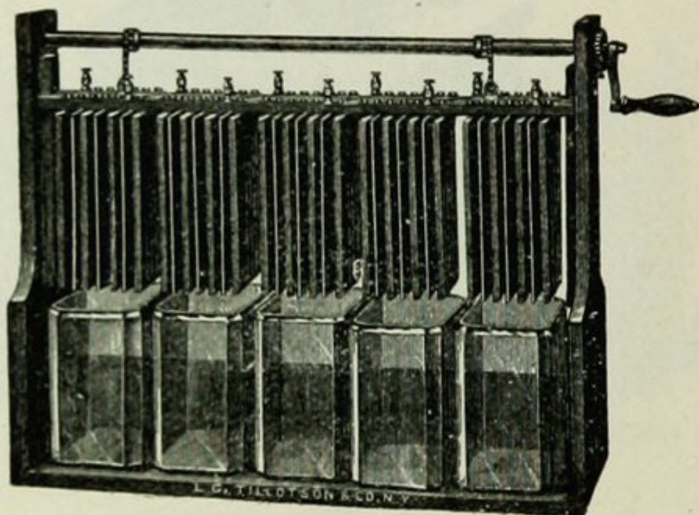
FIG. 19.—PLUNGE BATTERY.
