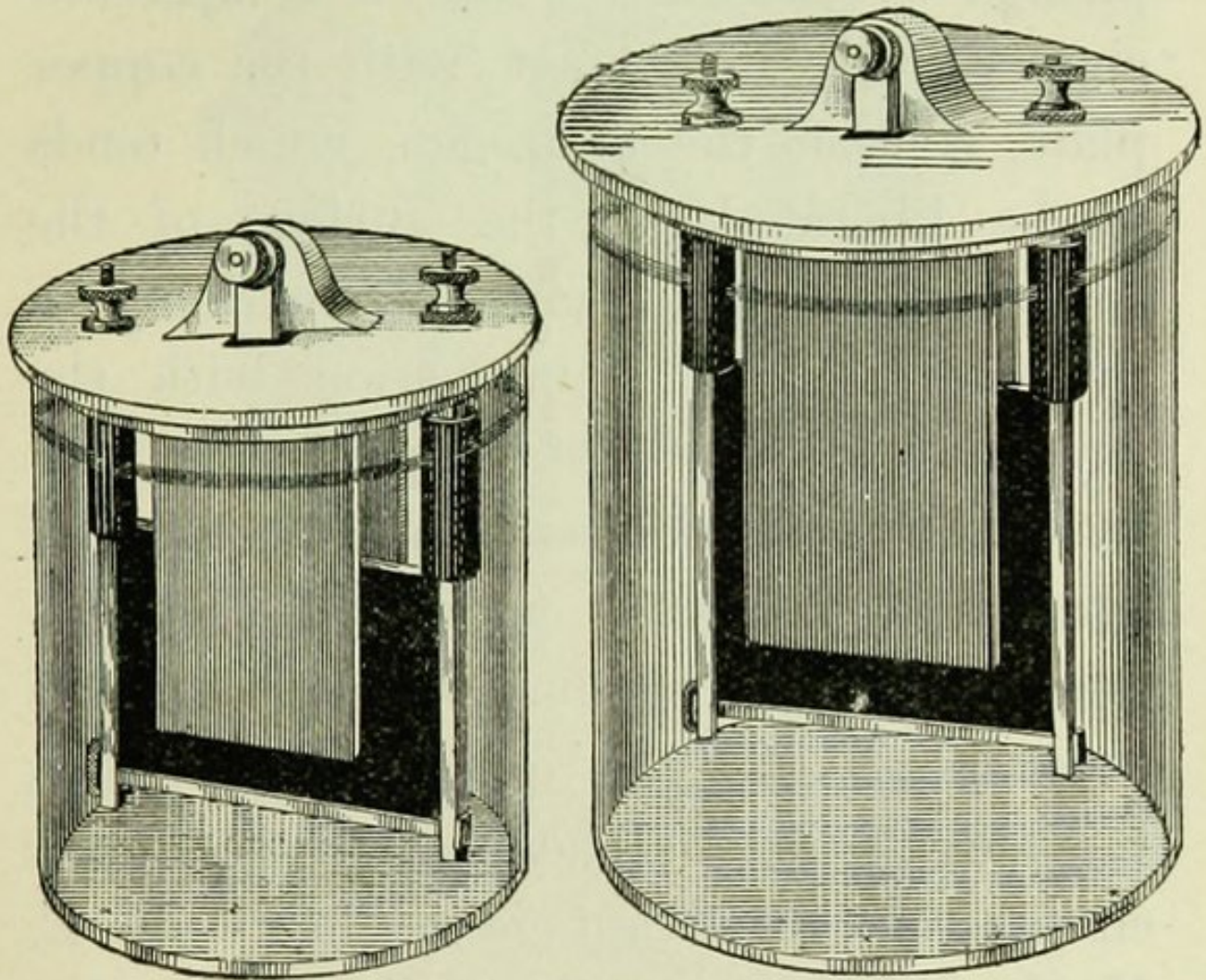
FIG. 13.—EDISON-LALANDE CELLS.
