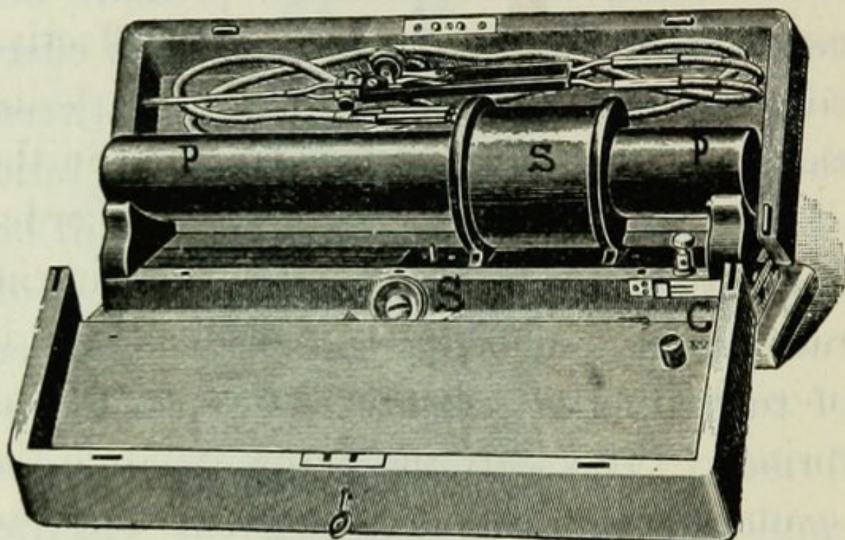
FIG. 113.—ALTERNATING-CURRENT TRANSFORMER FOR CAUTERY.
