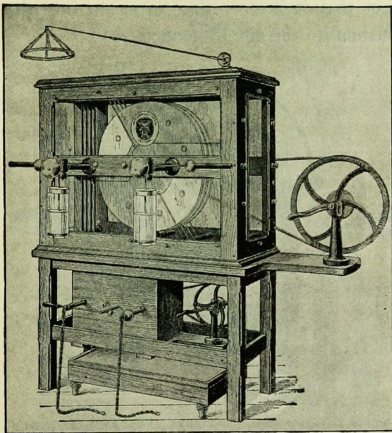
FIG. 71.—HOLTZ INFLUENCE MACHINE.
