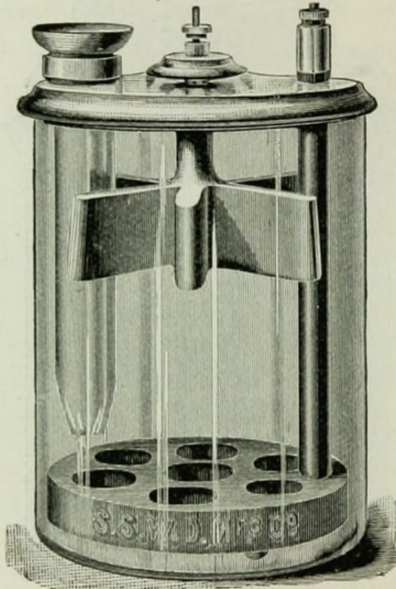
FIG. 15.—PARTZ GRAVITY CELL.
