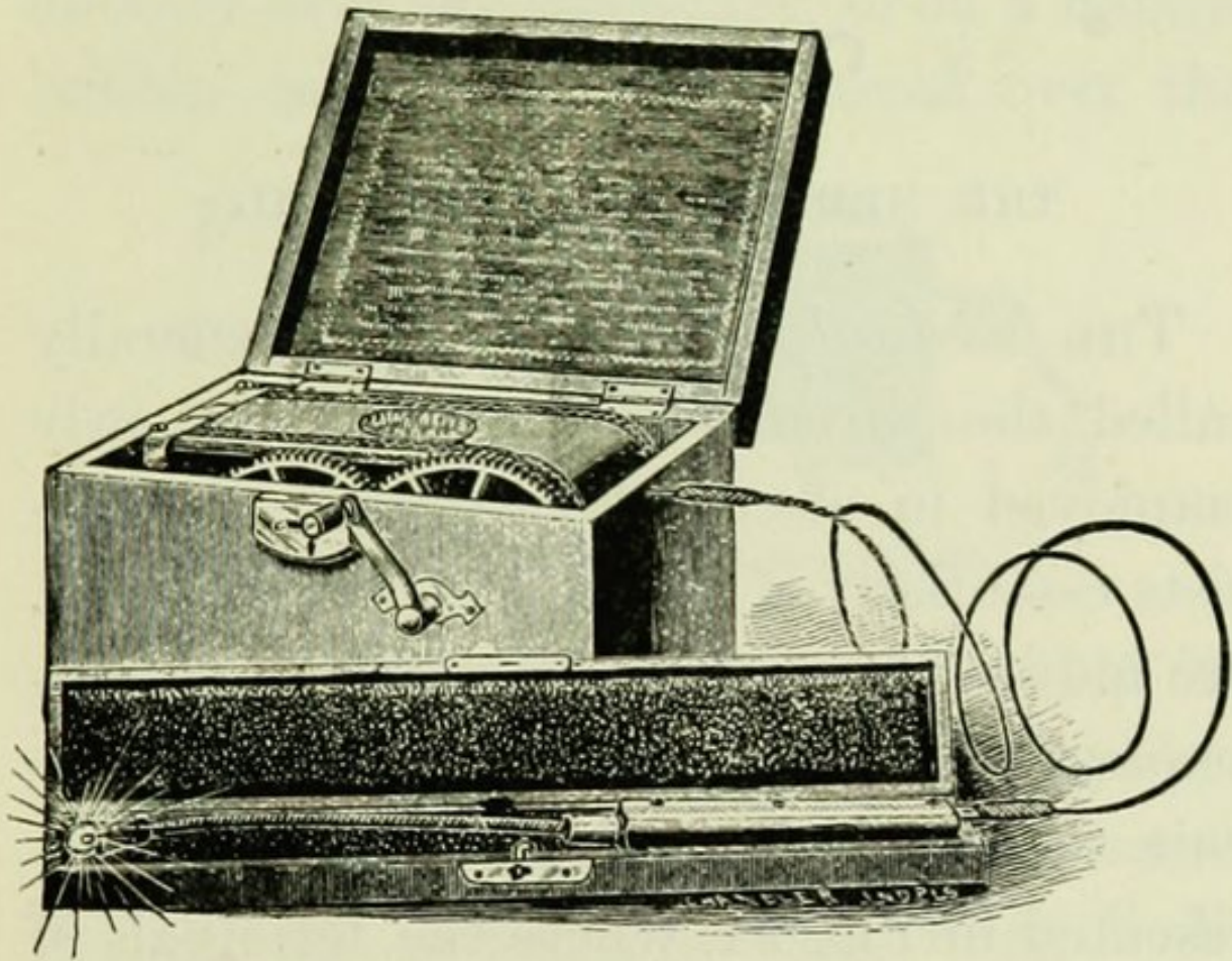
FIG. 93.—MAGNETO-ELECTRIC GENERATOR.
