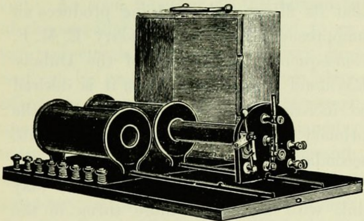
FIG. 98.—INDUCTION COIL, DUBOIS-RAYMOND TYPE.
