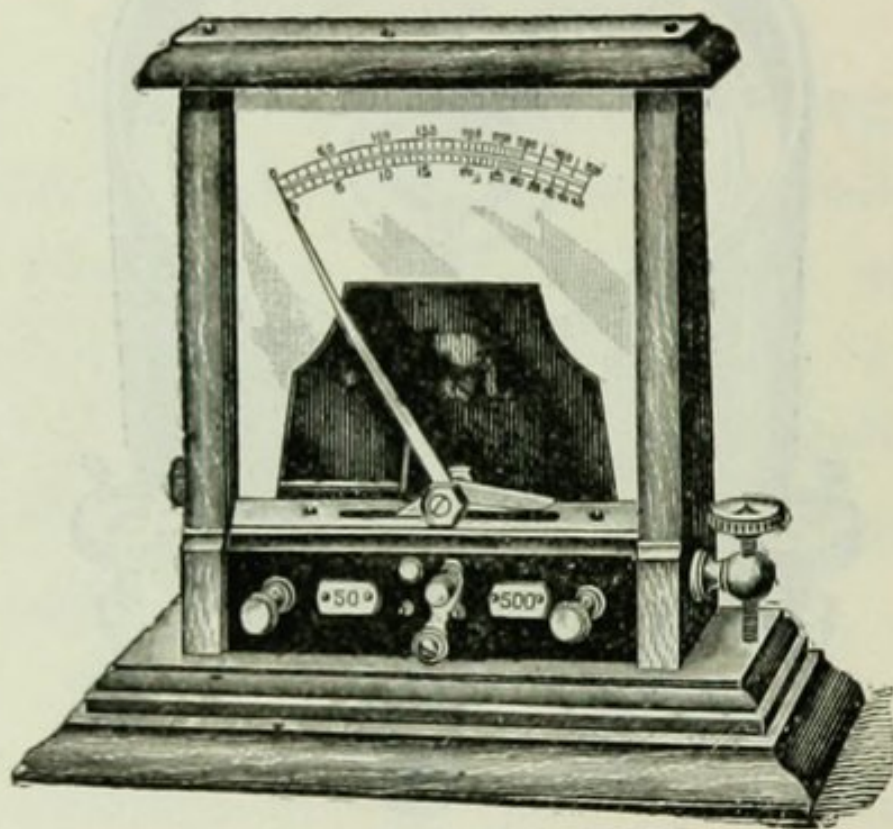
FIG. 31.—VERTICAL FORM OF MILLIAMMETER.
