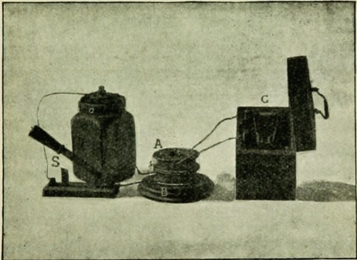
FIG. 86.—MUTUAL INDUCTION.
