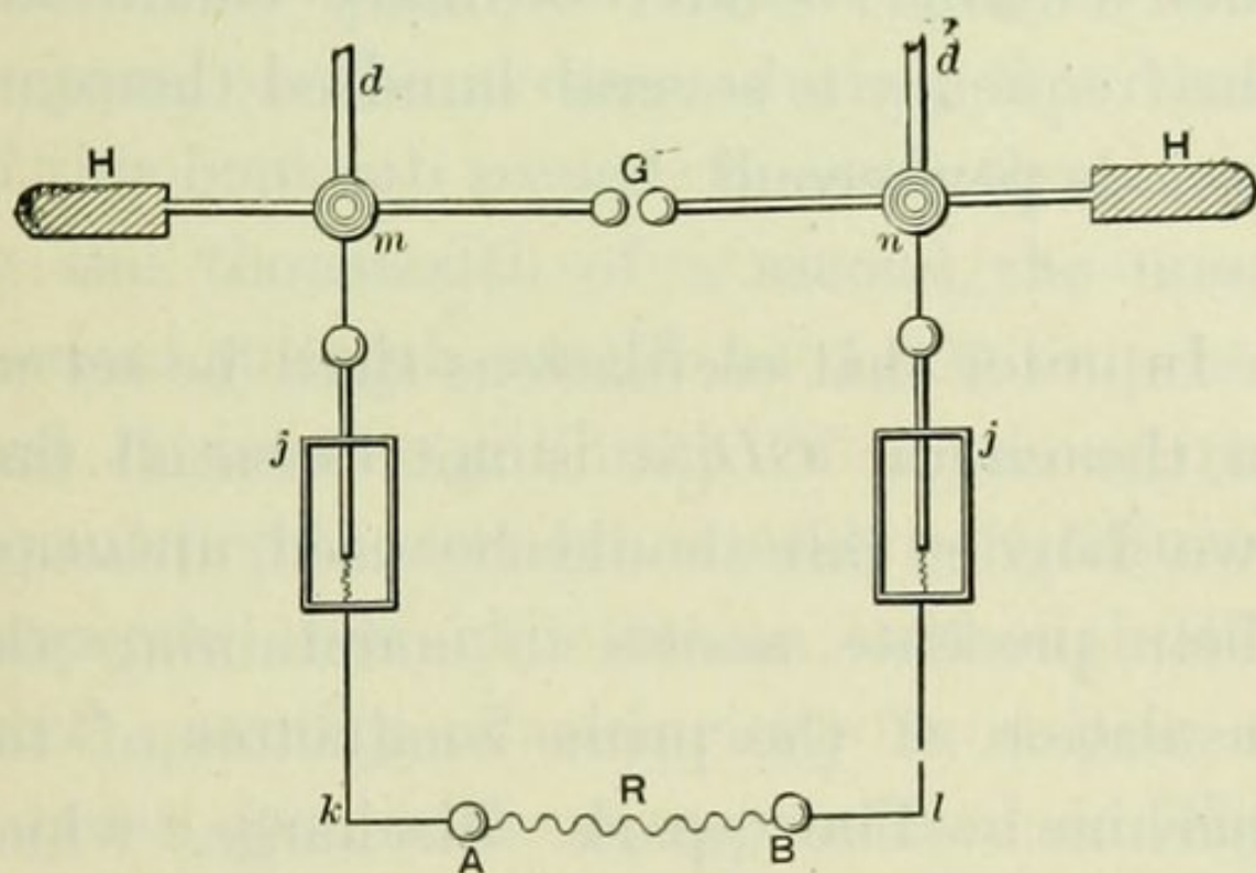
FIG. 126.—OSCILLATORY CURRENT CIRCUIT OF INFLUENCE MACHINE.
