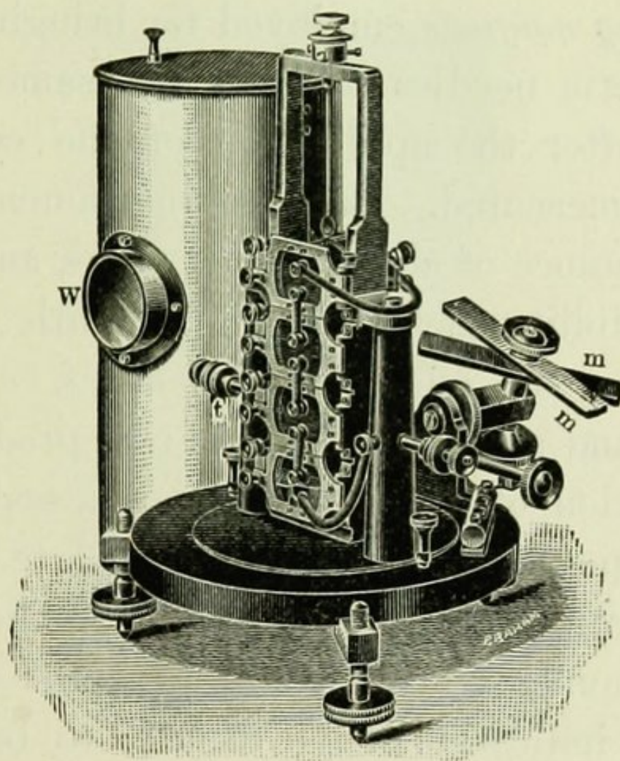
FIG. 37.—SENSITIVE MIRROR GALVANOMETER.
