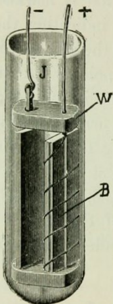
FIG. 8.—FORM OF SILVER-CHLORIDE CELL.
