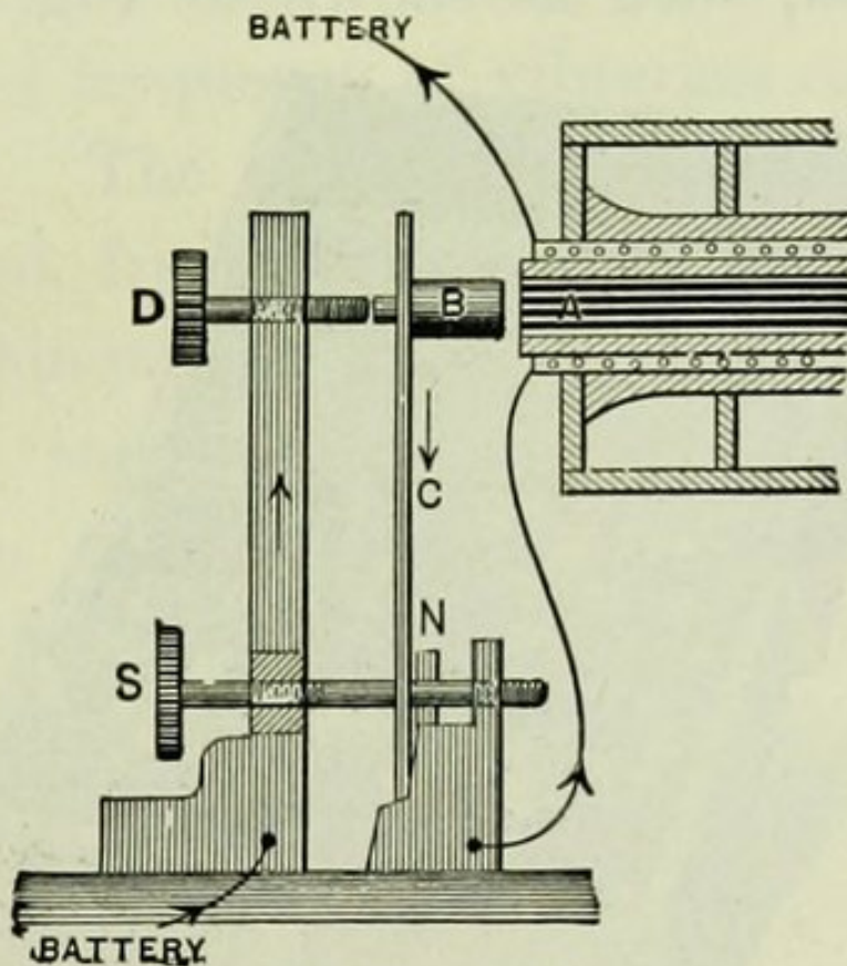
FIG 100.—ADJUSTABLE VIBRATOR FOR FARADIC COILS.
