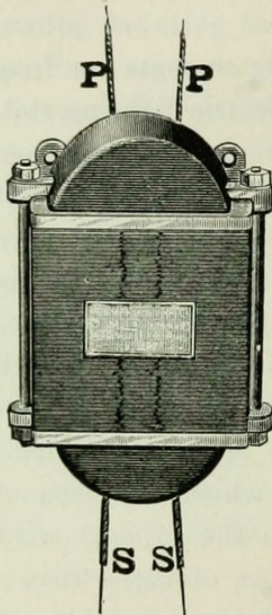
FIG. 112.—ALTERNATING CURRENT TRANSFORMER.
