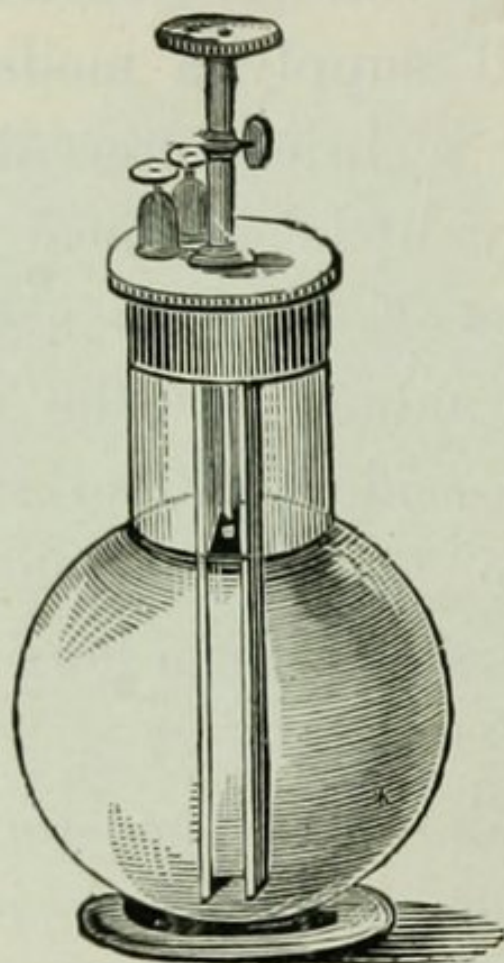
FIG. 12.—GRENET PLUNGE CELL.
