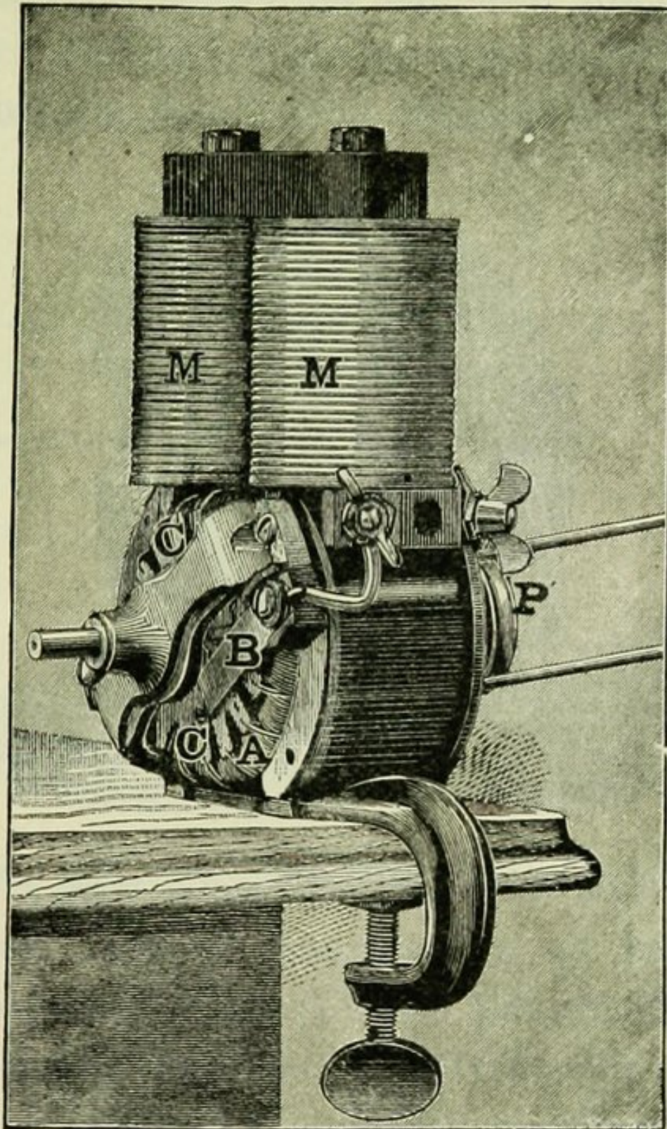
FIG. 109.—ELECTROMAGNETIC MOTOR.
