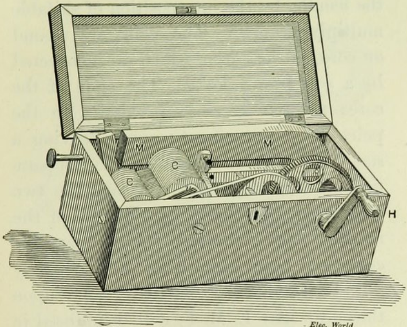
FIG. 88.—MAGNETO-ELECTRIC GENERATOR.
