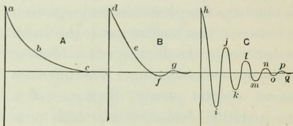
FIG. 123.—OSCILLATORY DISCHARGE.
