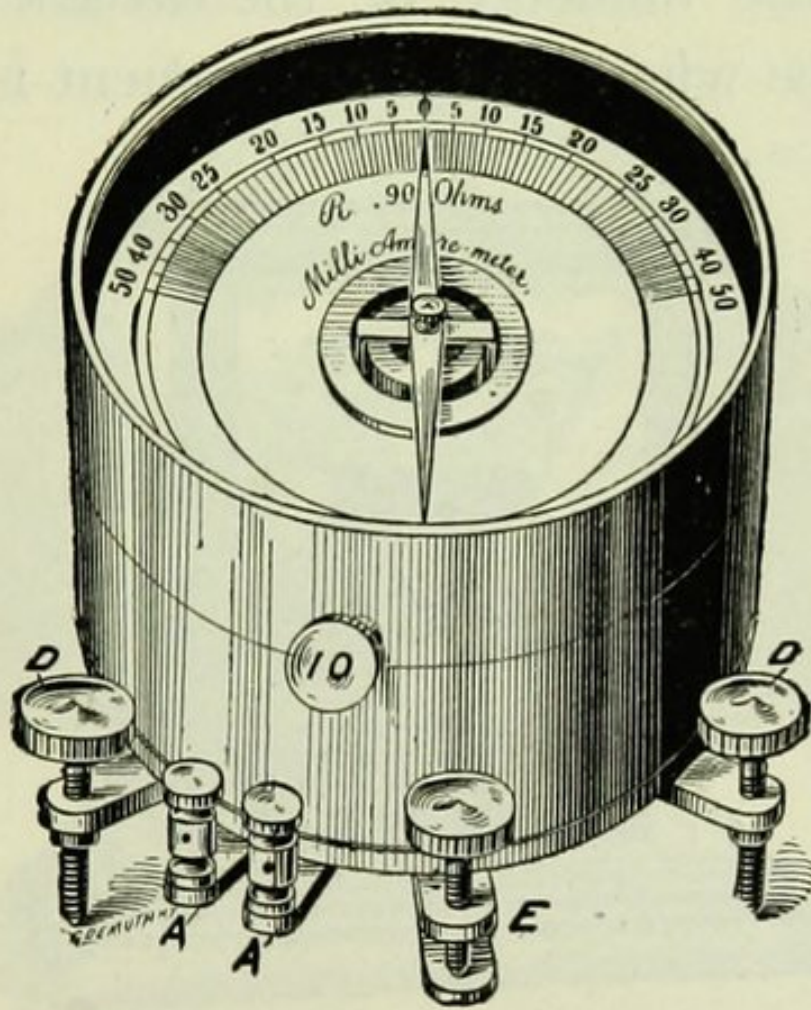
FIG. 30.—FORM OF MILLIAMMETER.
