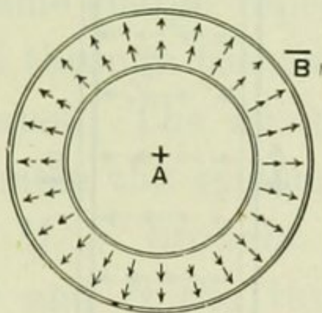
FIG. 57.—ELECTROSTATIC FLUX PATHS BETWEEN INSULATED CONCENTRIC SPHERES.
