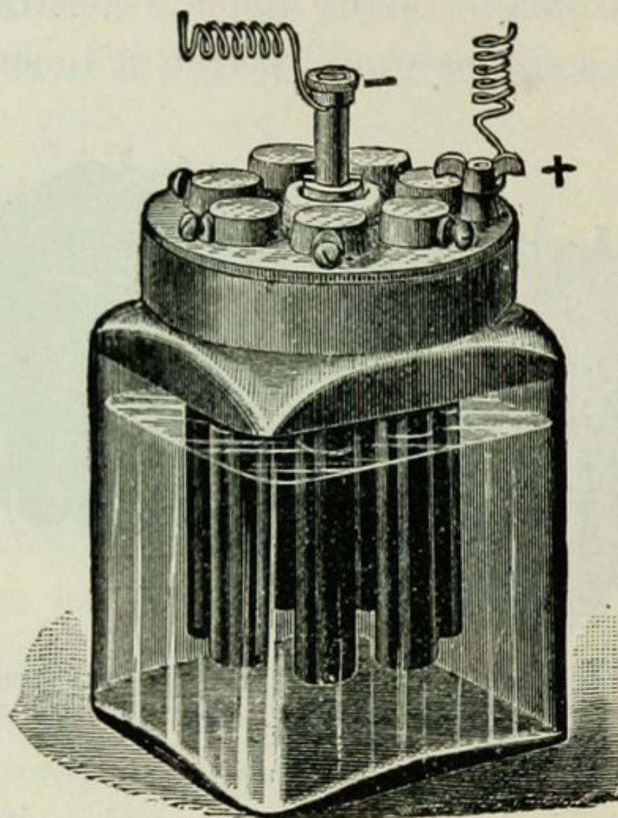
FIG. 11.—ZINC-CARBON CELL.
