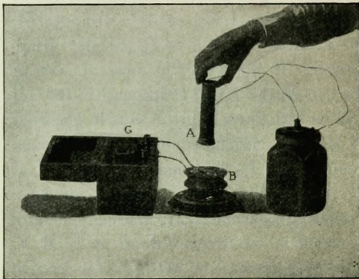
FIG. 85.—MUTUAL INDUCTION.
