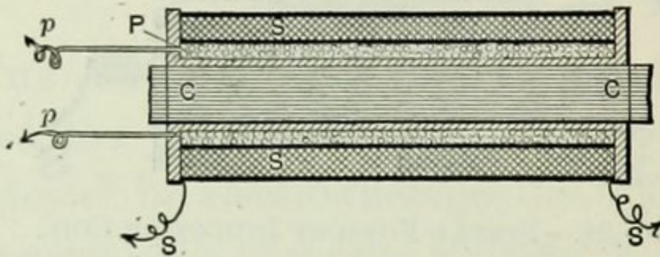
FIG. 95.—SECTION OF SIMPLE FORM OF INDUCTION COIL.
