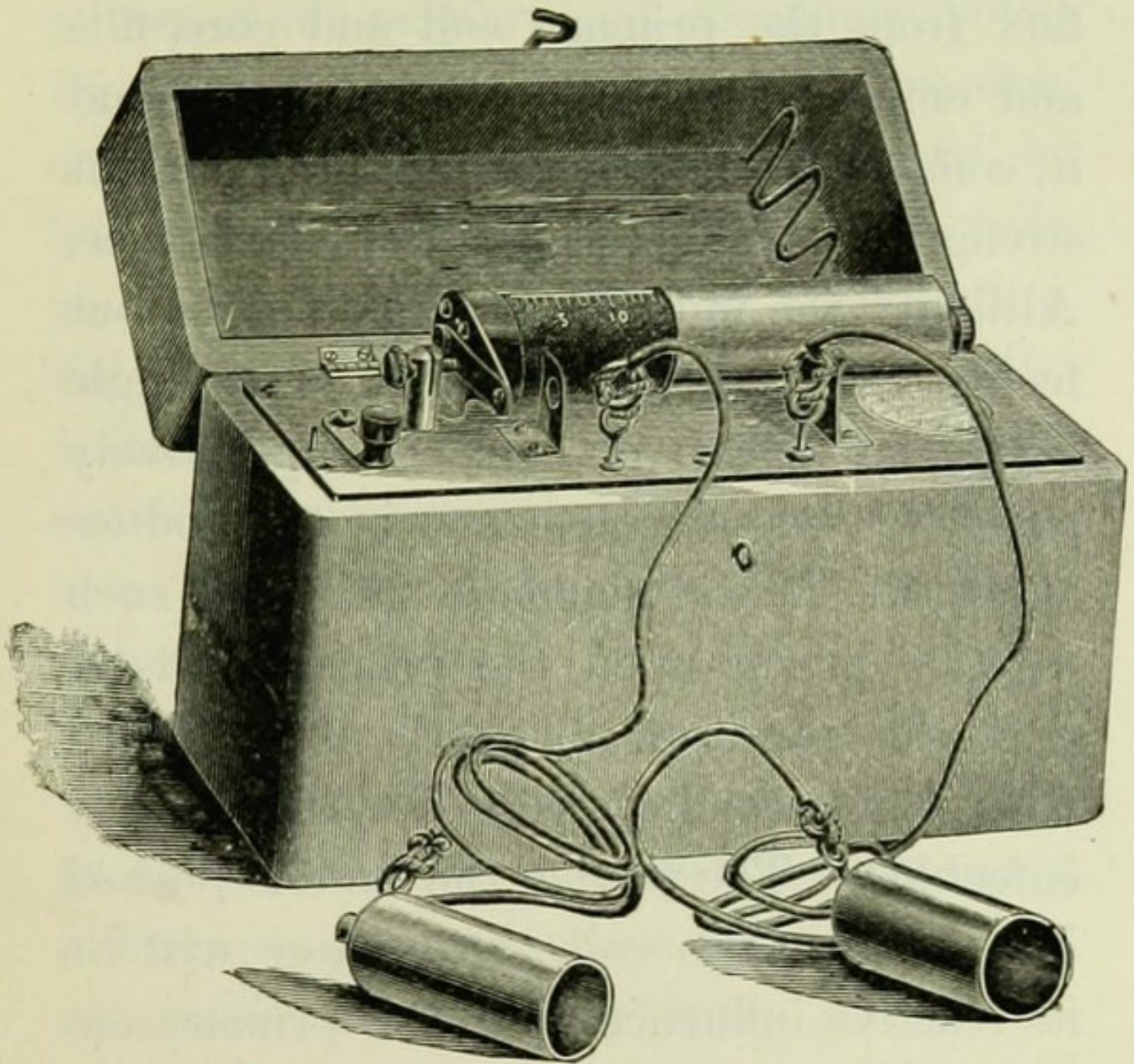
FIG. 104.—INDUCTION COIL WITH EXTERNAL DAMPING TUBE.
