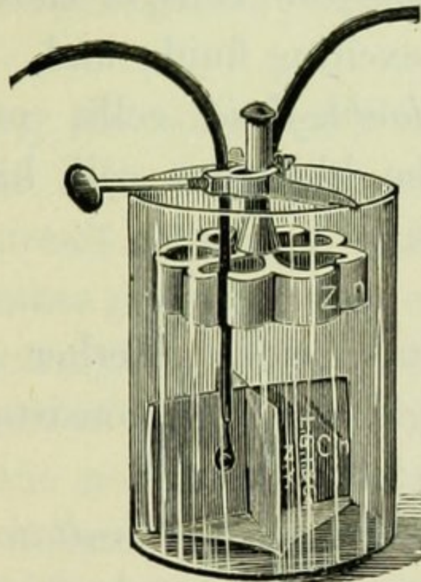
FIG. 7.—BLUESTONE OR GRAVITY VOLTAIC CELL.
