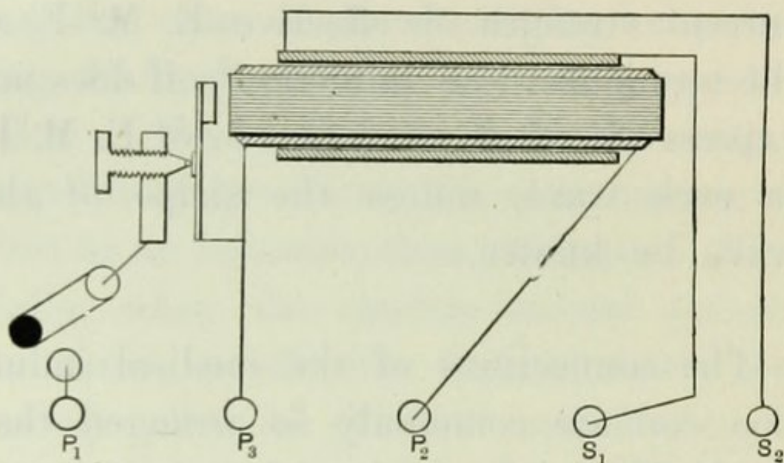
FIG. 105.—CONNECTIONS OF MEDICAL INDUCTION COIL.
