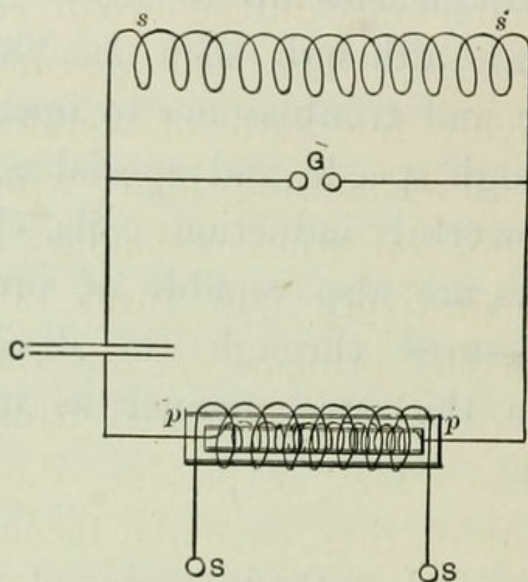
FIG. 127.—APPARATUS FOR HIGH FREQUENCY ALTERNATING CURRENTS.
