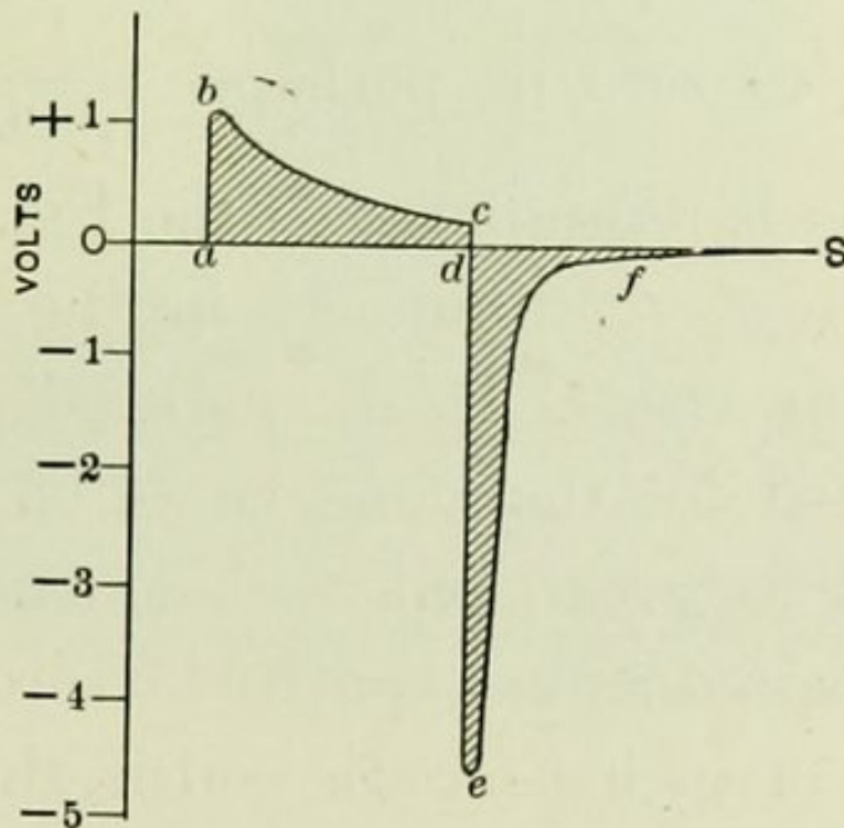
FIG. 97.—DIAGRAM OF PRIMARY INDUCED E. M. FS.
