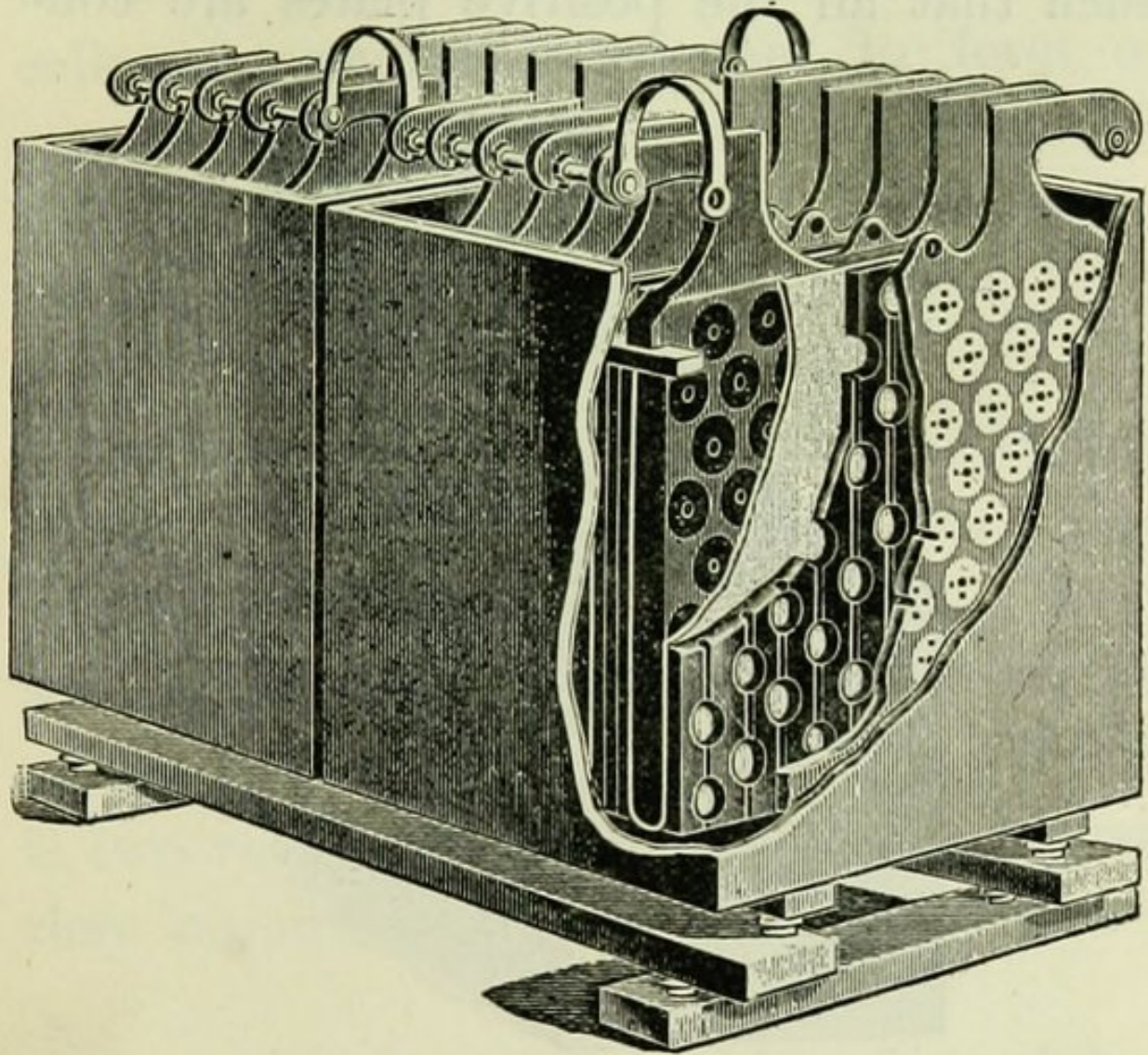
FIG. 22.—INTERIOR VIEW OF CHLORIDE STORAGE BATTERY.
