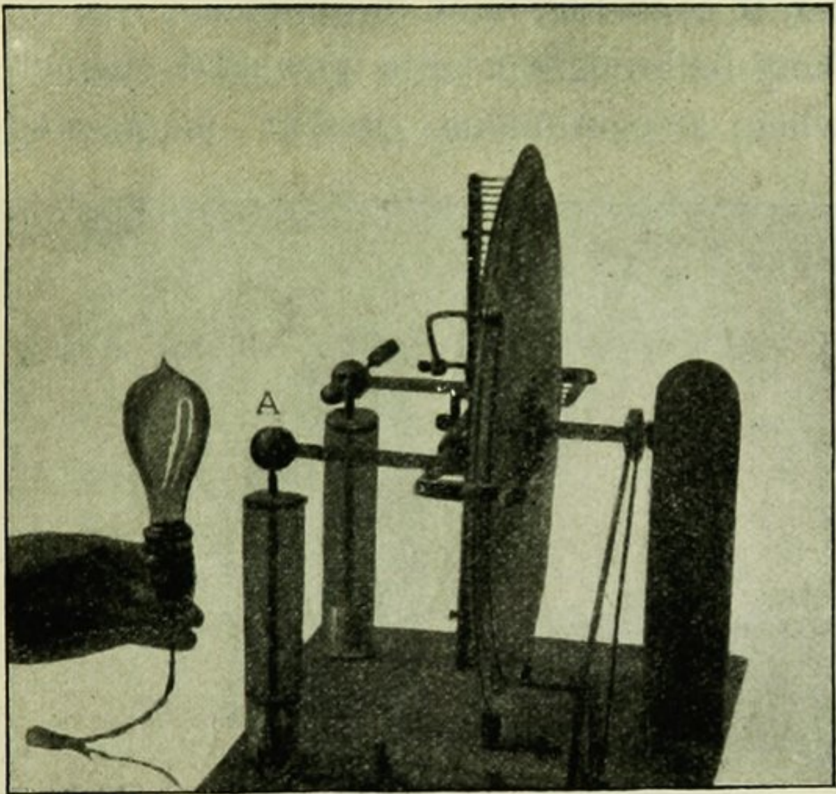
FIG. 4.—TRANSMISSION OF ELECTROSTATIC FORCE ACROSS A VACUUM.
