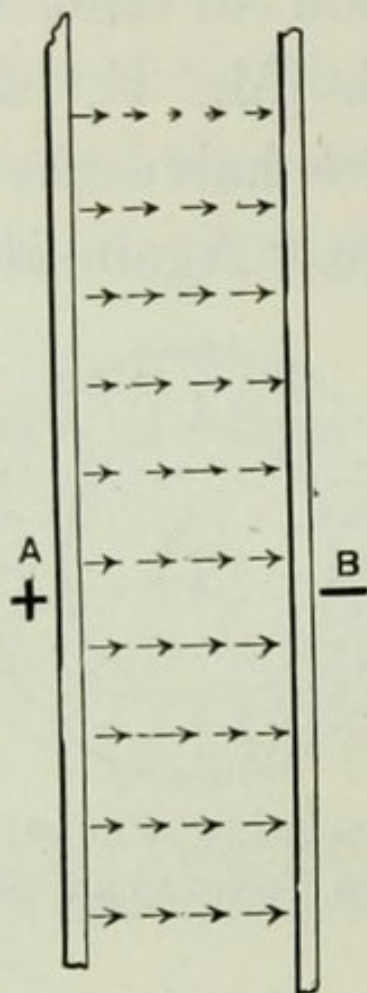
FIG. 58.—ELECTROSTATIC FLUX PATHS, PARALLEL PLANE SPHERES.
