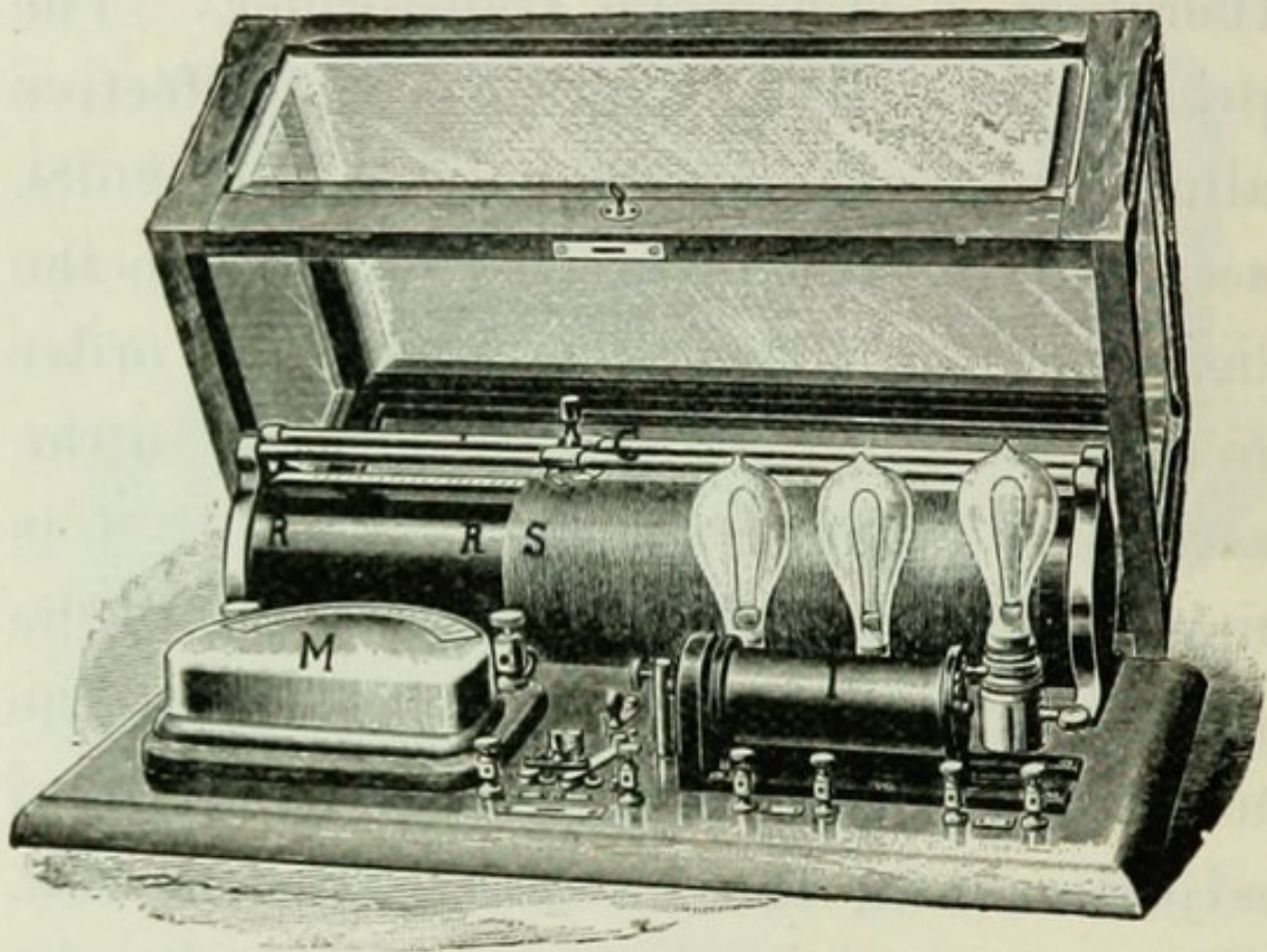
FIG. 114.—ADAPTER FOR CONTINUOUS CURRENT CIRCUITS.
