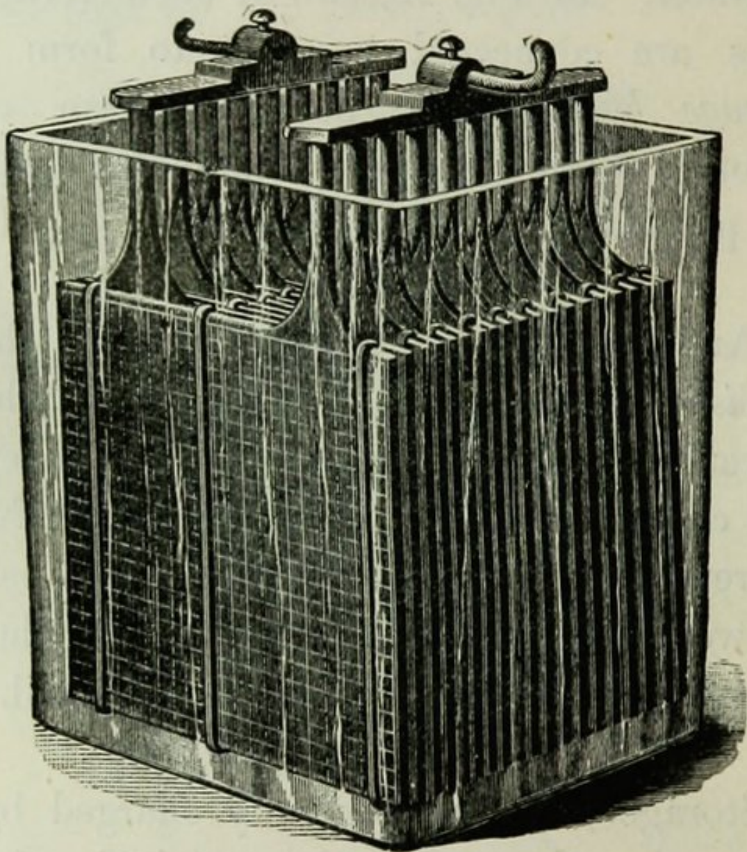
FIG. 24.—JULIEN STORAGE CELL.
