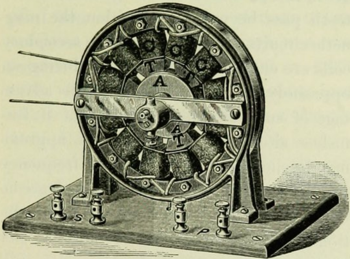
FIG. 111.—ELECTRO-THERAPEUTIC ALTERNATOR.
