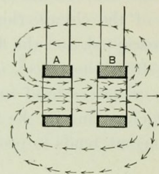
FIG. 84.—DIAGRAM ILLUSTRATING MUTUAL INDUCTION.
