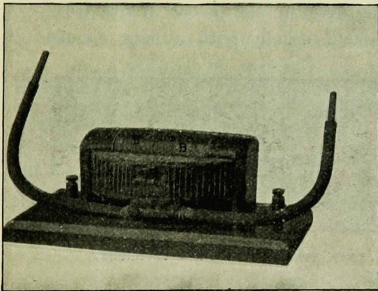
FIG. 78.—ALTERNATING-CURRENT TRANSFORMER, FERRIC MAGNETIC CIRCUIT.
