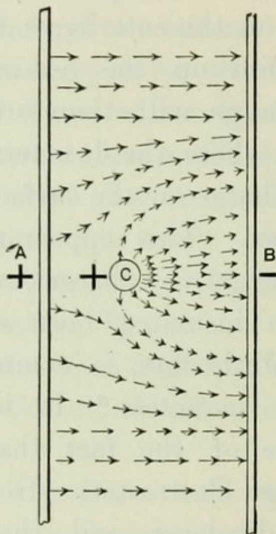
FIG. 59.—DIAGRAMMATIC REPRESENTATION OF ELECTROSTATIC FLUX PATHS.
