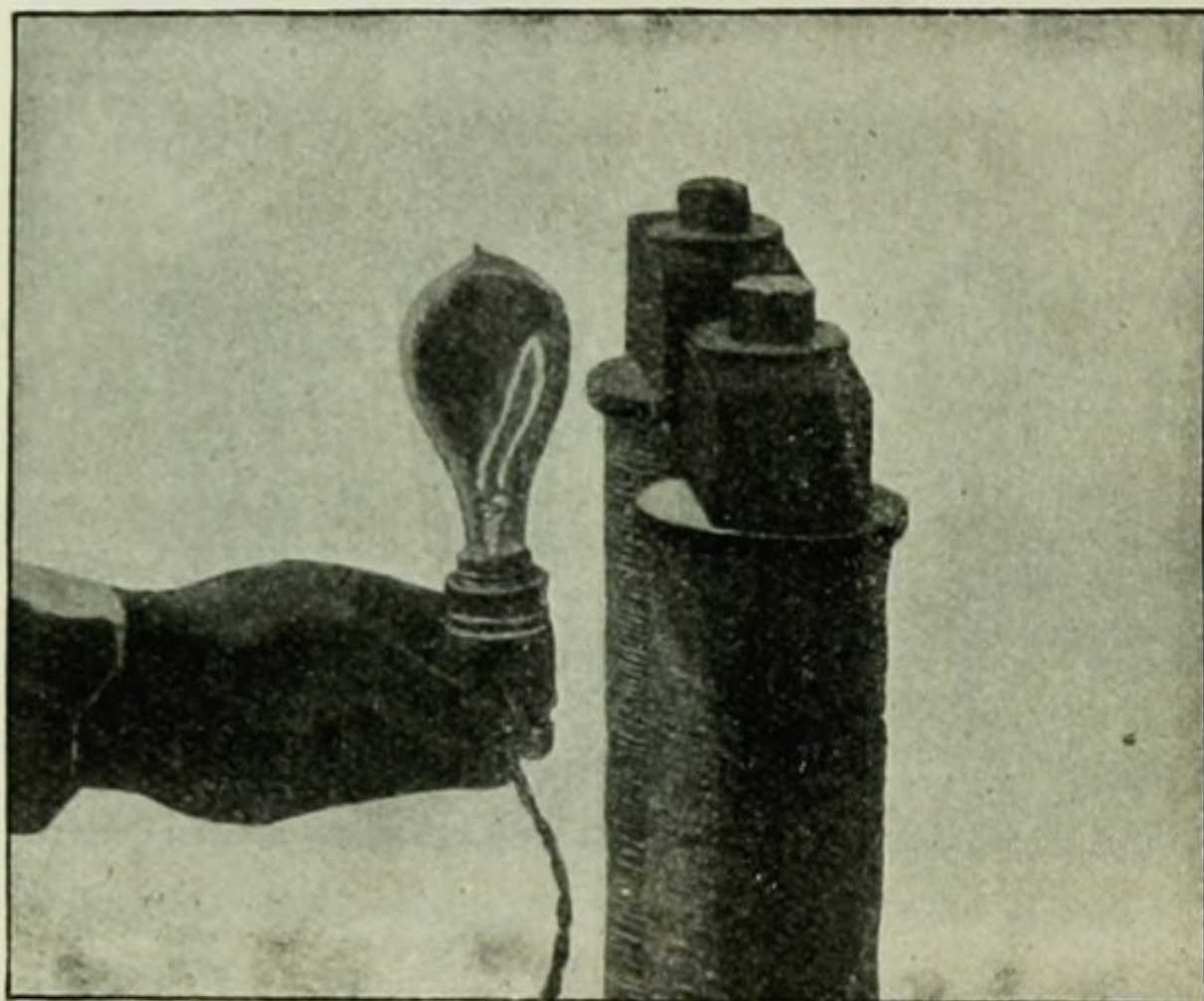
FIG. 5.—TRANSMISSION OF MAGNETIC FORCE ACROSS A VACUUM.
