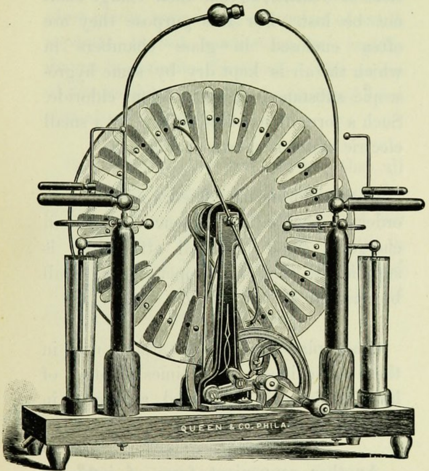
FIG. 73.—WIMSHURST ELECTRICAL MACHINE.
