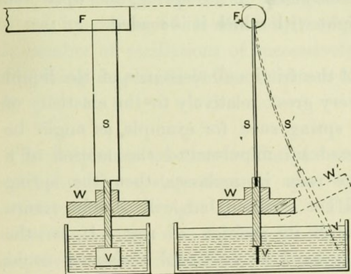
FIG. 124.—MECHANICAL VIBRATOR, SIDE AND END VIEW.
