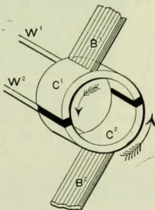
FIG. 91.—DIAGRAM OF TWO-PART COMMUTATOR.
