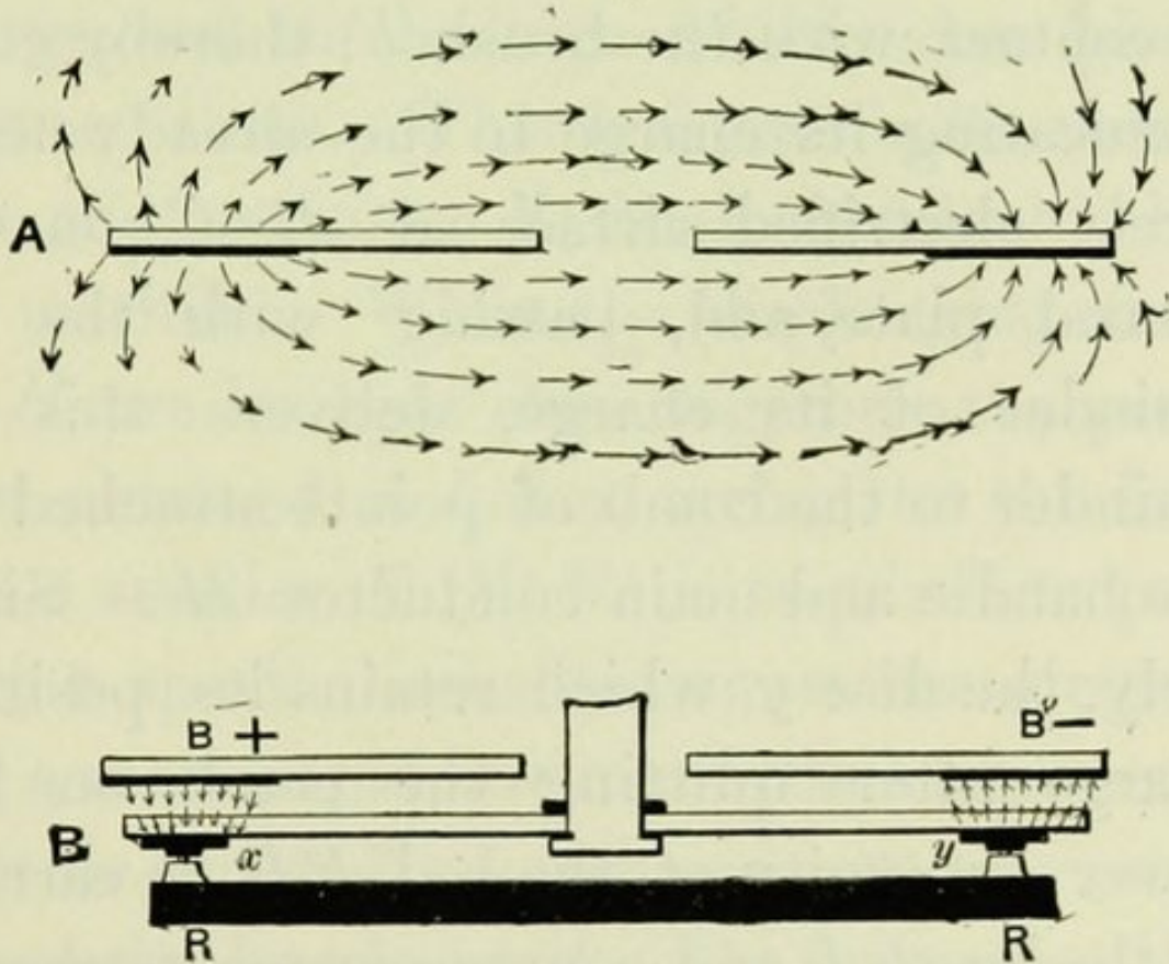
FIG. 69.—ELECTROSTATIC CIRCUITS OF INFLUENCE MACHINE.
