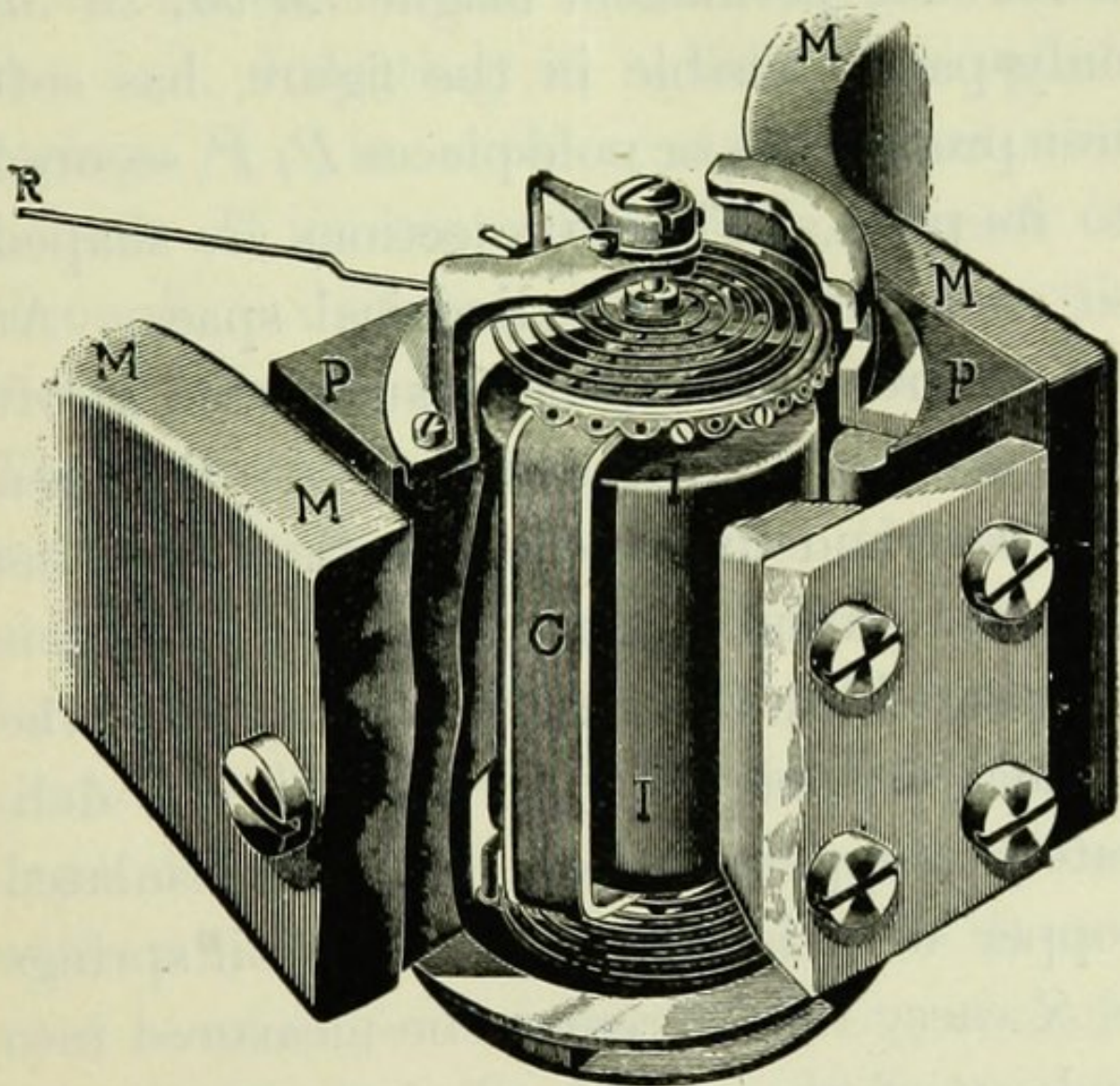
FIG. 34.—WORKING PARTS OF WESTON AMMETER.
