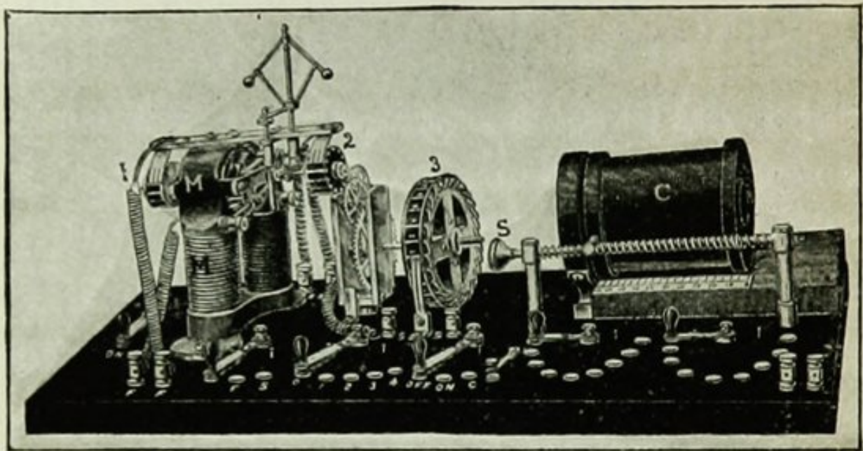
FIG. 102.—INDUCTION COIL WITH RAPID INTERRUPTER.
