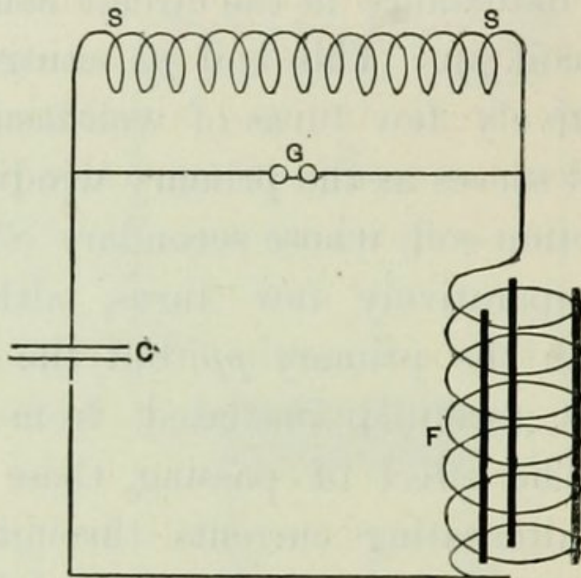
FIG. 128.—APPARATUS FOR CREATING RAPIDLY OSCILLATING MAGNETIC FIELD.
