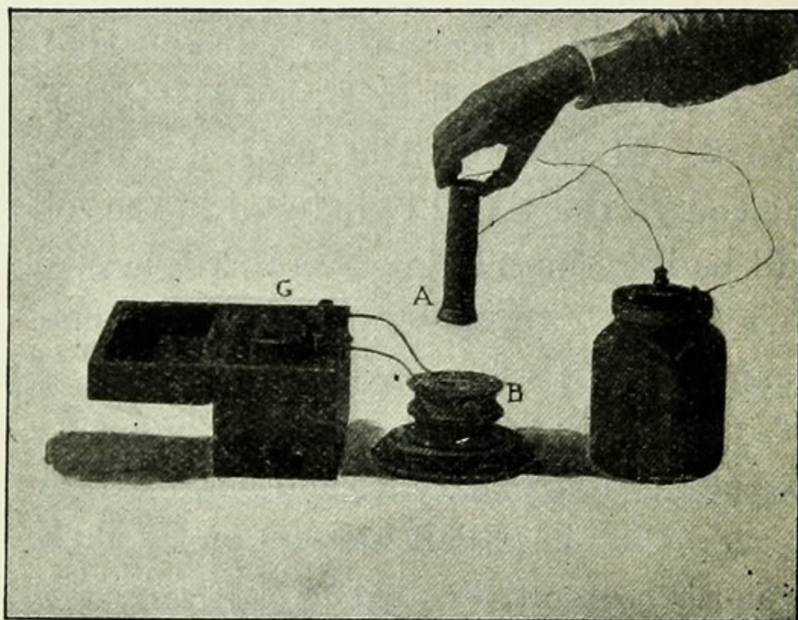
FIG. 85.—MUTUAL INDUCTION.
