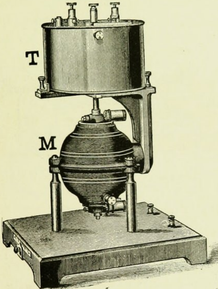
FIG. 140.—WATER INTERRUPTER.
