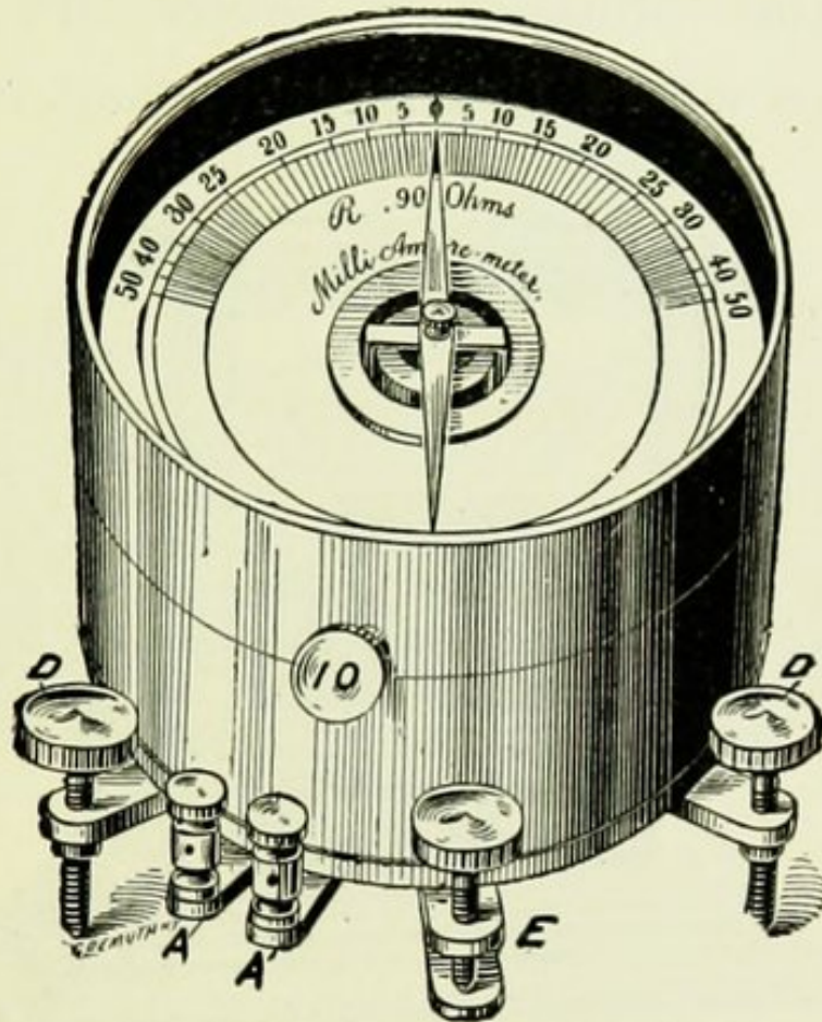
FIG. 30.—FORM OF MILLIAMMETER.
