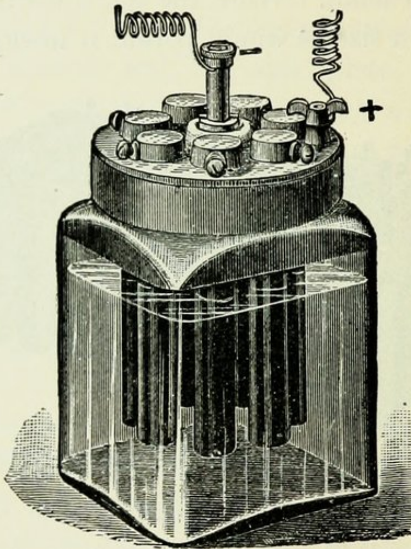
FIG. 11.—ZINC-CARBON CELL.
