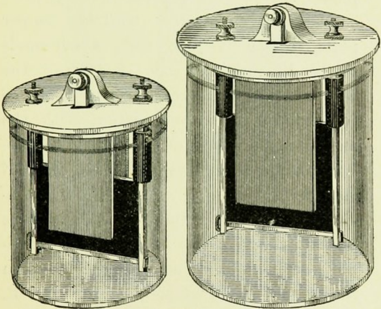
FIG. 13.—EDISON-LALANDE CELLS.
