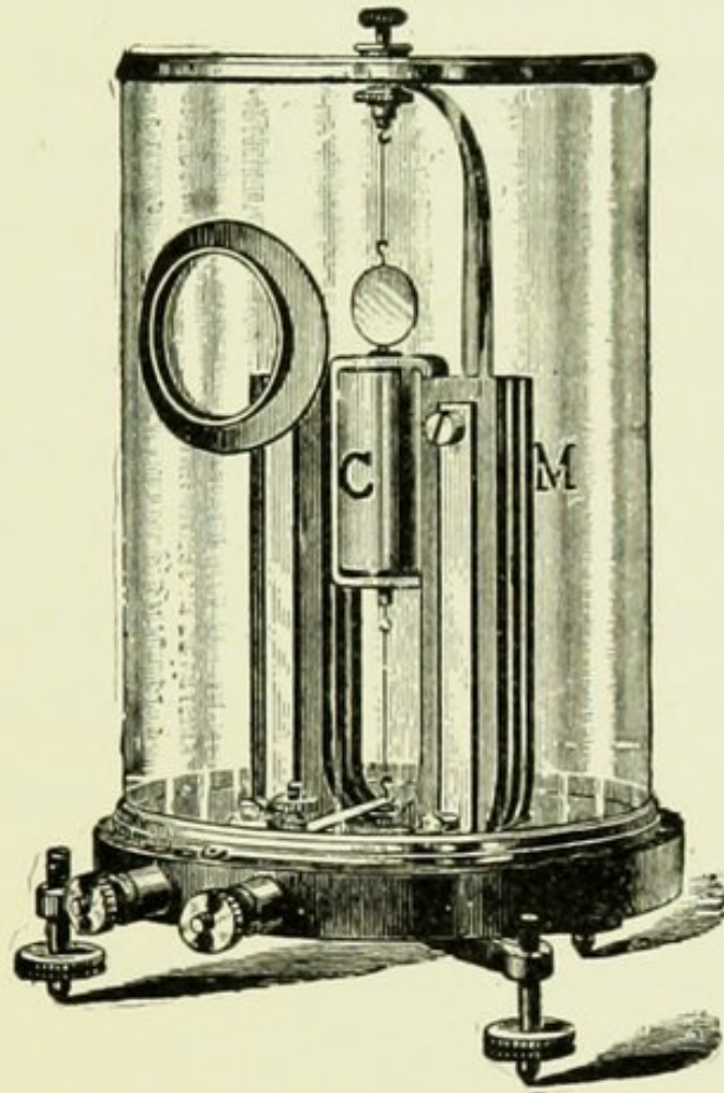
FIG. 38.—D'ARSONVAL GALVANOMETER.
