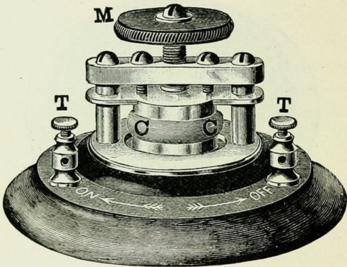
FIG. 120.—CARBON PRESSURE RHEOSTAT.
