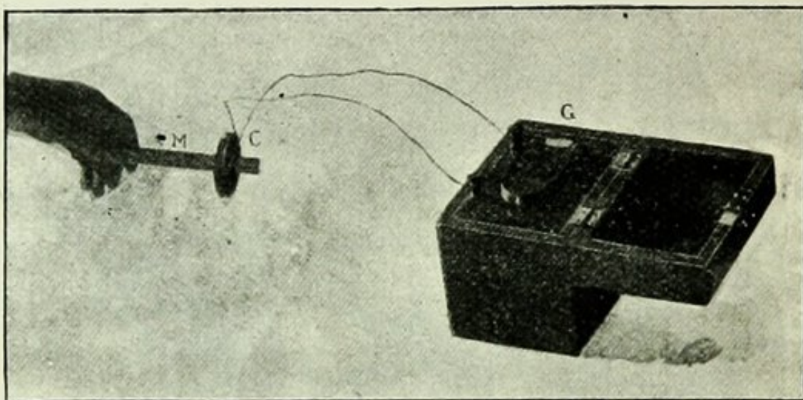
FIG. 87.—MAGNETO-ELECTRIC INDUCTION.
