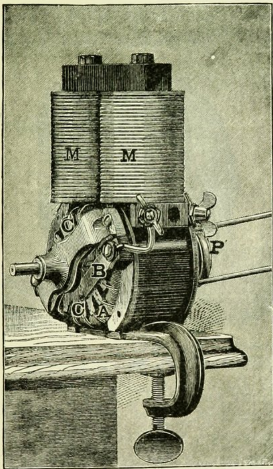
FIG. 109.—ELECTROMAGNETIC MOTOR.
