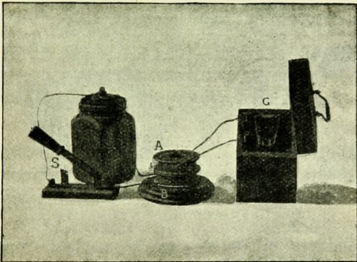
FIG. 86.—MUTUAL INDUCTION.
