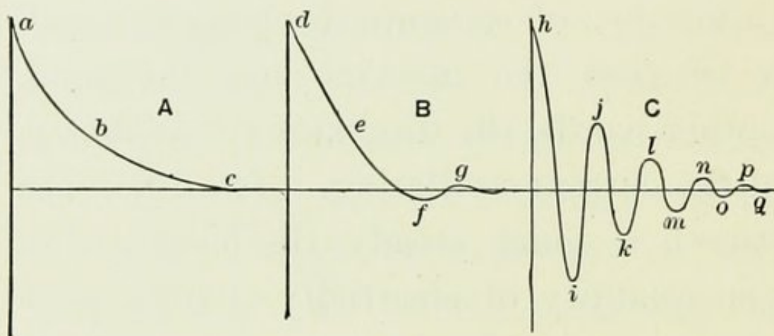
FIG. 123.—OSCILLATORY DISCHARGE.
