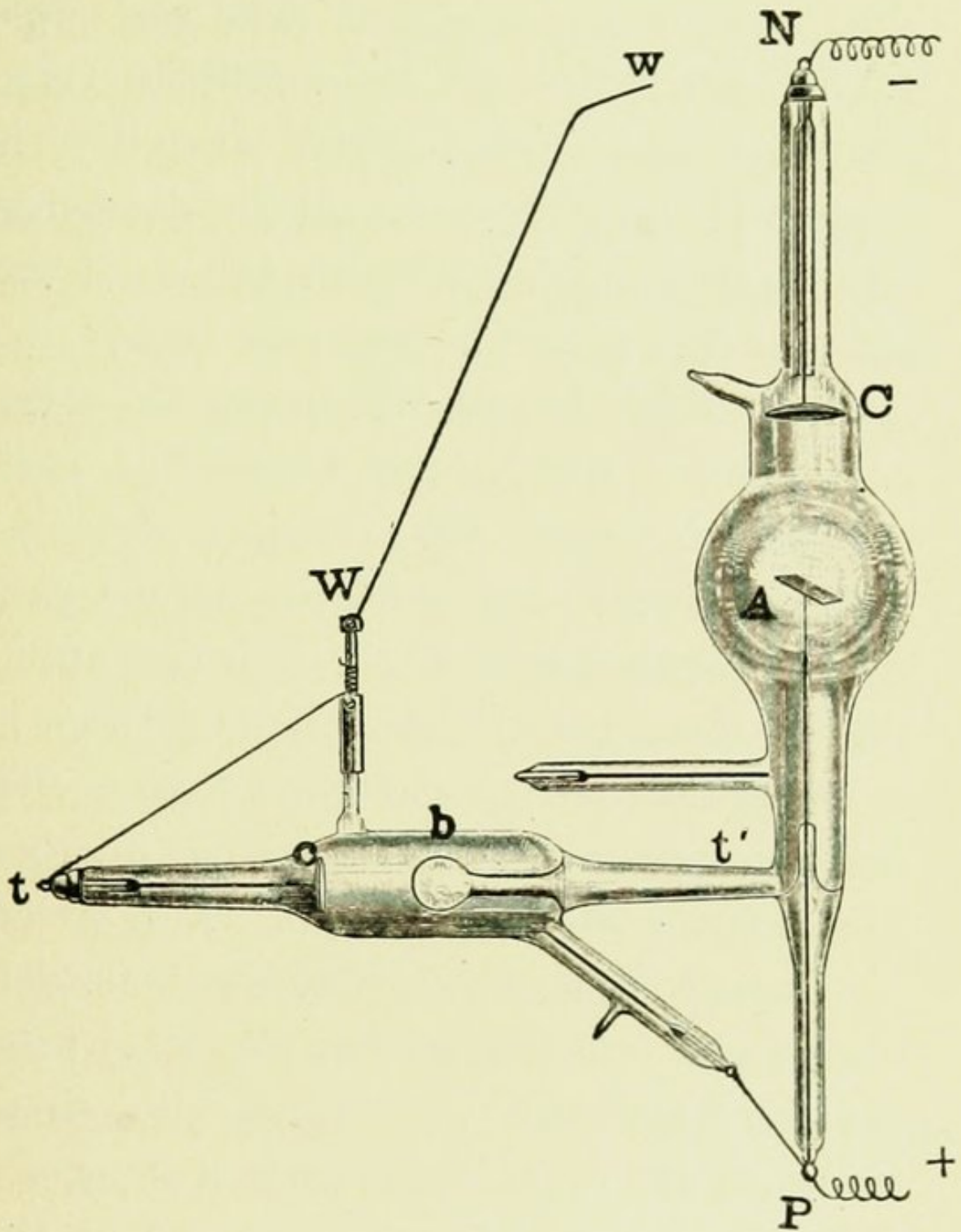
FIG. 147.—SELF-REGULATING X-RAY TUBE.
