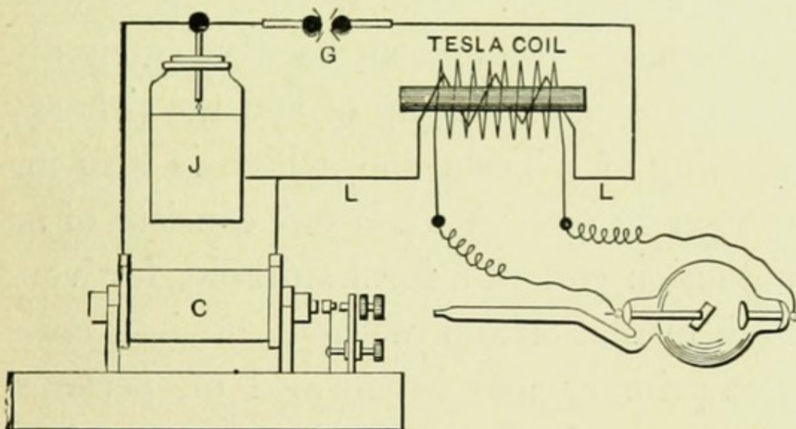
FIG. 145.—CONNECTIONS OF TESLA COIL.
