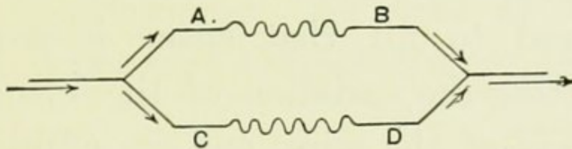
FIG. 27.—CONNECTION OF RESISTANCES IN PARALLEL.
