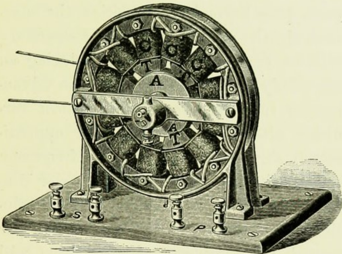
FIG. 111.—ELECTRO-THERAPEUTIC ALTERNATOR.
