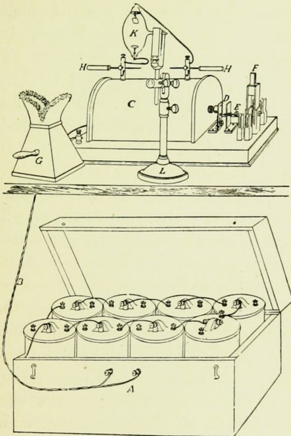
FIG. 136.—PRIMARY BATTERY AND INDUCTION COIL X-RAY OUTFIT.
