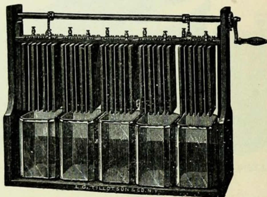
FIG. 19.—PLUNGE BATTERY.
