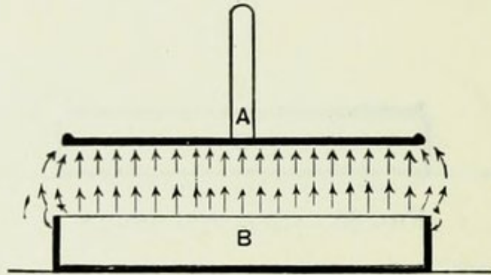
FIG. 66.—ELECTROPHORUS.
