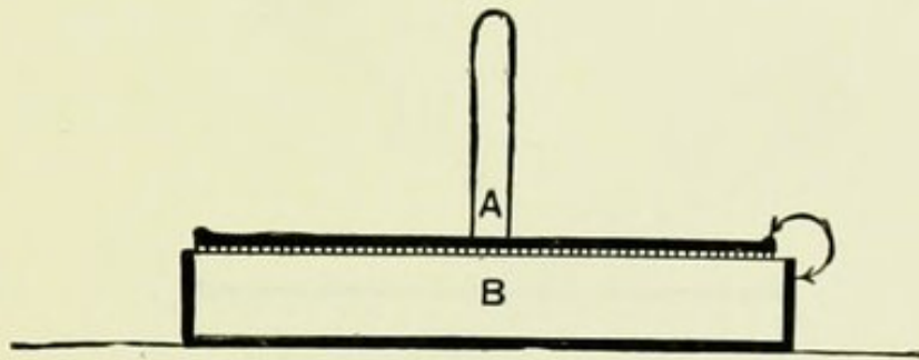
FIG. 65.—ELECTROPHORUS.
