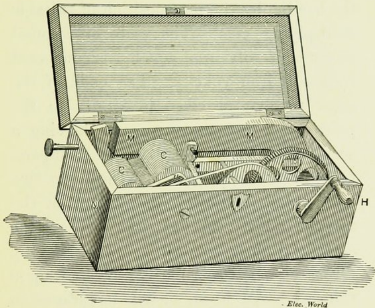
FIG. 88.—MAGNETO-ELECTRIC GENERATOR.
