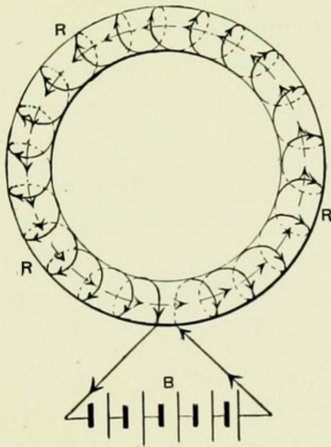
FIG. 77.—FERRIC MAGNETIC CIRCUIT.
