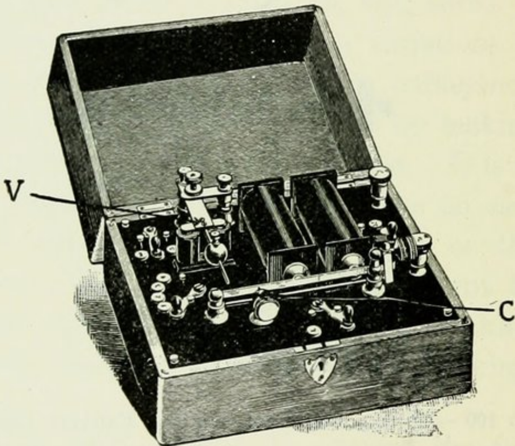
FIG. 101.—INDUCTION COIL WITH RIBBON VIBRATOR.
