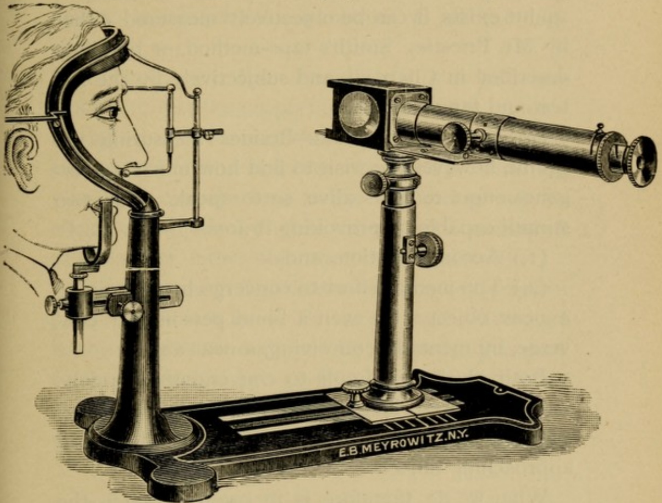
Fig. 73. —Stevens' Tropometer.
