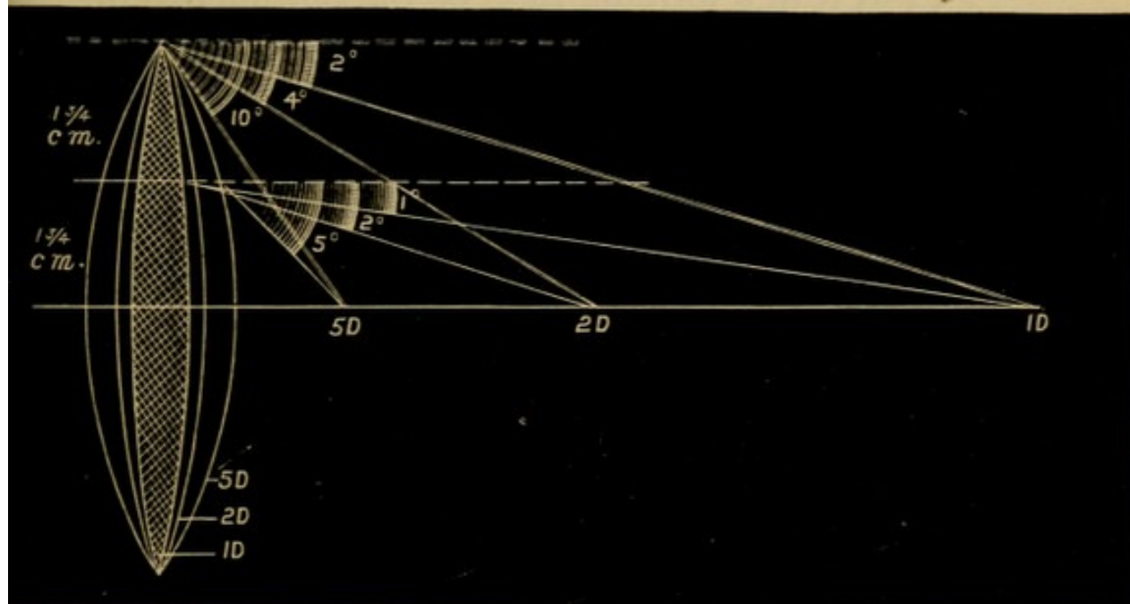
Fig. 99. —To show the Prismatic Effect of decentering ; each displacement of 1\frac{3}{4} cm. producing 1^\circ deviation for each dioptré in the lens. A metre-lens will have its principal focus at 1 D, so that light falling on the lens 1\frac{3}{4} cm. from its optical centre is deflected 1^\circ , another 1\frac{3}{4} cm. 2^\circ , and so on. A half-metre lens will have its focus at 2 D, and the corresponding deflections will be 2^\circ and 4^\circ . With a 5 D lens they will be 5^\circ and 10^\circ .
