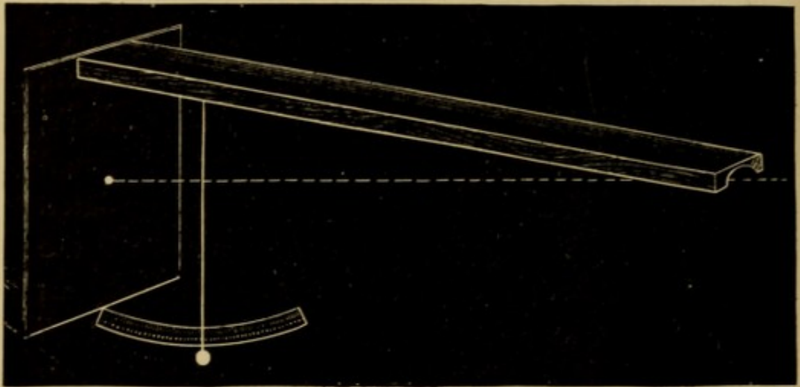
Fig. 106. —Eaton's mode of making Meissner's Test.
