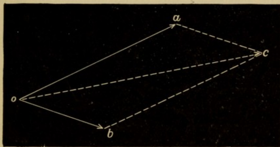
Fig. 28.—Composition of Rotations.
