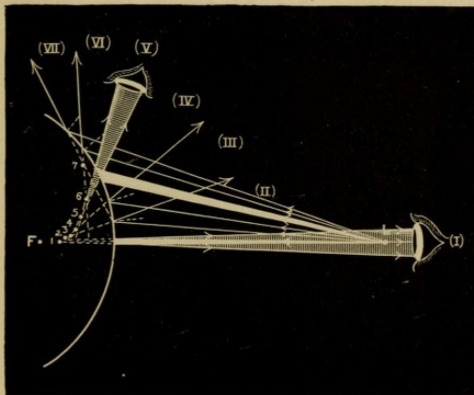
Fig. 84. —The Caustic Curve of a convex mirror whose principal focus is at F.
