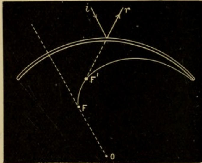
Fig. 48. —Section of Cornea, to show that light reflected from the centre of the cornea symmetrically does not produce an image in the optic axis, but rather to one side of the centre of the pupil.
