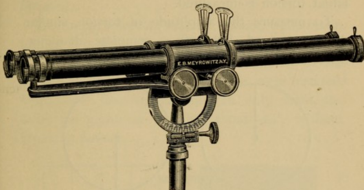
Fig. 102. —Stevens' Clinoscope.
