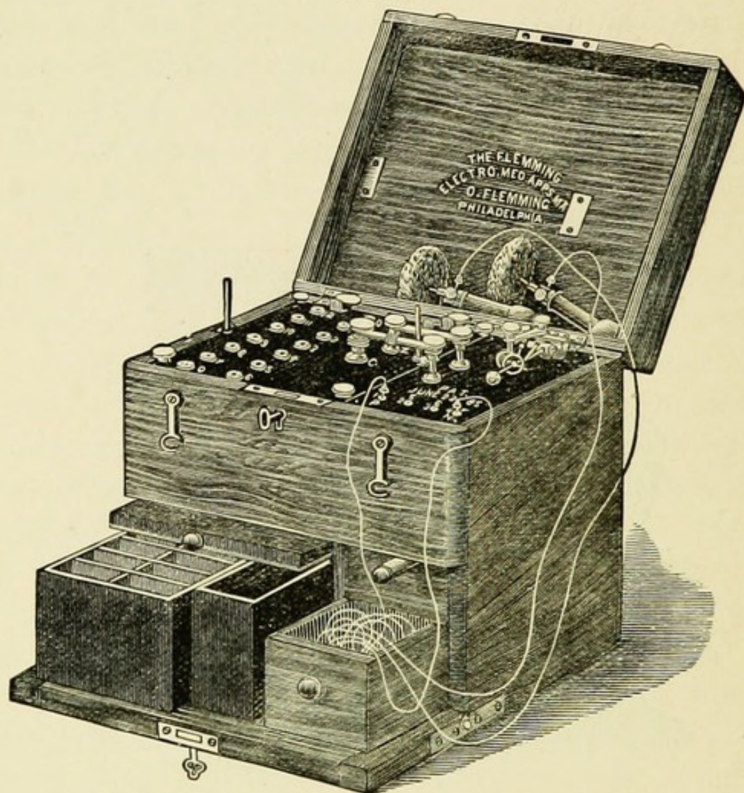
FLEMING'S 30-CELL COMBINATION BATTERY.
