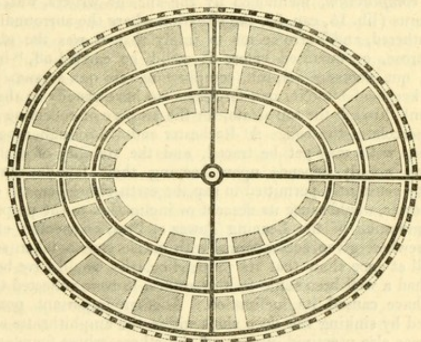
Plan of the Amphitheatre at Verona.
