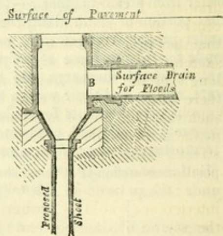
Section in a line with Street.
