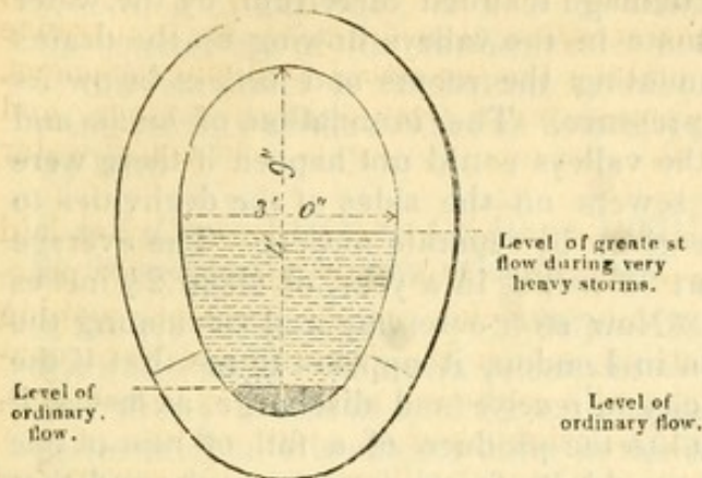
Main Sewer of the egg shape. Fig. 3.
