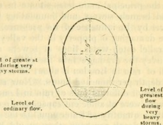
Collateral Sewer of the egg shape. Fig. 4.
