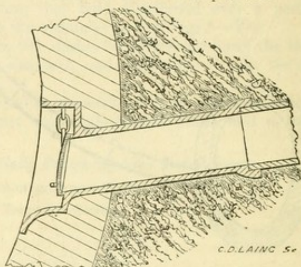
Section of Drain and Flap at Vent.
