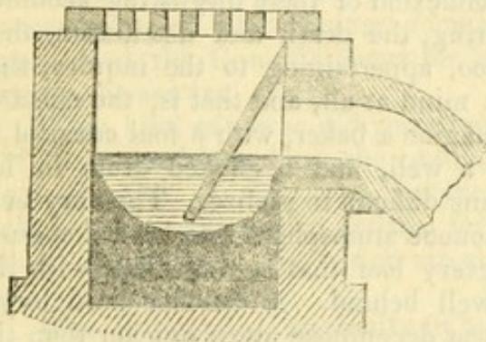
Section of an ordinary Trap to Gully Shoots, showing deposit of filth.
