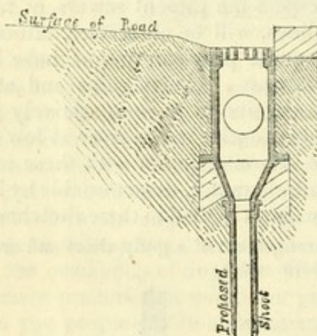
Section across Street.
