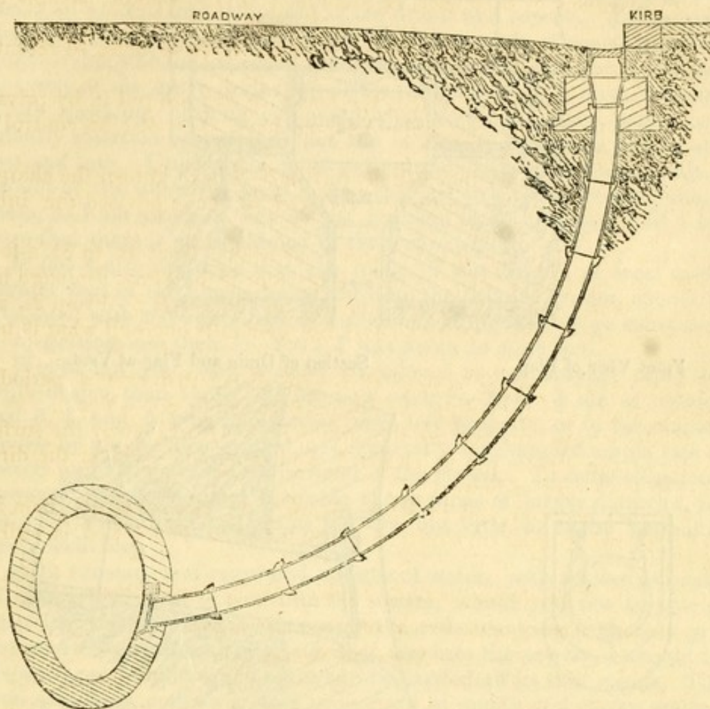
Section of Gully Drain from Grating to Sewer.
