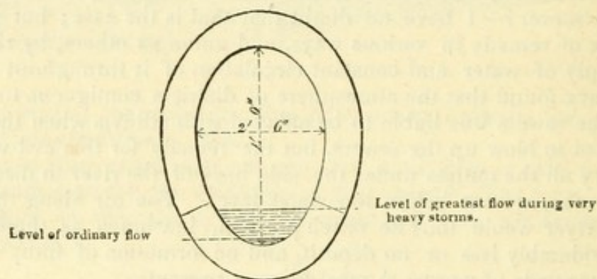
Collateral Sewer of the egg shape.
