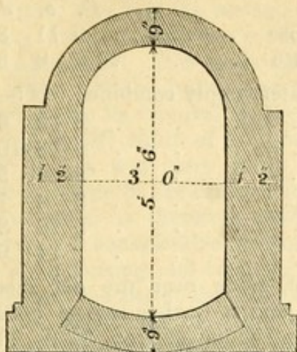
Past Form, Second Size.
