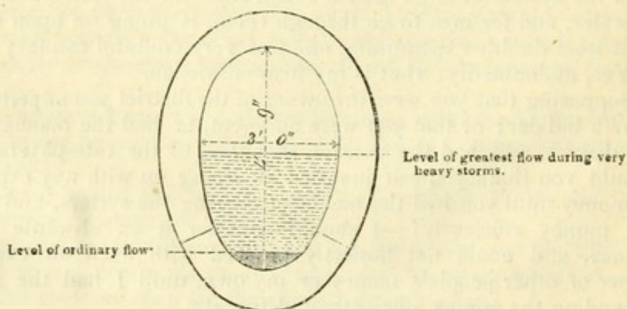
Main Sewer of the egg shape.
