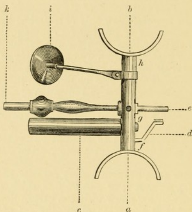
FIG. 67.—THE UNIVERSAL ACOUMETER DESIGNED BY THE AUTHOR.
