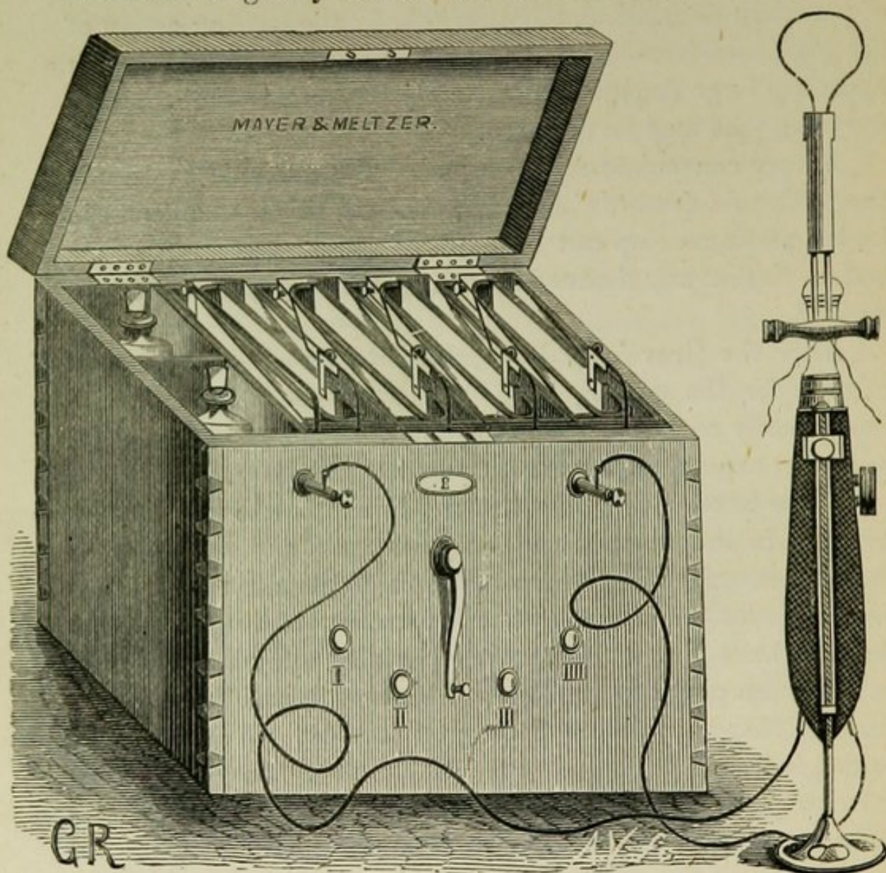
FIG. 26.—Large-celled Bunsen's battery for the galvanic cautery.
