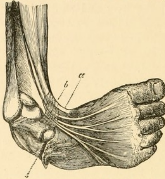
Fig. 49.—Dissection of equino-varus club-foot, dorsal view (Adams).
