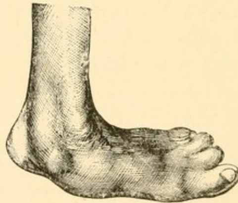
Fig. 35. —Flat-foot (after Adams).
