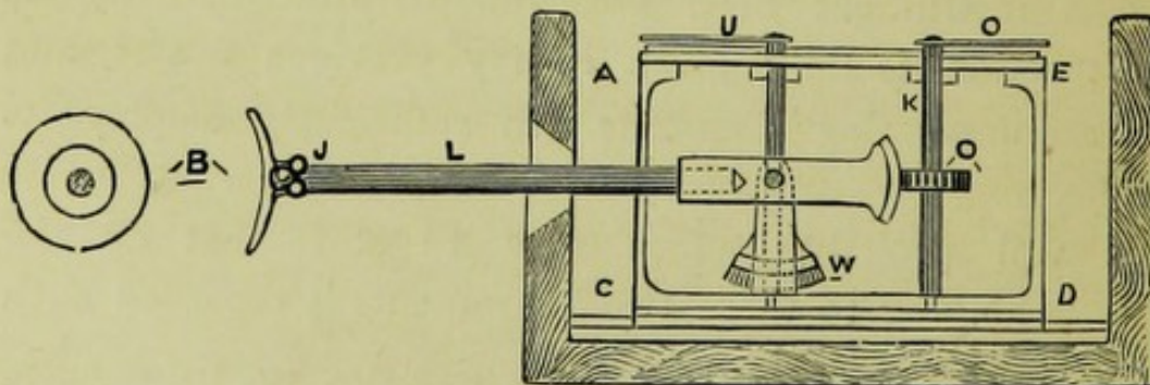
FIG. 4.—Sectional side elevation.
