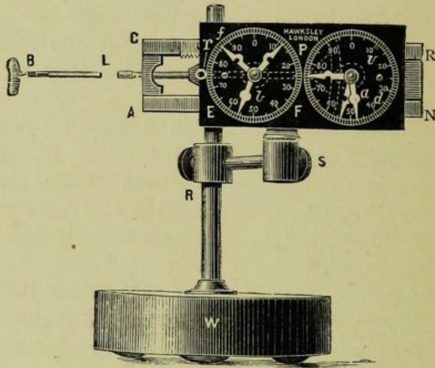
FIG. I.—Two-Plane Stethometer.
