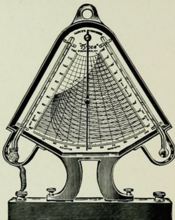
CONVENIENT HYGRODEIK FOR INSPECTION OF HUMIDITY AT REGULAR INTERVALS
