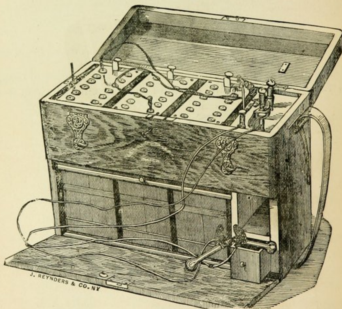
FIG. 9.—Thirty Cell Zinc-carbon Battery. (Fleming & Talbot.)
