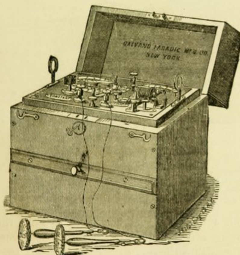
FIG. 10.—Twenty-four-cell Zinc-carbon Battery. (Galvano-Faradic Manufacturing Co.)
