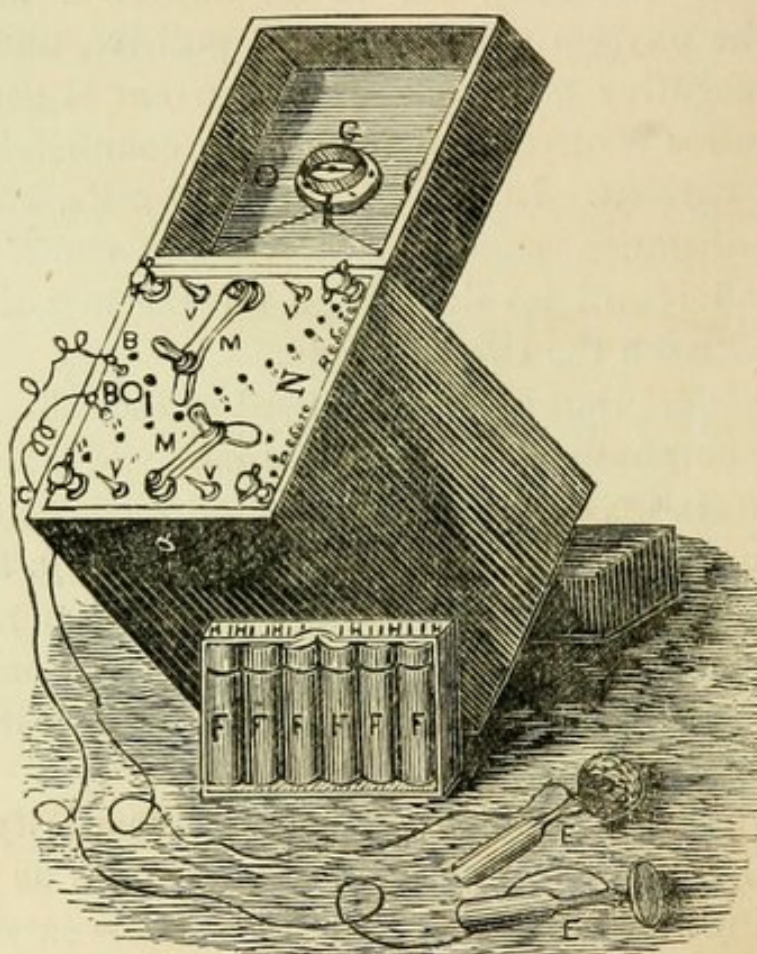
FIG. 6.—Gaiffe's Chloride of Silver Battery.
