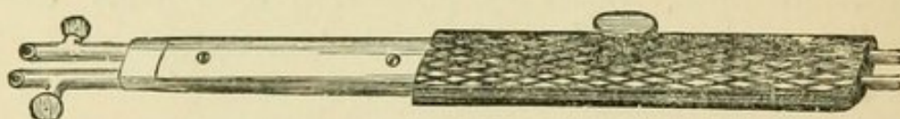
FIG. 26.—Handle for platinum knife or burner, with spring for closing and interrupting the circuit.
