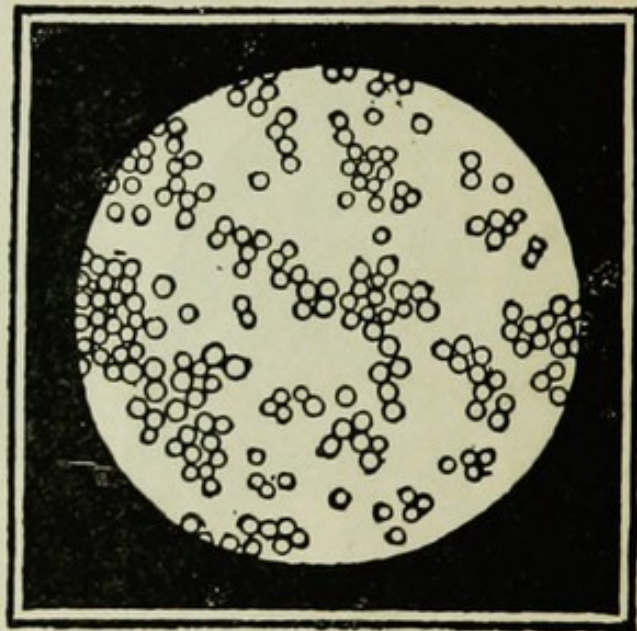
Pure Milk, showing oil globules (magnified 400 diameters).
