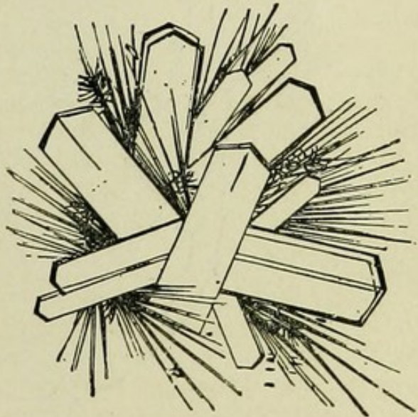
Aloin , prepared from Barbadoes Aloes ( Aloe Vulgaris ). Microscopical appearance.
