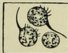
Trichomonas vaginæ, showing the large heads, with granules and cilia.
