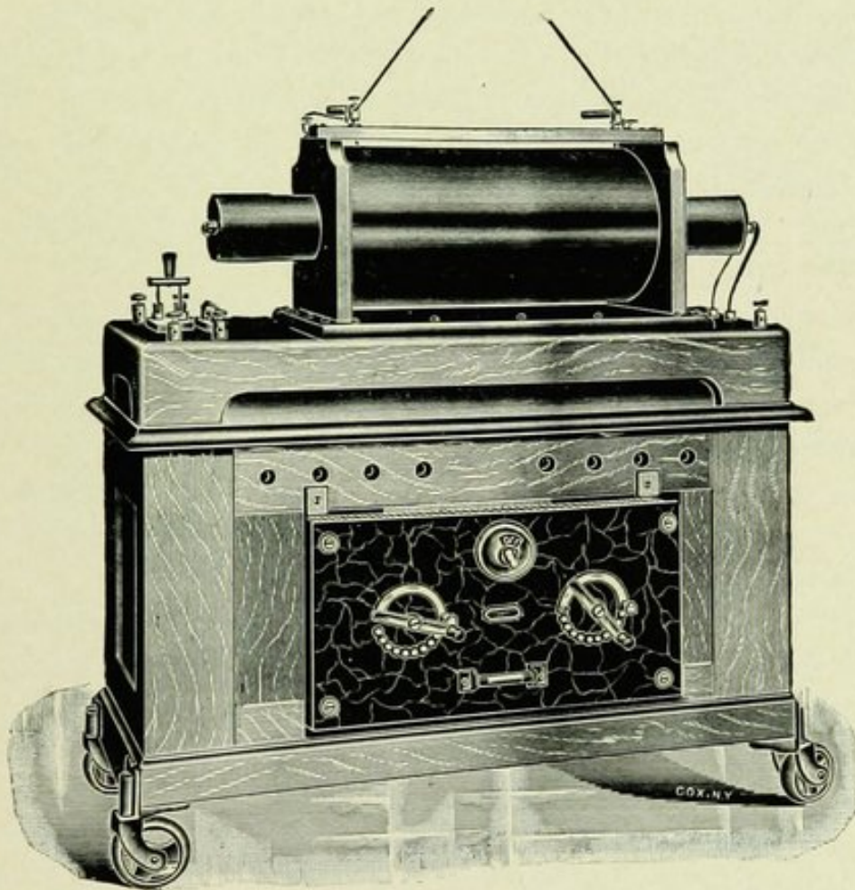
Fig. 4.—Type of X-Ray Coil.
