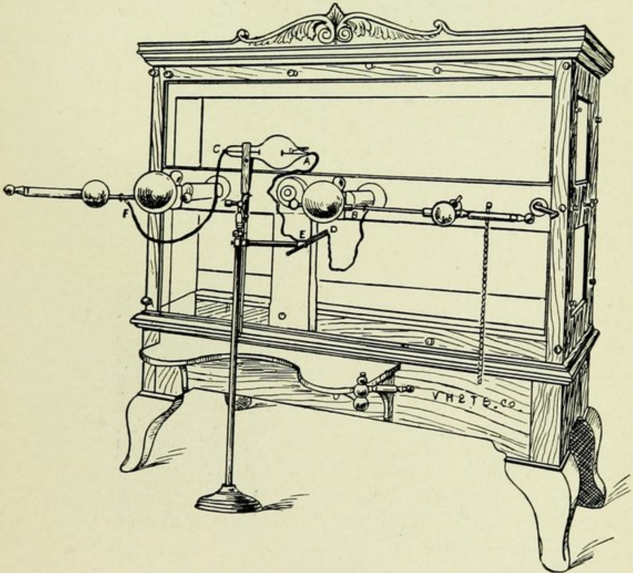
Fig. 5.—Files Interrupter in Circuit.
