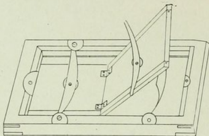
Fig. 21.—Printing Frame.
