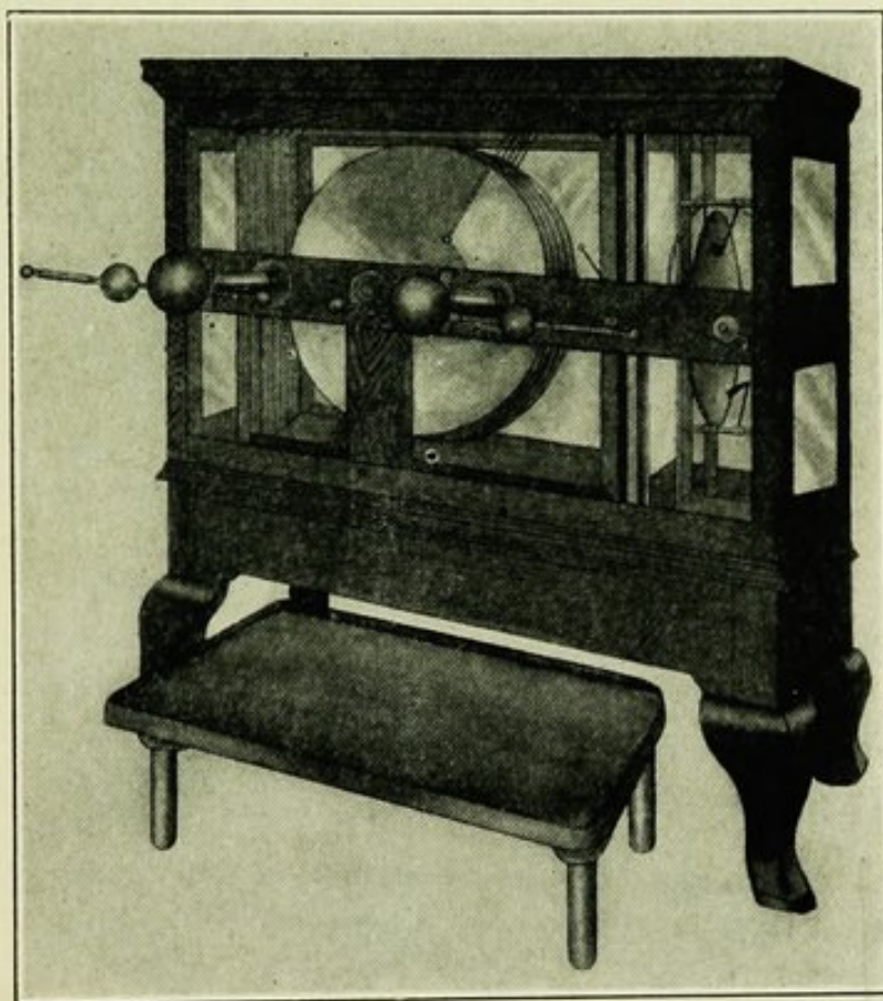
Fig. 2.—A Modern Holtz Machine.
