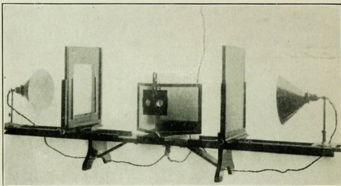
Fig. 22.—X-Ray Stereoscope.
