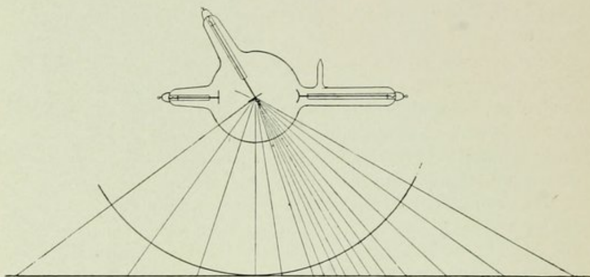
Fig. 18.—Showing Radio-active Field and Occasion for Distortion.
