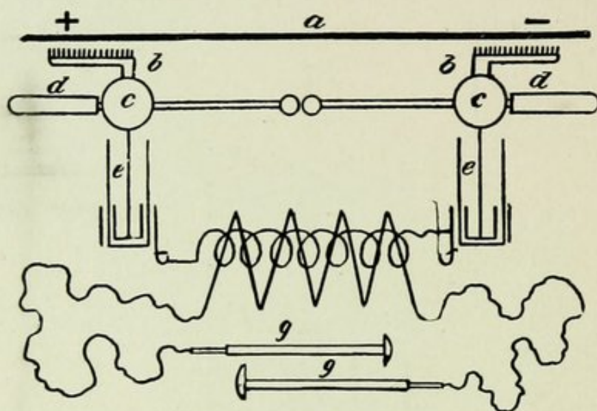
Fig. 33.— a , Revolving Plate ; b , Collecting Combs ; c , Prime Conductors ; d , Discharging Rods ; e , Leyden Jars ; g , Electrode.
