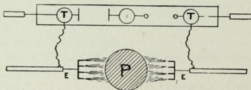
FIG. 170.—Double Effluvation from the Author's Apparatus.
