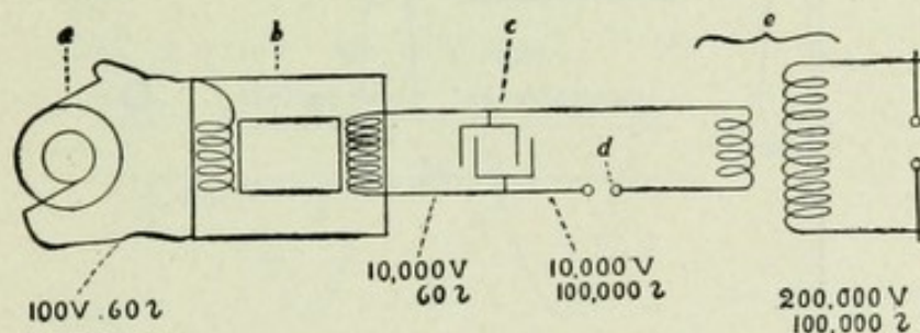
FIG. 89.—Arrangement for the Production of Tesla-Thomson Currents.
