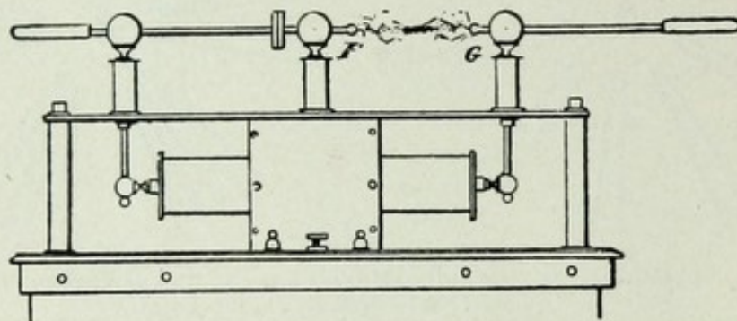
FIG. 99.—"Pseudo-Static Spark" from the Author's Hercules Machine.
