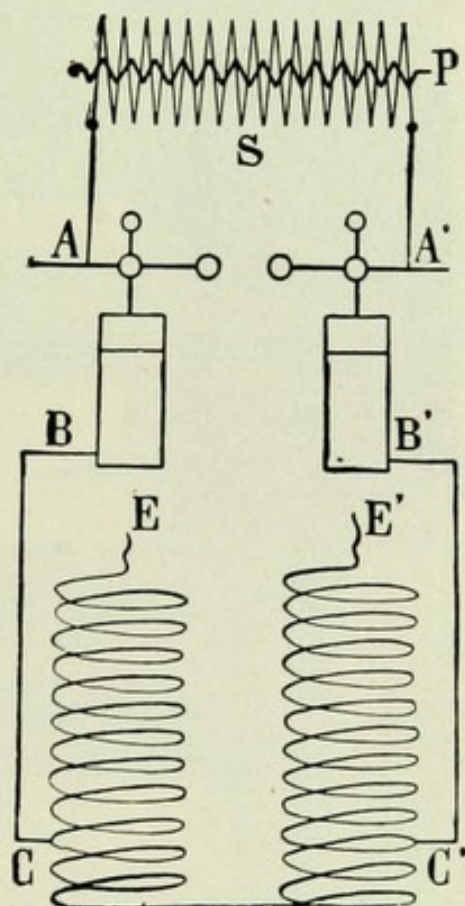
FIG. 41.—Rochefort's Bipolar Resonator. (Freund.)
