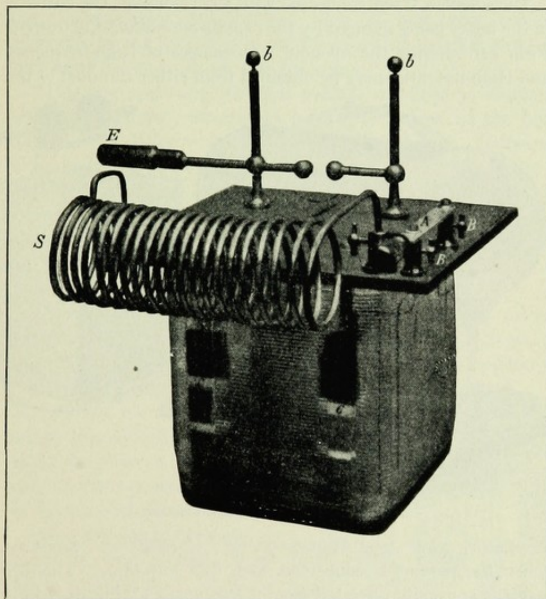
FIG. 44.—Gaiffe's Oil Condenser and Heavy Solenoid.
