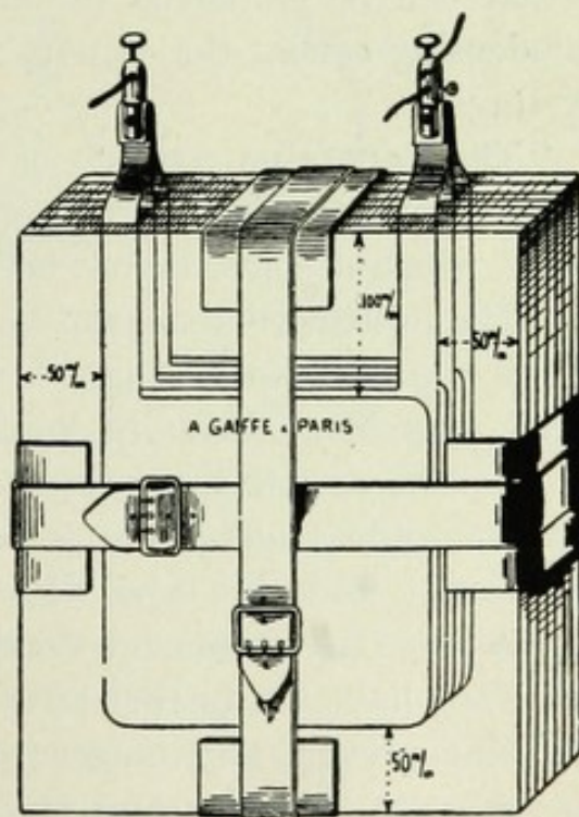
FIG. 46.—Condenser. (From Belot.)
