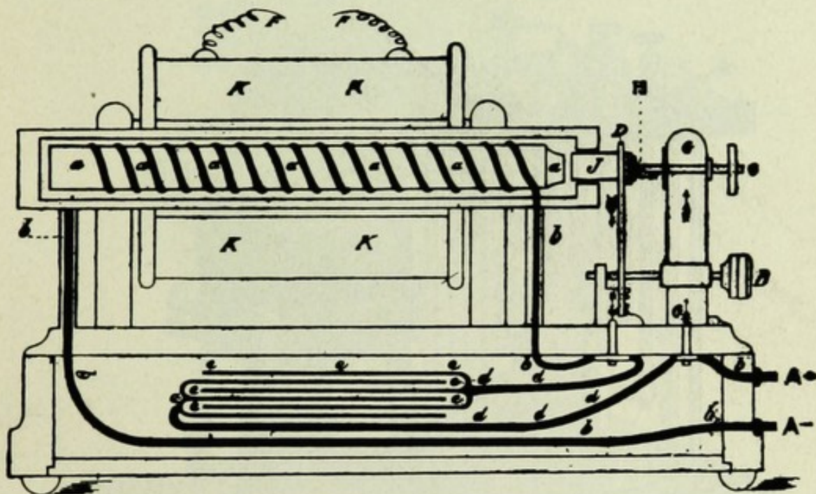
FIG. 34.—Ruhmkorff Induction Coil, Shown Diagrammatically. (Williams.)
