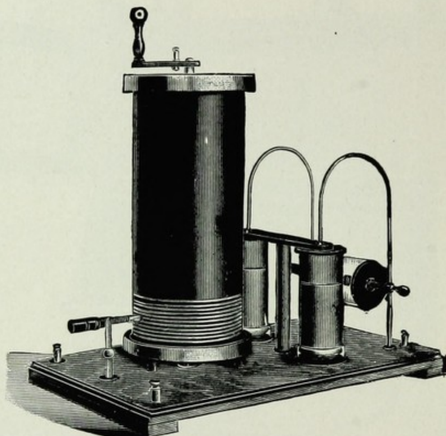
FIG. 56.—Resonator and Condensers (small model). (Williams.)
