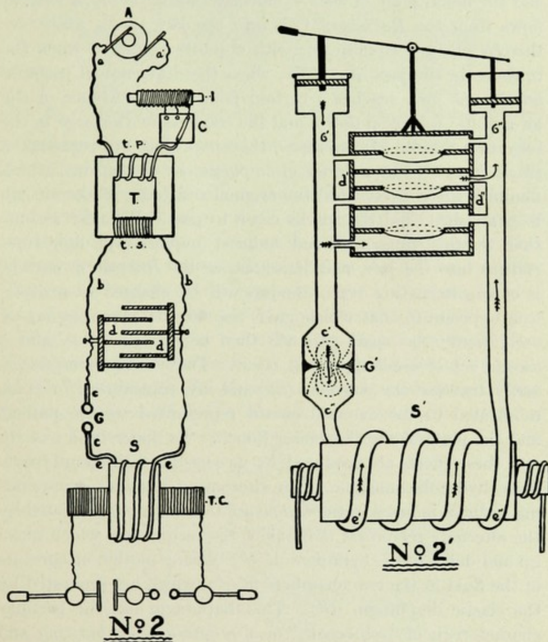
FIG. 27.—Plate II. Tesla-Thomson Circuit and Hydraulic Analogue.
