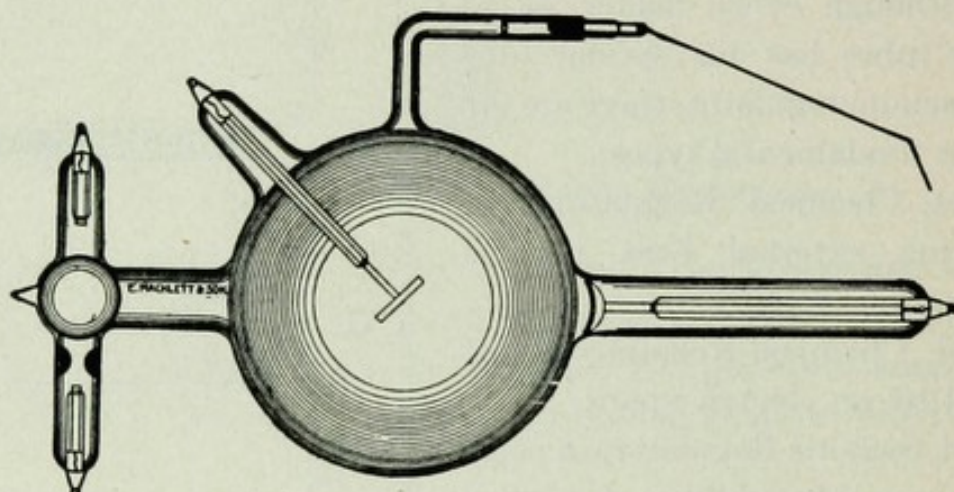
FIG. 142 — "Self-regulating" X-Ray Tube.
