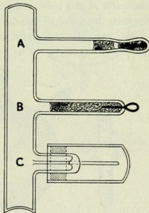
FIG. 141.—Vacuum Regulators for X-Ray Tubes.
