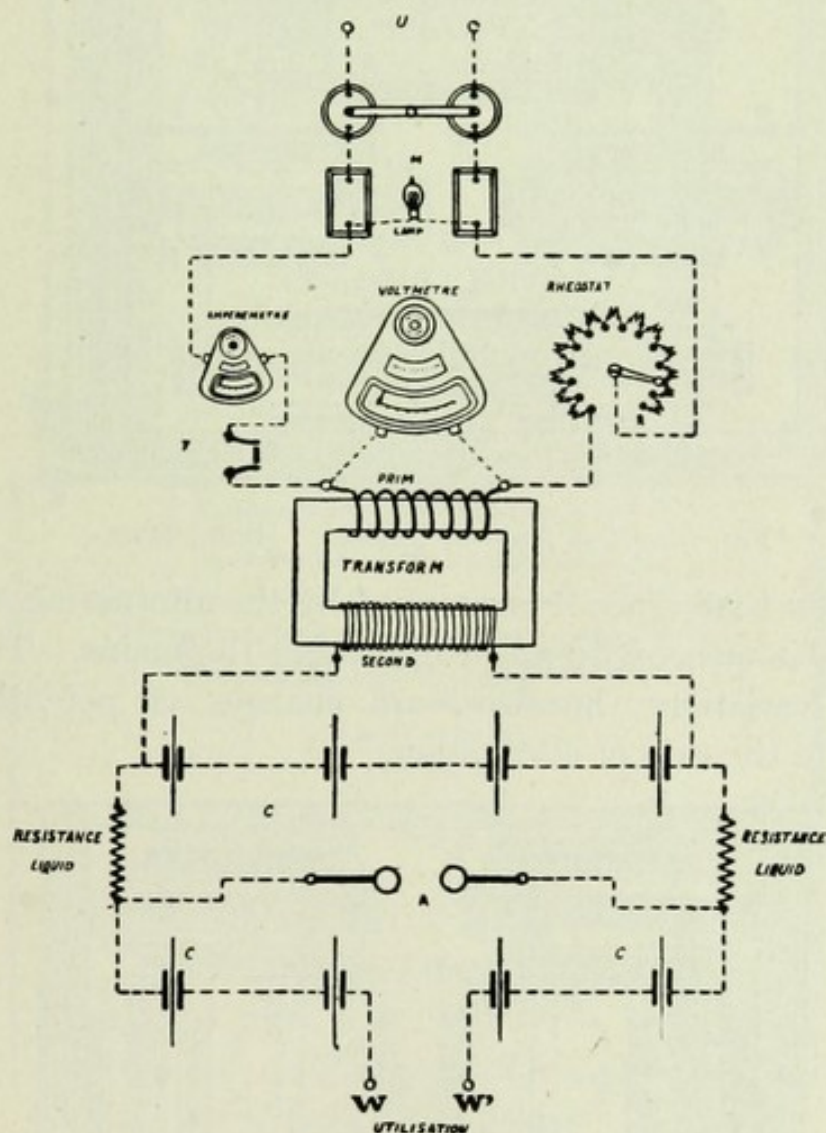
FIG. 50.—General Diagram. (From Belot.)
