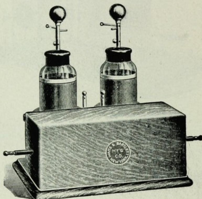
FIG. 12.—Piffard's "Hyperstatic Transformer."
