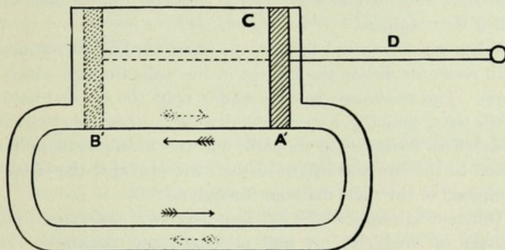
FIG. 19.—Hydraulic Analogue of “Alternating Current” Circuit.
