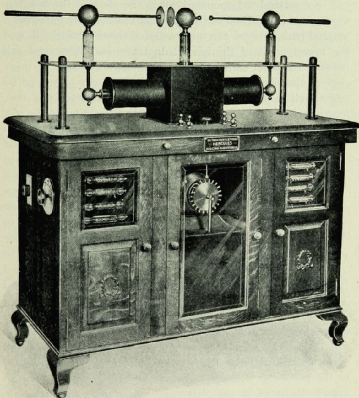
Fig. 76.—The Author's "Hercules" High-frequency Apparatus.
