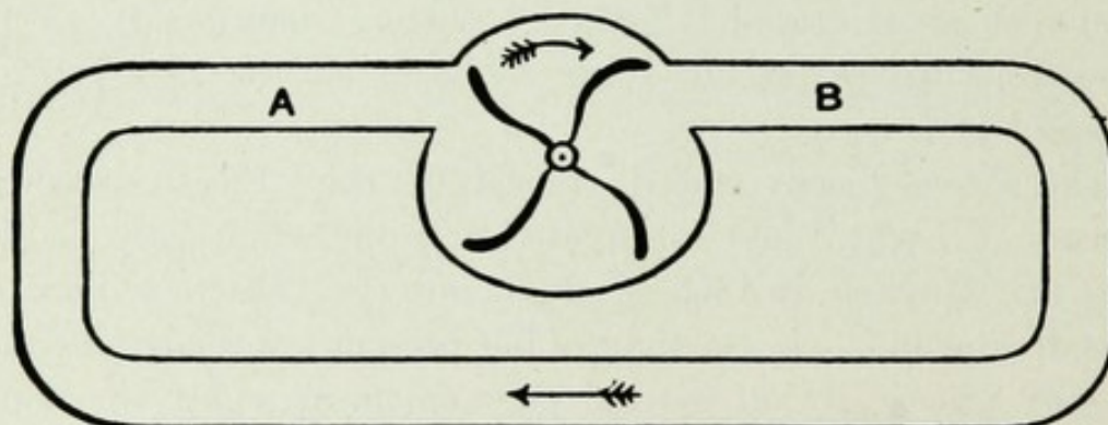
FIG. 18.—Hydraulic Analogue of “Continuous Current” Circuit.
