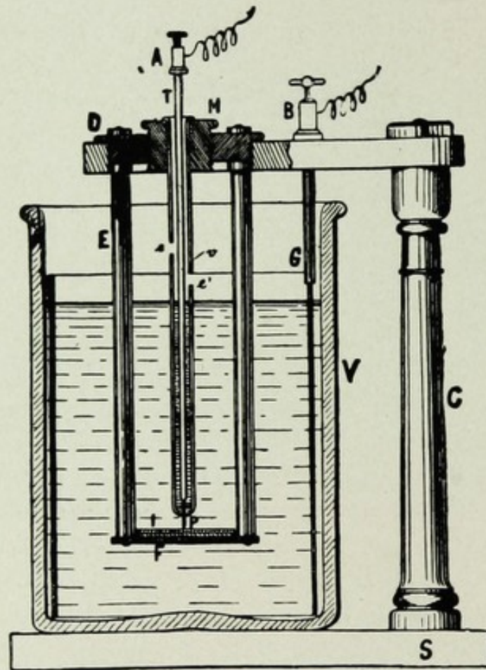
FIG. 31.—Electrolytic Interrupter of Wehnelt. (Williams.)
