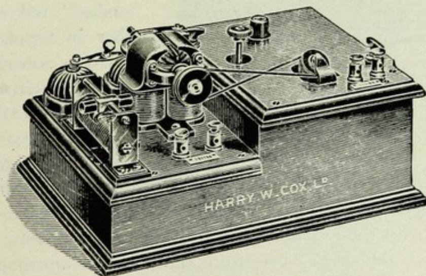
FIG. 37.—Mackenzie-Davidson Interrupter.
