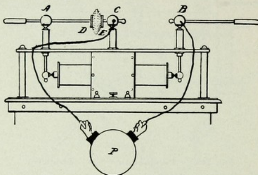
FIG. 119.—High-frequency "Motor-Wave Current."
