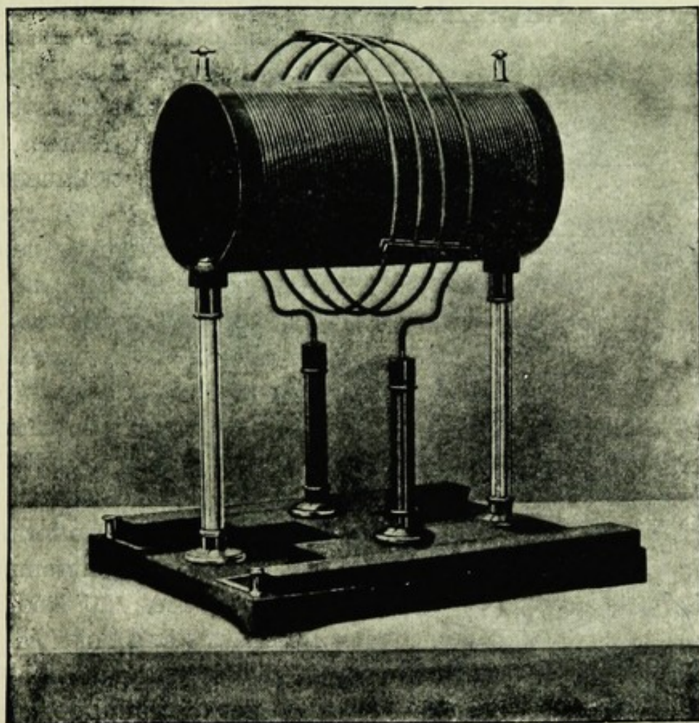
FIG. 7.—D'Arsonval Bipolar High-tension Coil. (Williams.)
