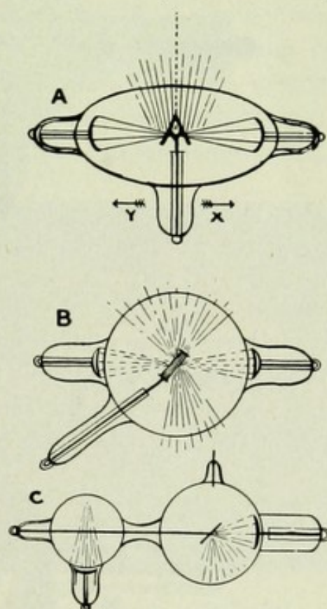
FIG. 143.—Types of "High-frequency X-Ray Tubes."
