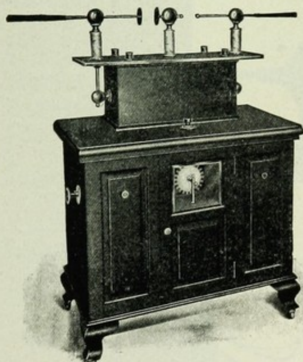
FIG. 70.—The Author's "Special Hercules" Coil.
