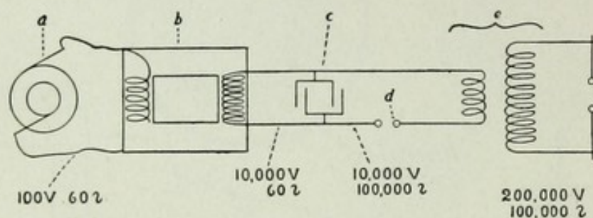
FIG. 62.—Tesla-Thomson High-frequency Apparatus.
