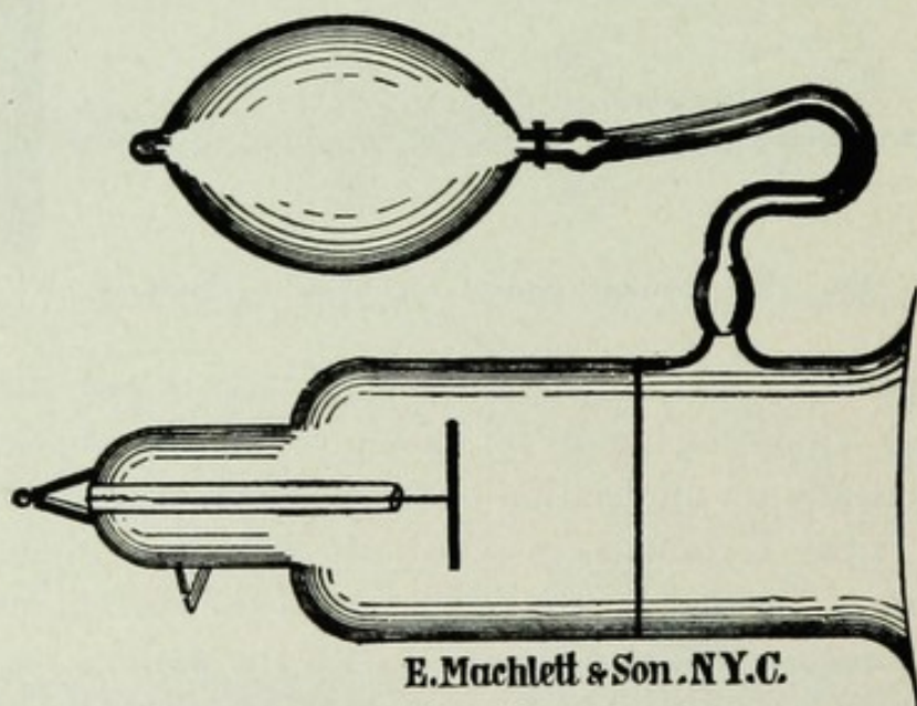
FIG. 132.—Vacuum Condenser Electrode with Cupping Device.
