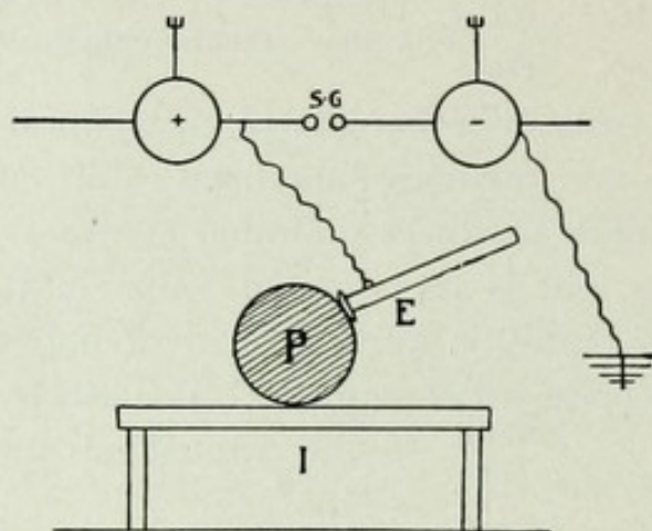
FIG. 157.—Diagram of Static Wave Current.
