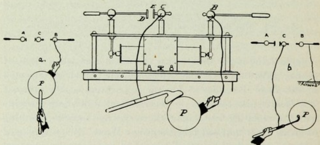
FIG. 167.—The Author's Technic for Vacuum Electrodes.
