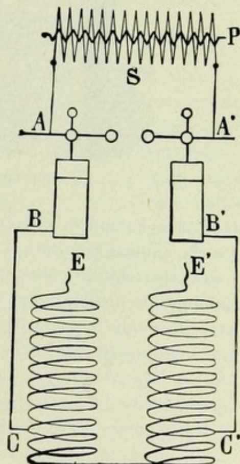
FIG. 11.—Rochefort's Bipolar Resonator. (Guilleminot.)
