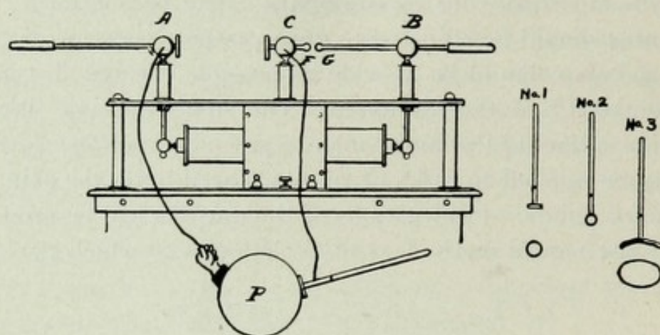
FIG. 166.—“Motor Impulse” Treatment.
