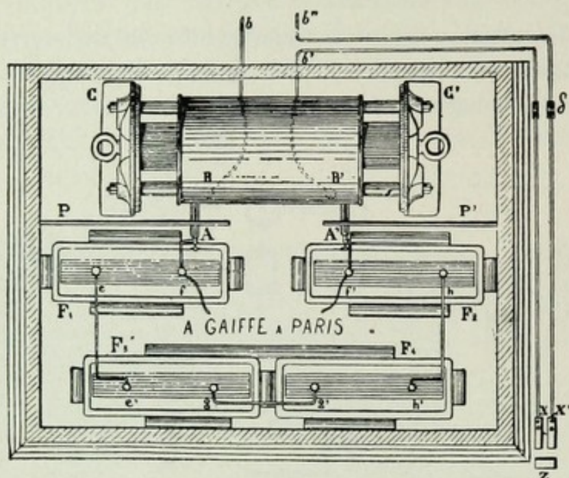
FIG. 51.—Top Shelf of Cabinet. (From Belot.)
