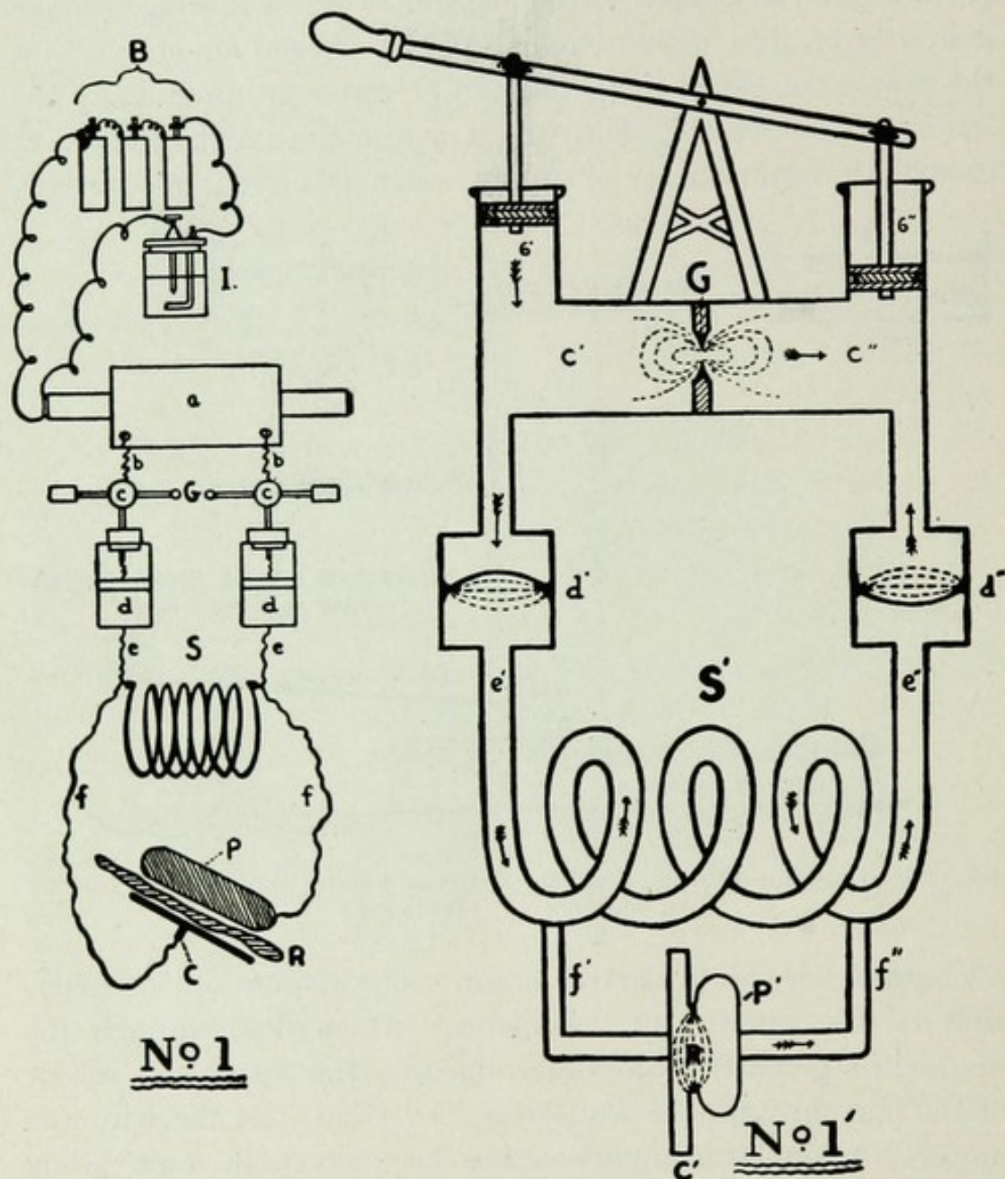
FIG. 27.—Plate I. D'Arsonval Circuit and Hydraulic Analogue.
