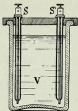
FIG. 47.—Liquid Resistances. (From Belot.)
