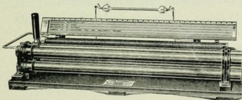
FIG. 107.—Professor Flemming's "Direct-reading Cymometer." (Marconi Wireless Telegraph Co.)
