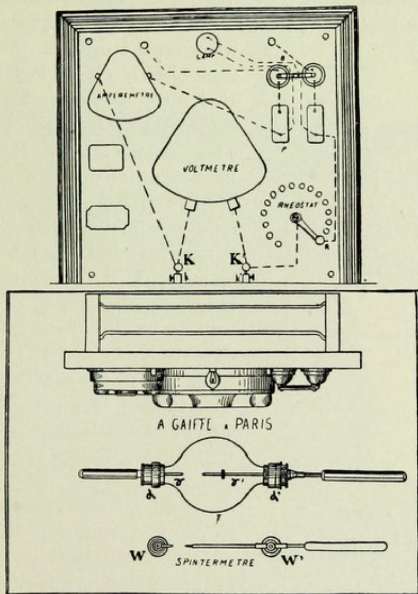
FIG. 53.—Springs and Contact Plate. (From Belot.)
