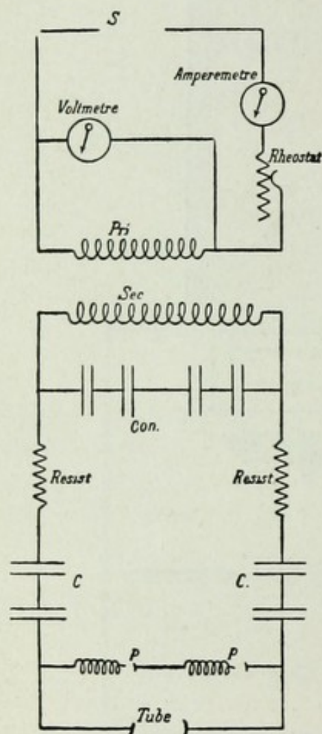
FIG. 54.—Regulating Apparatus. Arrangement of Transformer. (From Belot.)
