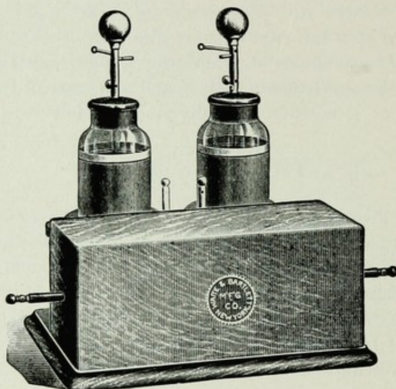
FIG. 63.—Piffard's Hyperstatic Transformer.
