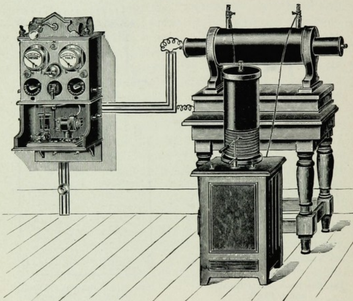
FIG. 42.—Upright Solenoid on Cabinet. (Williams.)
