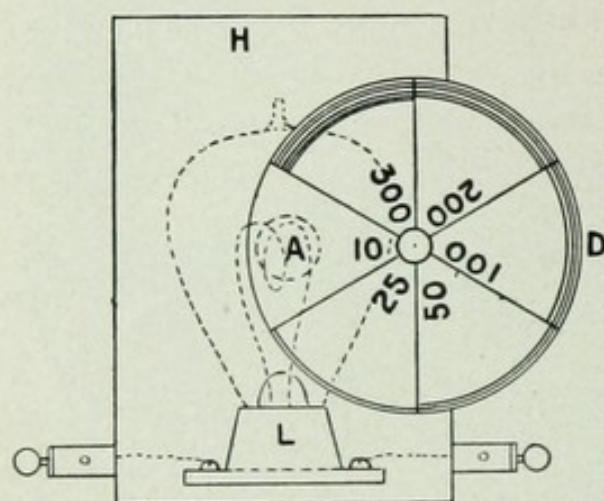
FIG. 106.—The Author's Photometric Mil-ammeter.
