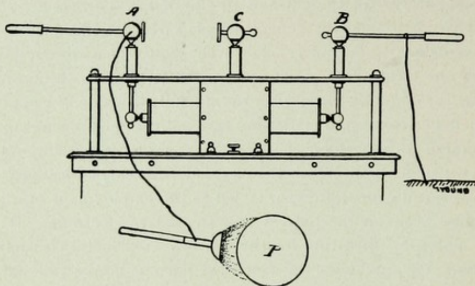
FIG. 13.—The Author's Air-gap Condenser Terminals.
