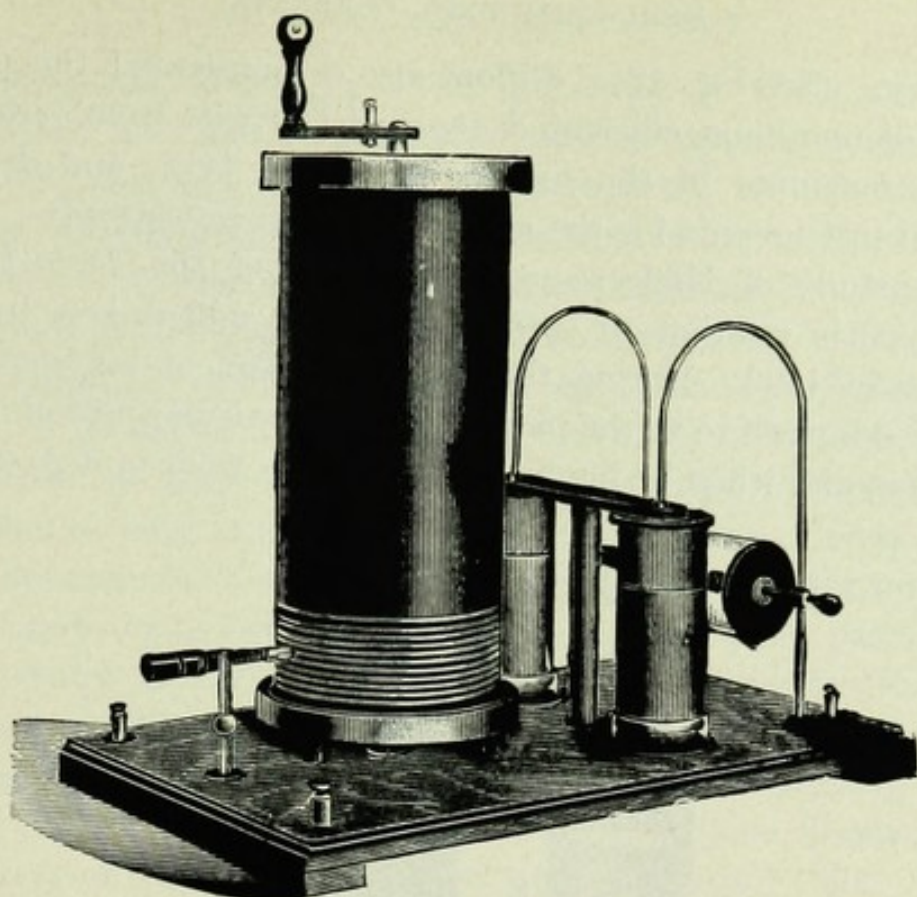
FIG. 9.—Oudin Resonator. (Williams.)
