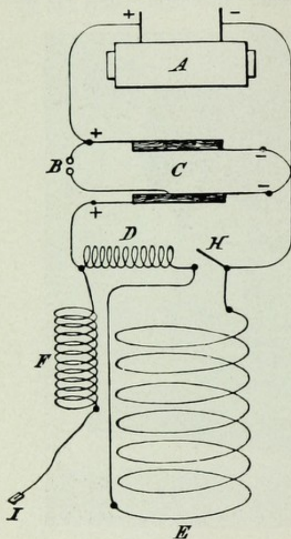
FIG. 8.—Diagram of Solenoid and Resonator. (Freund.)
