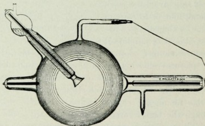
FIG. 140.—“Water-cooled” X-Ray tube.
