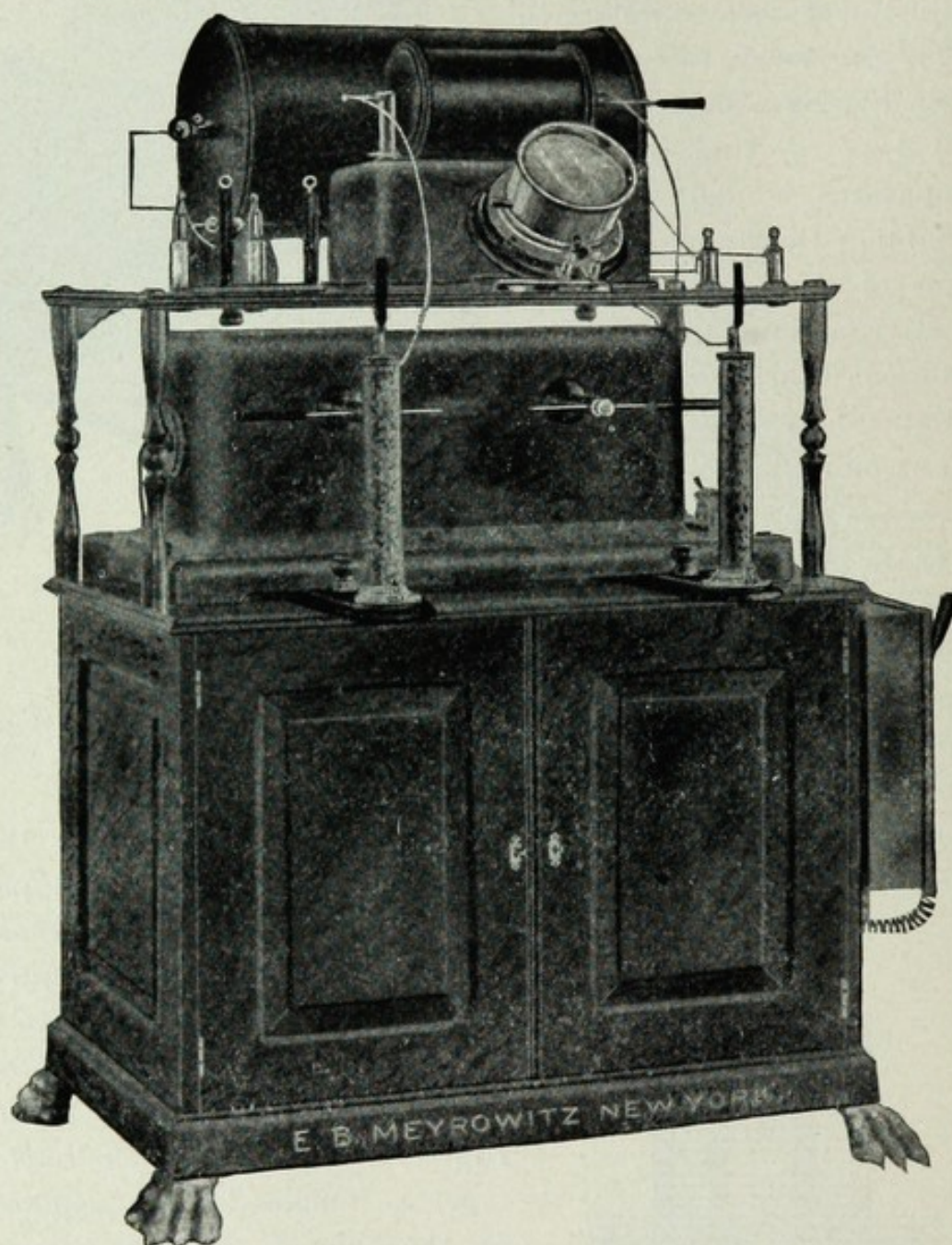
FIG. 82.— Meyrowitz High-frequency Apparatus.
