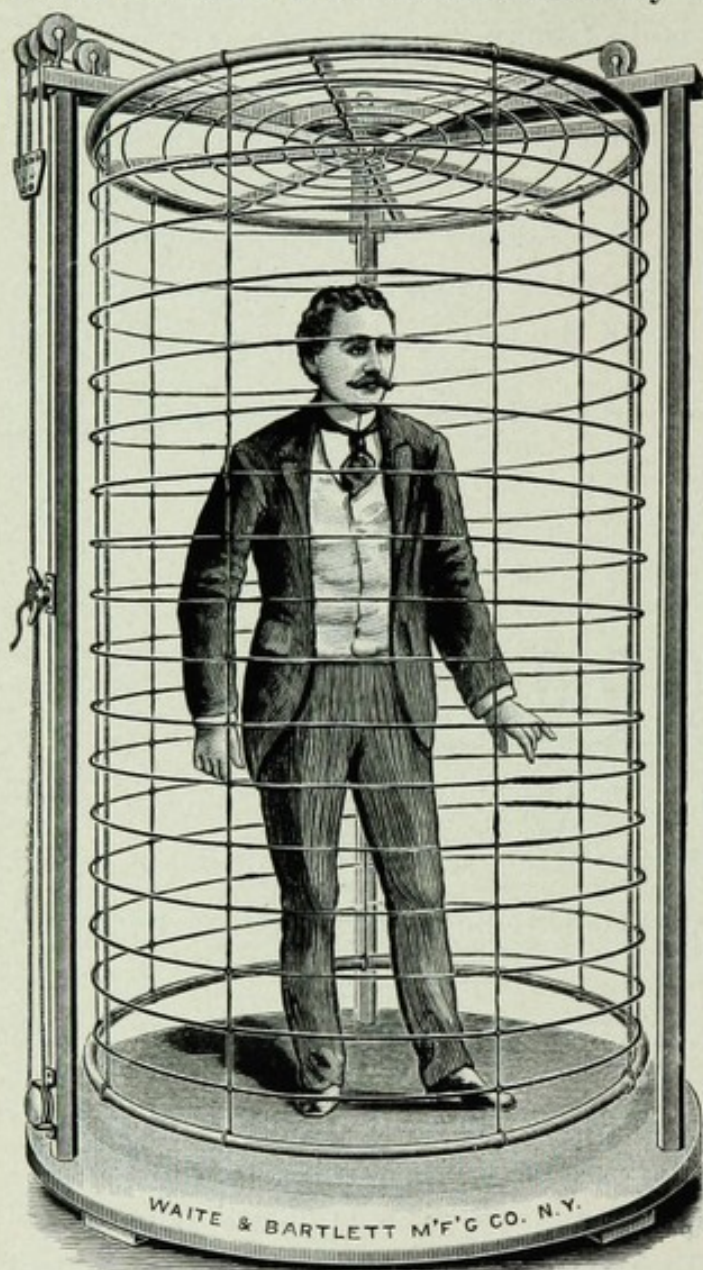
FIG. 2.—D'Arsonval Auto-Conduction Cage; Upright Form. (Piffard's.)
