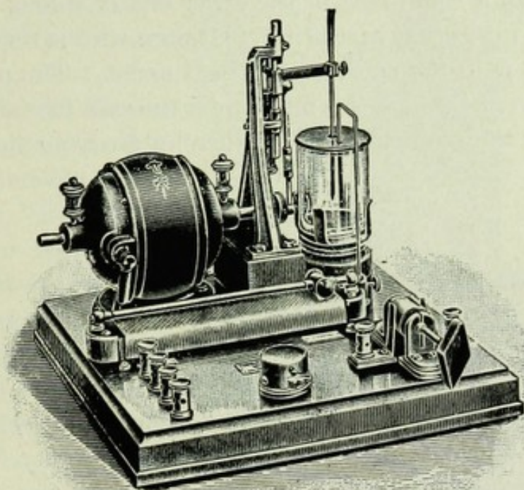
FIG. 36.—Dipper Mercury Interrupter.
