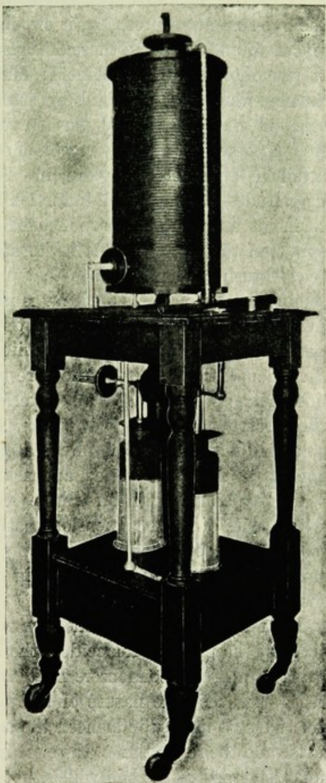
FIG. 39.—Oudin-Dean Resonator. (Williams.)
