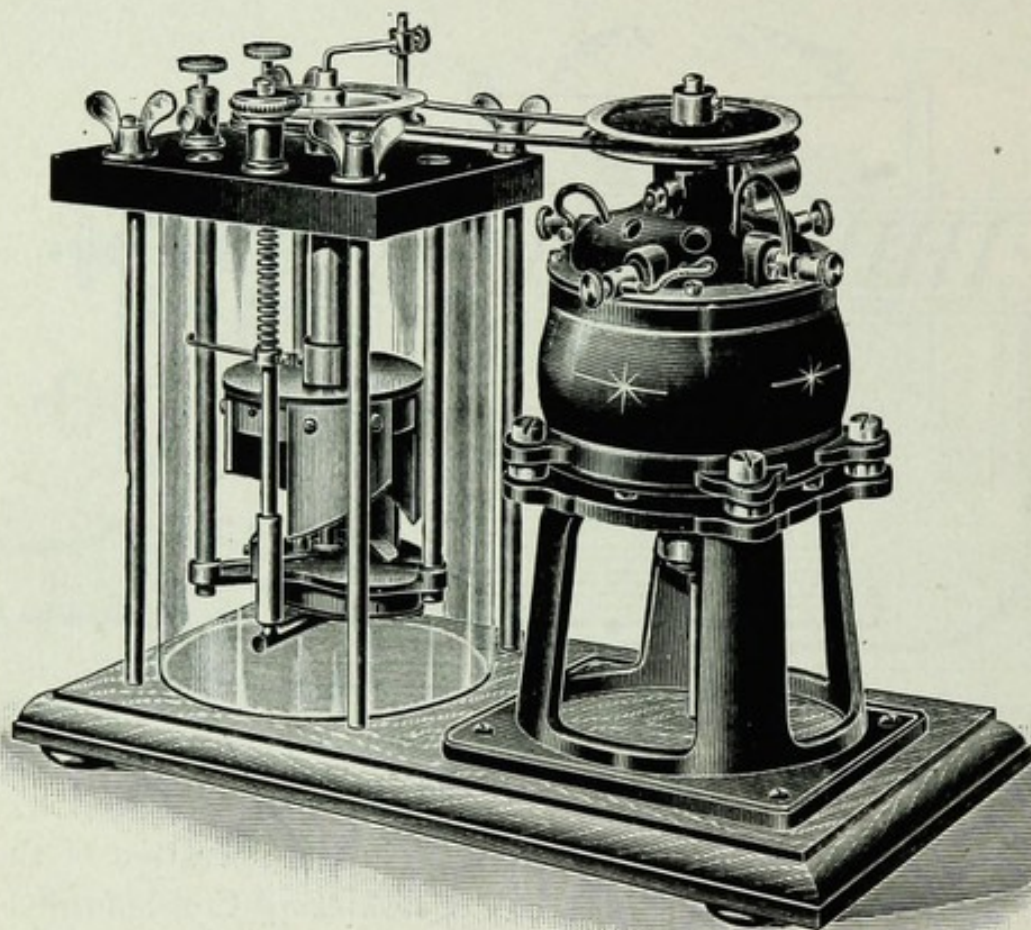
FIG. 35.—Mercury Jet Interrupter. (Isenthal & Co.)
