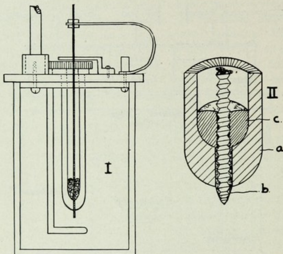
FIG. 85.—The Author's Improved Electrolytic Interrupter.
