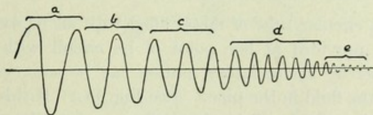
FIG. 17.—Diagram Indicating Wave Length and Frequency of Known Forms of Radiant Energy.
