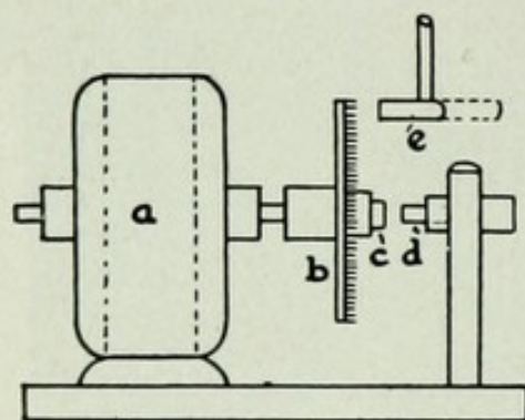
FIG. 77.—The Author's Improved Rotary Spark-gap.
