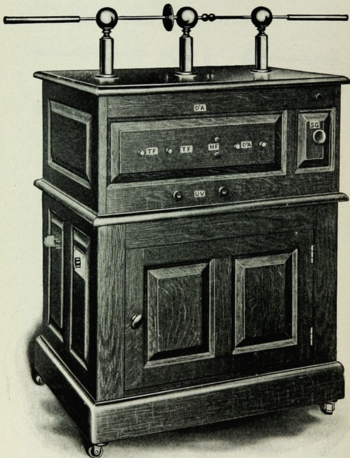
FIG. 73.—The "Ajax Special Coil."
