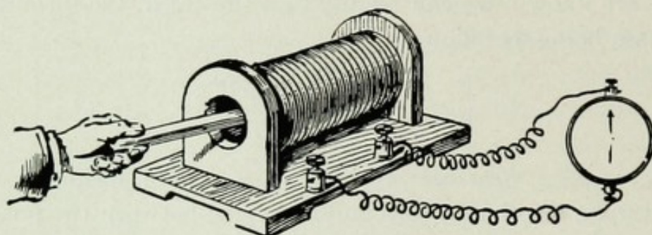
FIG. 21.—Magnetic-electric Induction. (Williams.)
