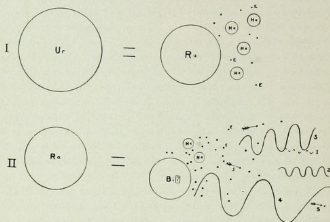
FIG. 15.—Schematic Diagram Showing Spontaneous Degeneration of Atoms.
