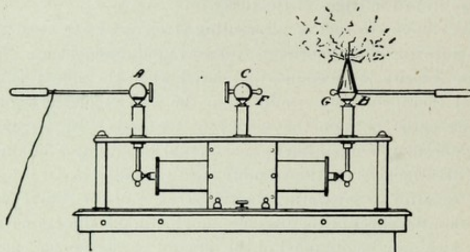
FIG. 100.—Resonator Discharge from Terminal of Tesla Coil.
