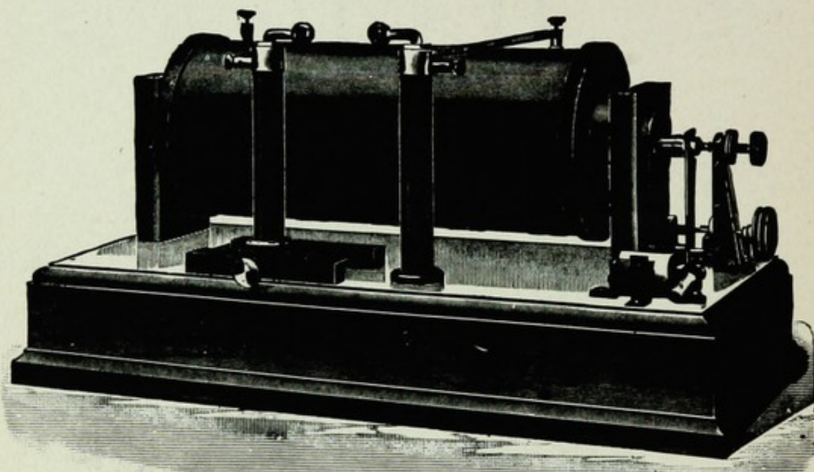
FIG. 33.—Ruhmkorff Induction Coil. (Watson, London.)
