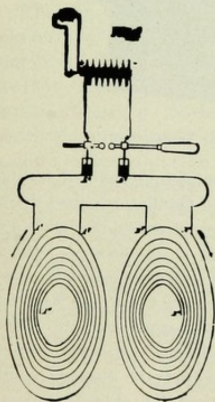
Fig. 10.—Bipolar Resonator of O'Farrell.
