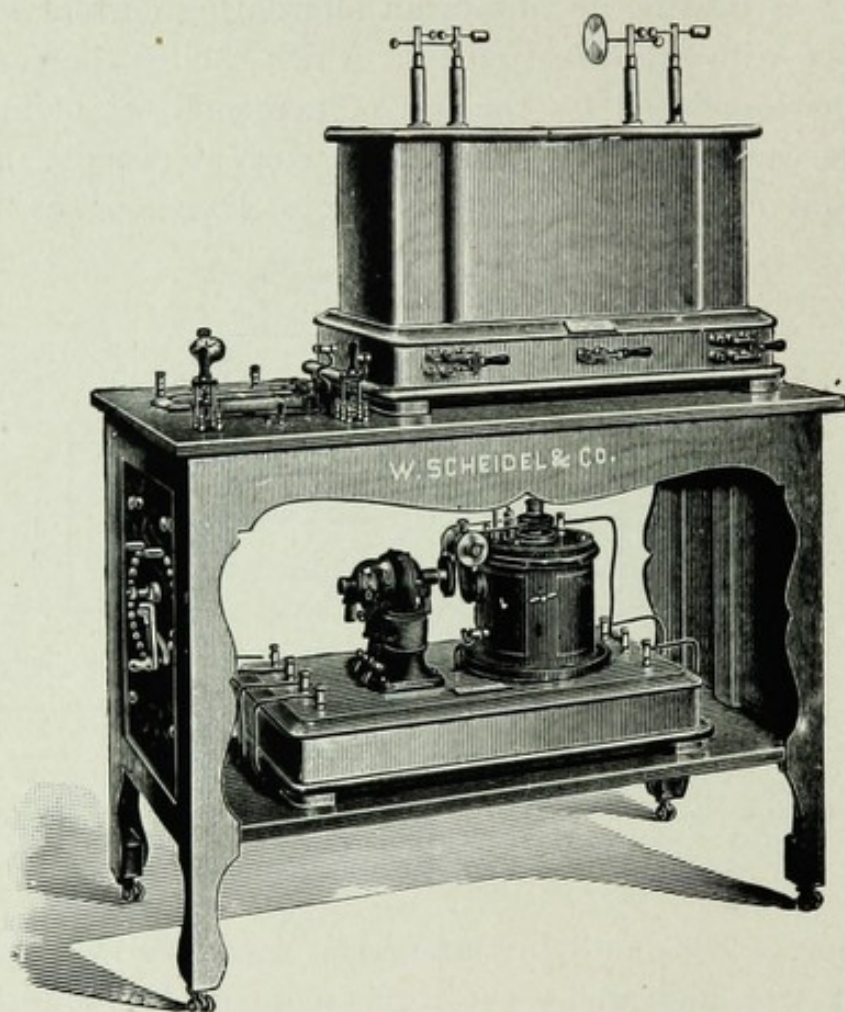
FIG. 79.—“Scheidel-Western” Coil for Exciting High-frequency Apparatus.
