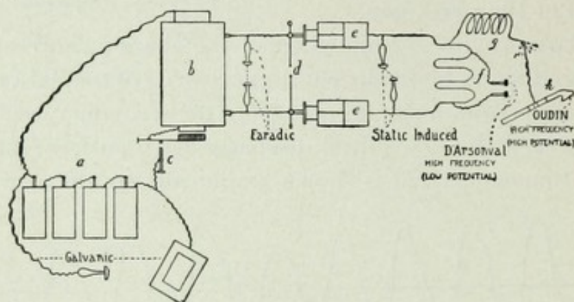
FIG. 88.—Arrangement for the Production of Oudin-d'Arsonval Currents.
