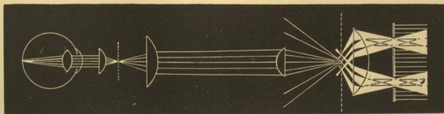
FIG. 90. ARRANGEMENT BY WHICH THE PREPARATION IS ILLUMINATED BY HOLLOW, AND IMAGED BY SOLID, BEAMS.
