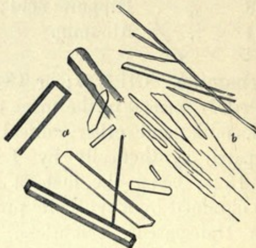
Fig. 8.—CRYSTALS OF UREA— a , Quadrangular prisms; b , Indefinite crystals, as deposited from alcoholic solutions.
