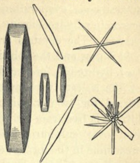
Fig. 14.—CREATININE (after Frey).
