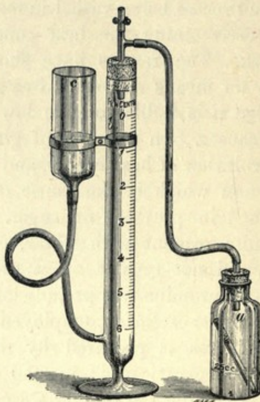
Fig. 10.—GERRARD'S UREOMETER.
