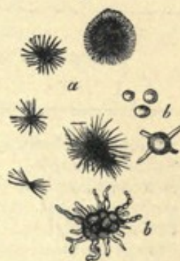
Fig. 17. — ACID SODIUM URATE. (After Frey).
