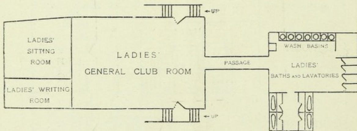
CLUB HOUSE FOR LADY EMPLOYEES—FIRST FLOOR PLAN
