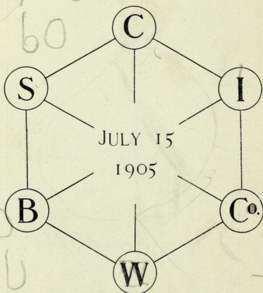
THE BENZENE RING RE-CAST
