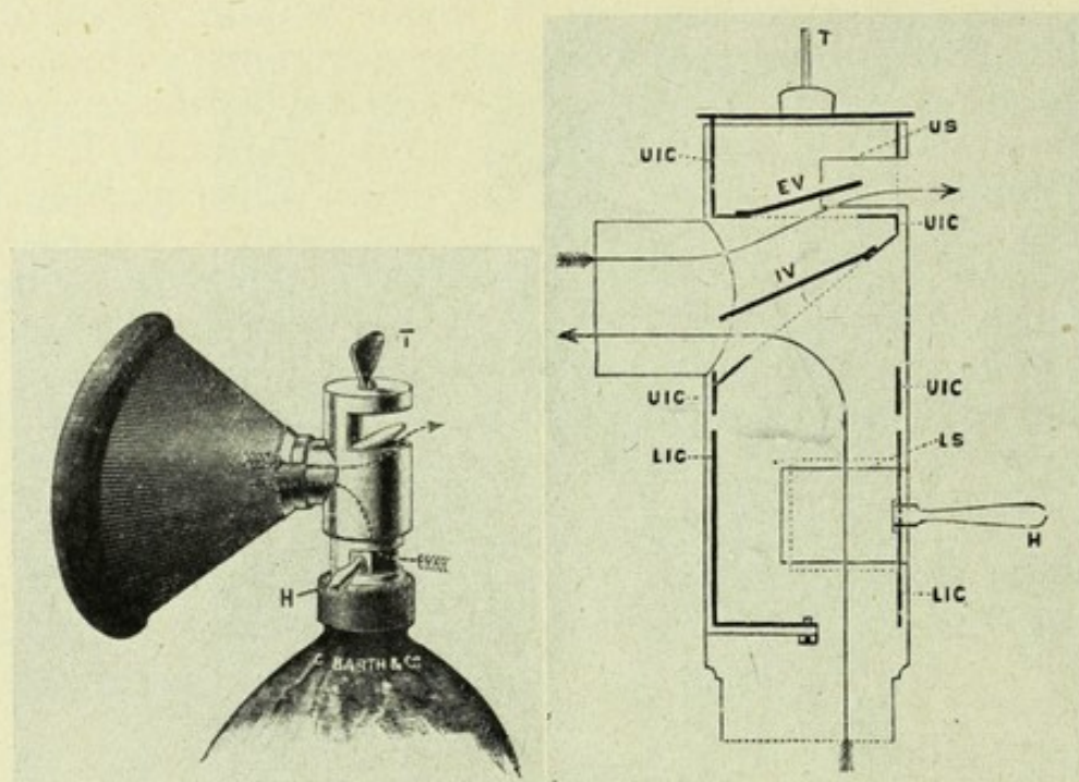
FIG. 125.—HEWITT'S VALVED STOPCOCK (VS in Fig. 124)
