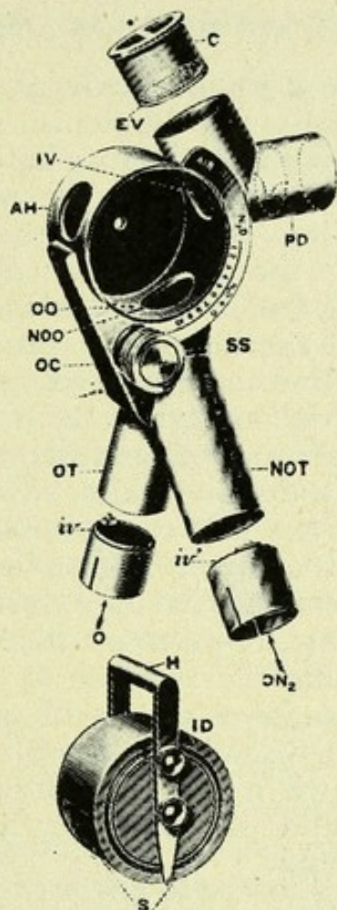
FIG. 132.—REGULATING STOPCOCK AND MIXING CHAMBER OF HEWITT'S APPARATUS FOR NITROUS OXIDE AND OXYGEN, 1897 (see also Fig. 131)
