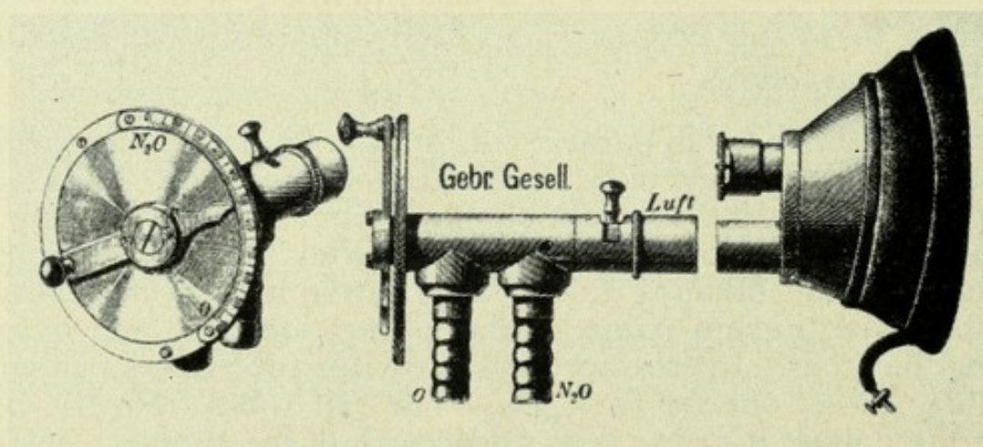
FIG. 128.—NITROUS OXIDE AND OXYGEN APPARATUS
