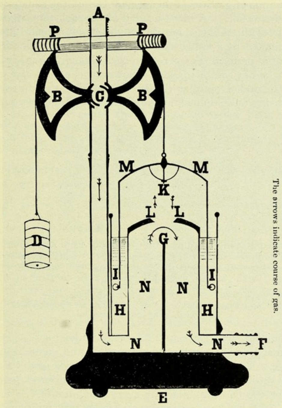
FIG. 77.—HELE'S GOVERNOR
