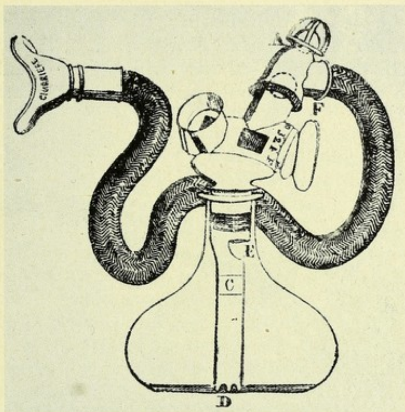
FIG. 18.—CHARRIÈRE'S INHALER for ether, in use in Paris during 1847.
