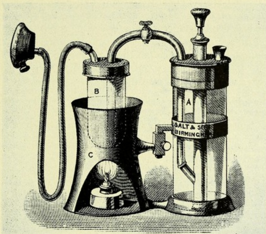
FIG. 157.—LAWSON TAIT'S WARMED ETHER INHALER (1876)
