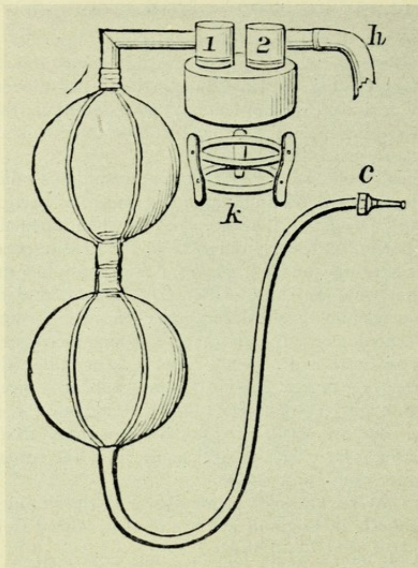
FIG. 72.—COLEMAN'S 'ECONOMISING APPARATUS' for absorbing carbon dioxide from the patient's exhalations during to-and-fro breathing in nitrous oxide anaesthesia.
