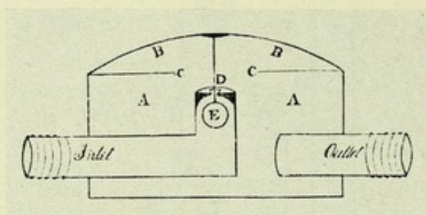
FIG. 78.—HELE'S REGULATOR
