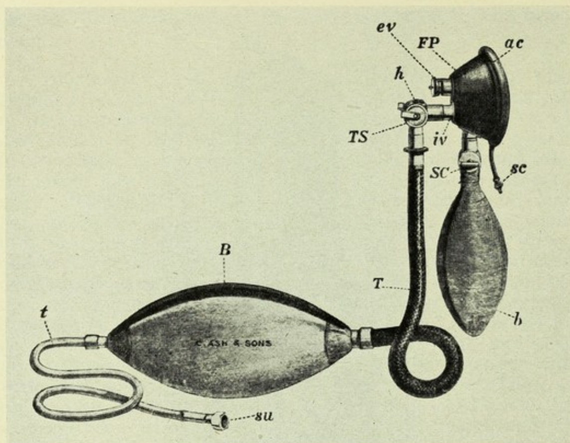
FIG. 74.—LATER MODEL, c. 1890, OF THE TYPE OF NITROUS OXIDE APPARATUS
