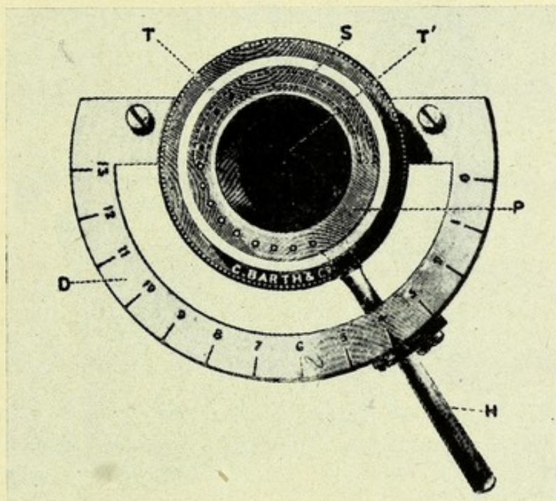
FIG. 130.—THE REGULATING MECHANISM OF HEWITT'S NITROUS OXIDE-OXYGEN APPARATUS
