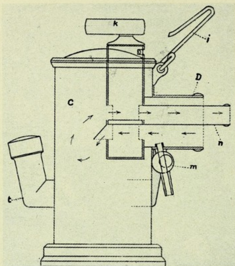
FIG. 84.—DIAGRAM OF THE ETHER VESSEL OF CLOVER'S 'COMBINED GAS-AND-ETHER APPARATUS', IN SECTION
