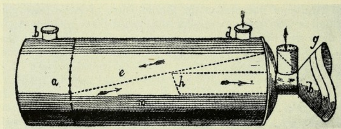
FIG. 20.—SMEE'S INHALER
