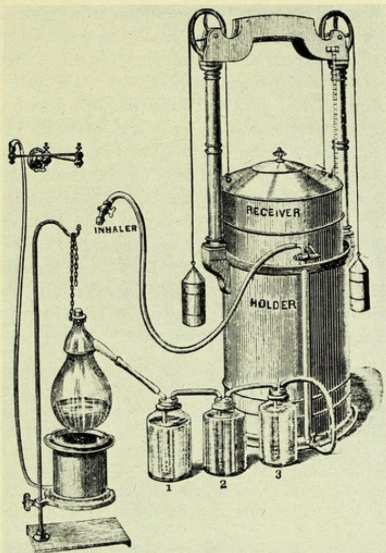
FIG. 68.—TYPE OF APPARATUS DESIGNED BY SPRAGUE (c. 1863) FOR GENERATING, PURIFYING AND COLLECTING NITROUS OXIDE GAS
