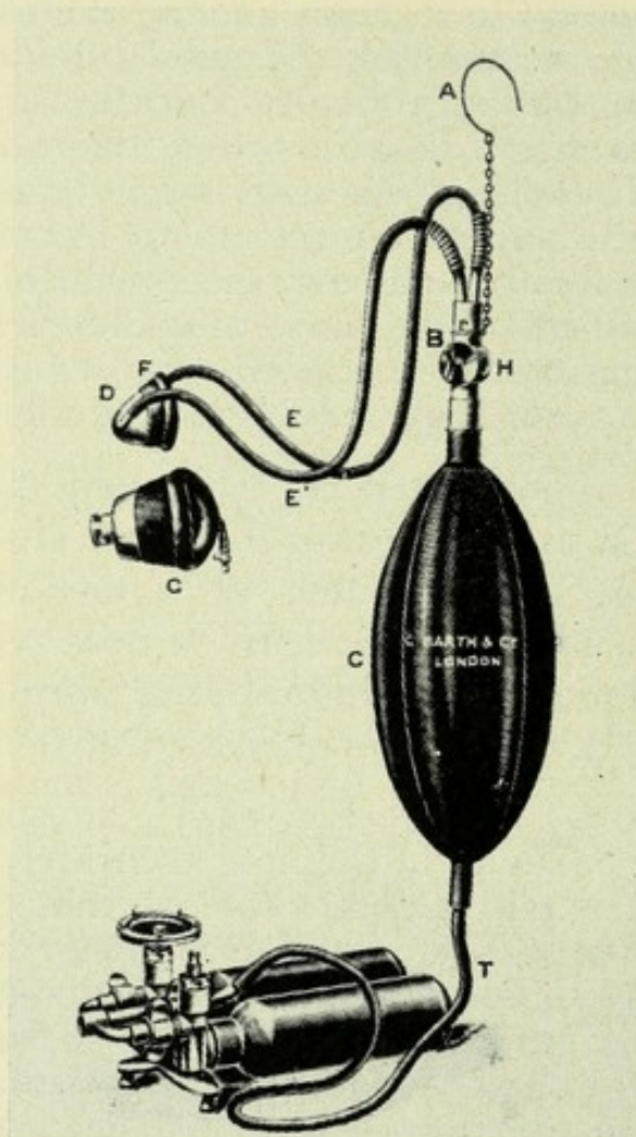
FIG. 134.—PATERSON'S APPARATUS FOR MAINTAINING NITROUS OXIDE ANAESTHESIA THROUGH THE NOSE (1899)
