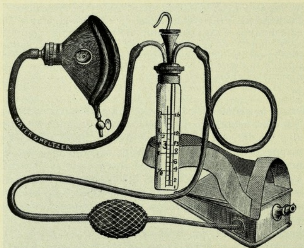
FIG. 118.—BUXTON'S MODIFICATION OF JUNKER'S CHLOROFORM INHALER
