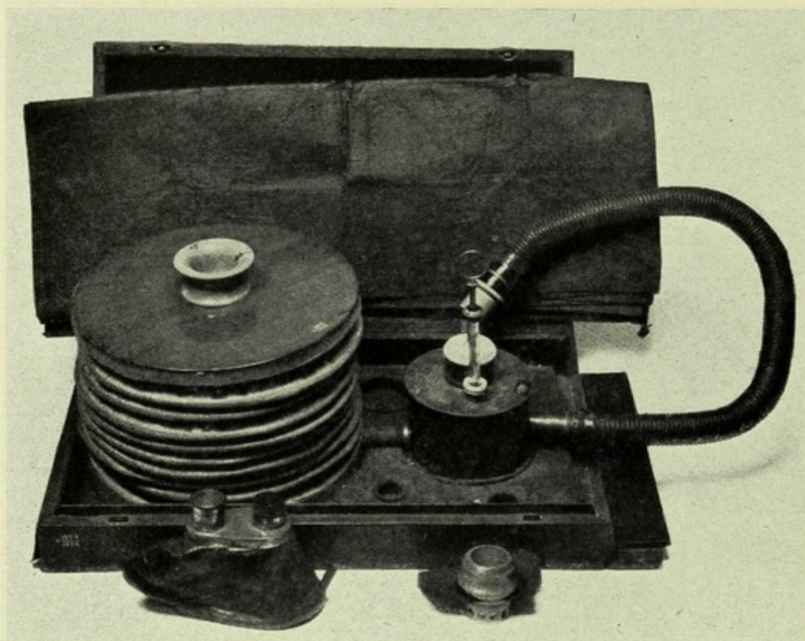
FIG. 55.—A CLOVER'S CHLOROFORM APPARATUS
