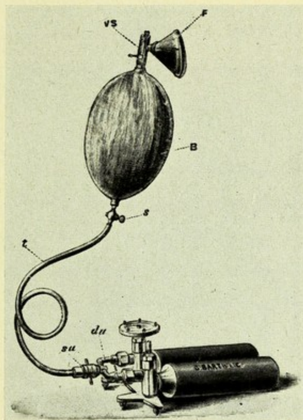
FIG. 124.—HEWITT'S APPARATUS for administering nitrous oxide gas, in use in 1893.
