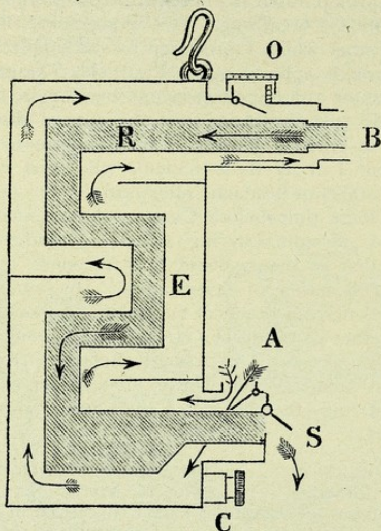
FIG. 82.—CLOVER'S 'DOUBLE-CURRENT INHALER' FOR ETHER (March 1873)
