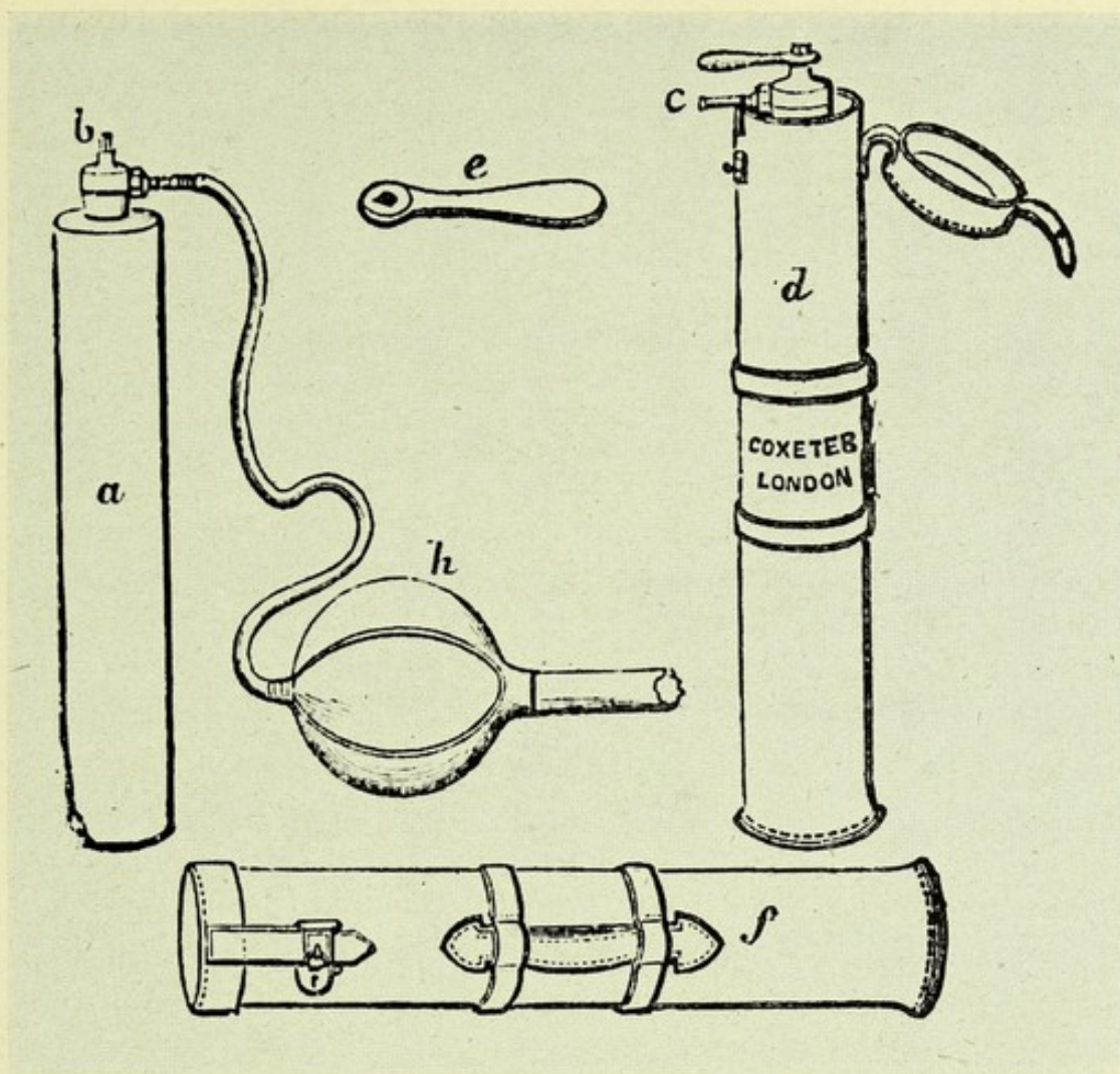
FIG. 75.—COXETERS' PORTABLE APPARATUS FOR COMPRESSED NITROUS OXIDE (1869)
