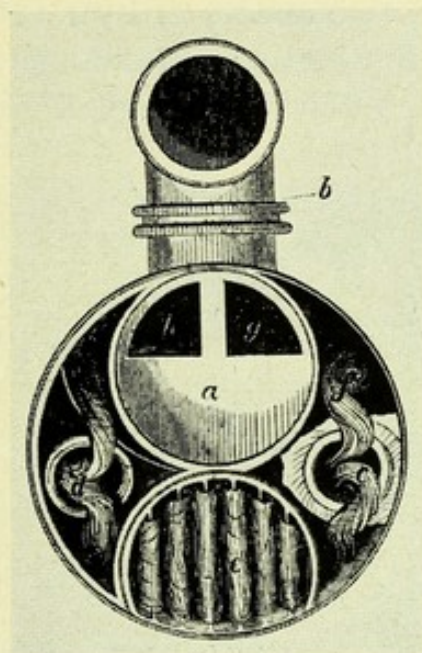
FIG. 62C.—ELLIS'S APPARATUS (see Fig. 62B)
