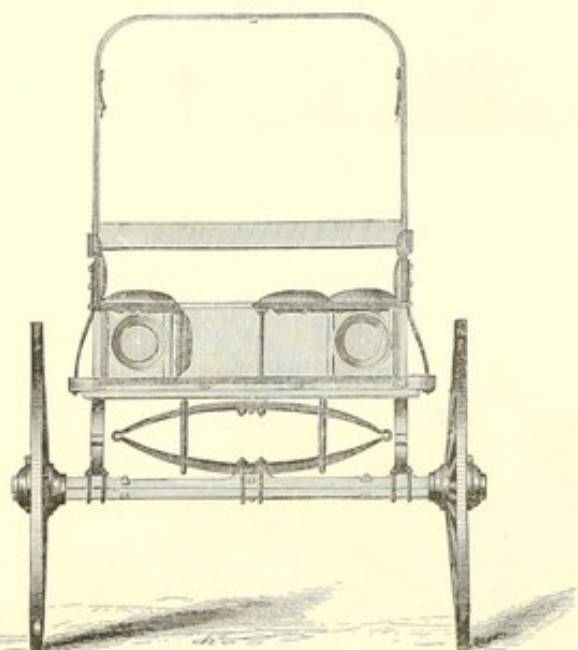
FIG. 87.—Rear elevation of the Wheeling ambulance.
