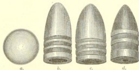
FIG. 96.— a. U. S. round musket-ball, calibre 69, weight 357 grains; b. Springfield rifled musket-ball, calibre 58, weight 500 grains; c. Enfield rifled musket-ball, weight 450 grains; d. Austrian rifle-ball, weight 460 grains.
