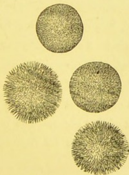
FIG. 6.—Globular masses composed of acicular crystals of Tyrosin.
