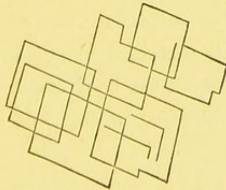
FIG. 3.—Crystalline Plates of Cholesterin.
