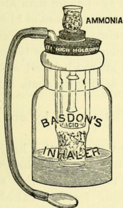
FIG. 28.—Basdon's inhaler.
