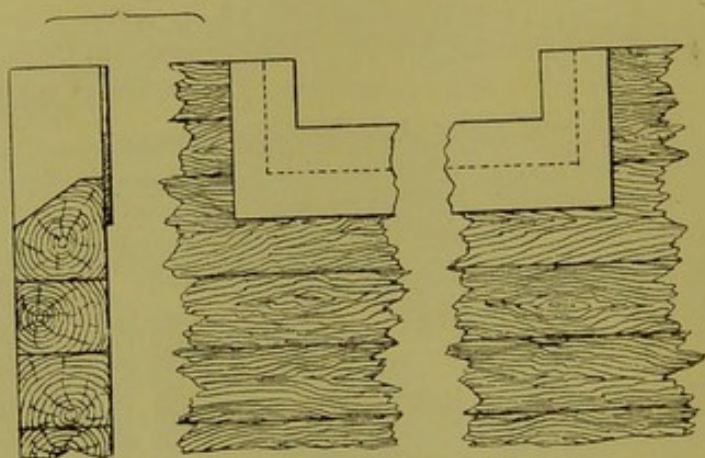
Fig. 3.—Metal plate for weir or notchboard for gauging streams.
