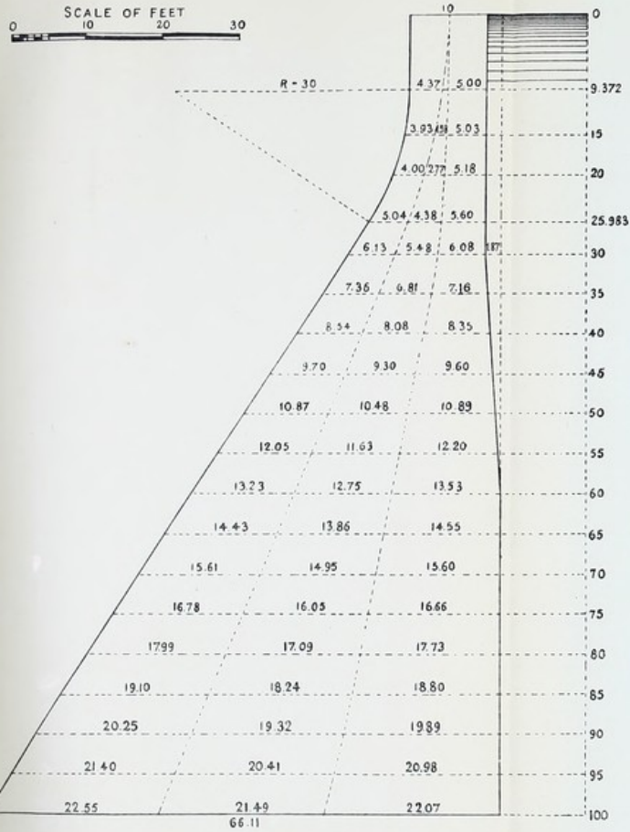
Fig. 52.—Practical Profile No. 2.
