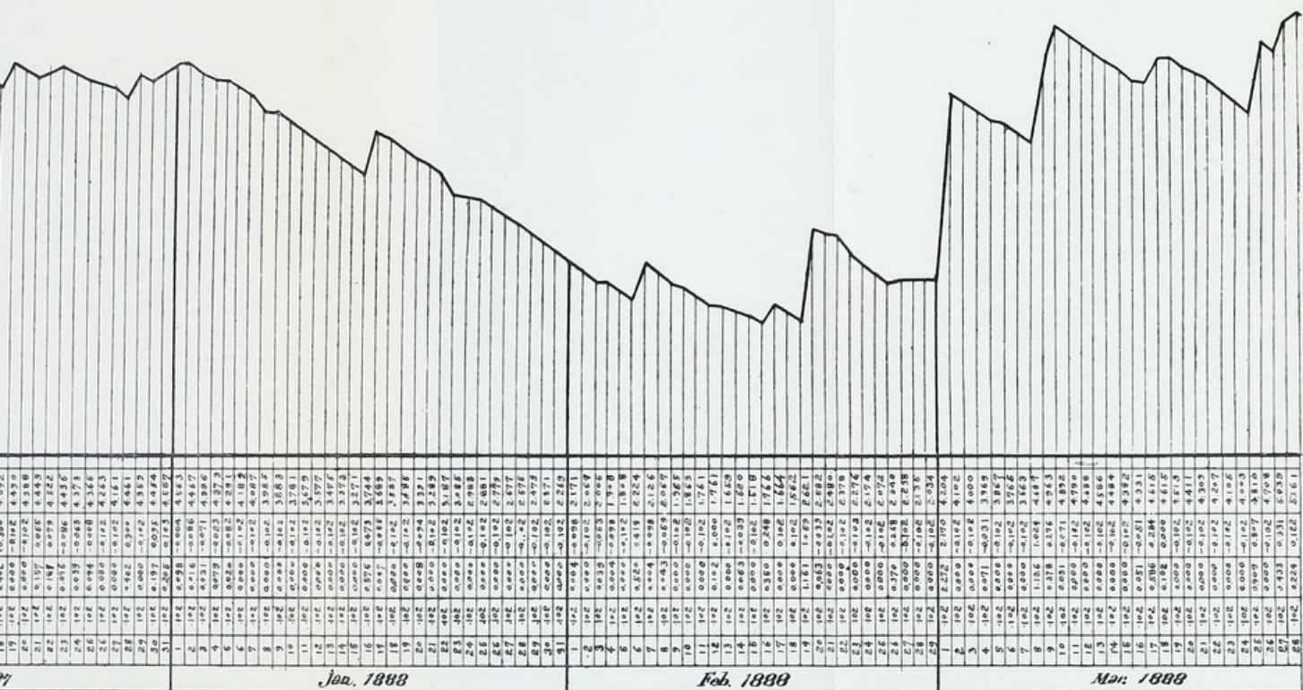
GRAM ILLUSTRATING REQUIRED STORAGE CAPACITY (DAILY RAINFALL).
