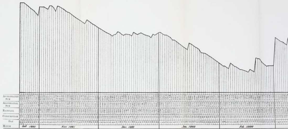
FIG. 6.—DIAGRAM ILLUSTRATING REQUIRED STORAGE CAPACITY (DAILY RAINFALL).
