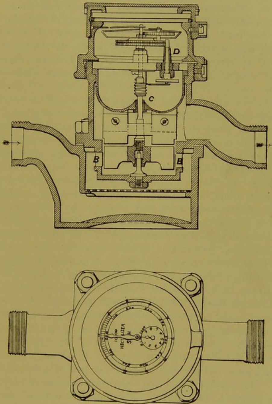
Figs. 233, 234.—Siemens and Halske's patent water meter.
