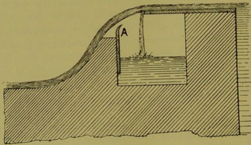
Fig. 47.—Arrangement for directing flow into reservoir.
