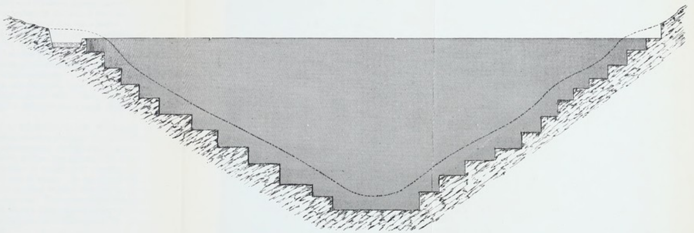
FIG. 29.—SECTION OF PUDDLE TRENCH.
