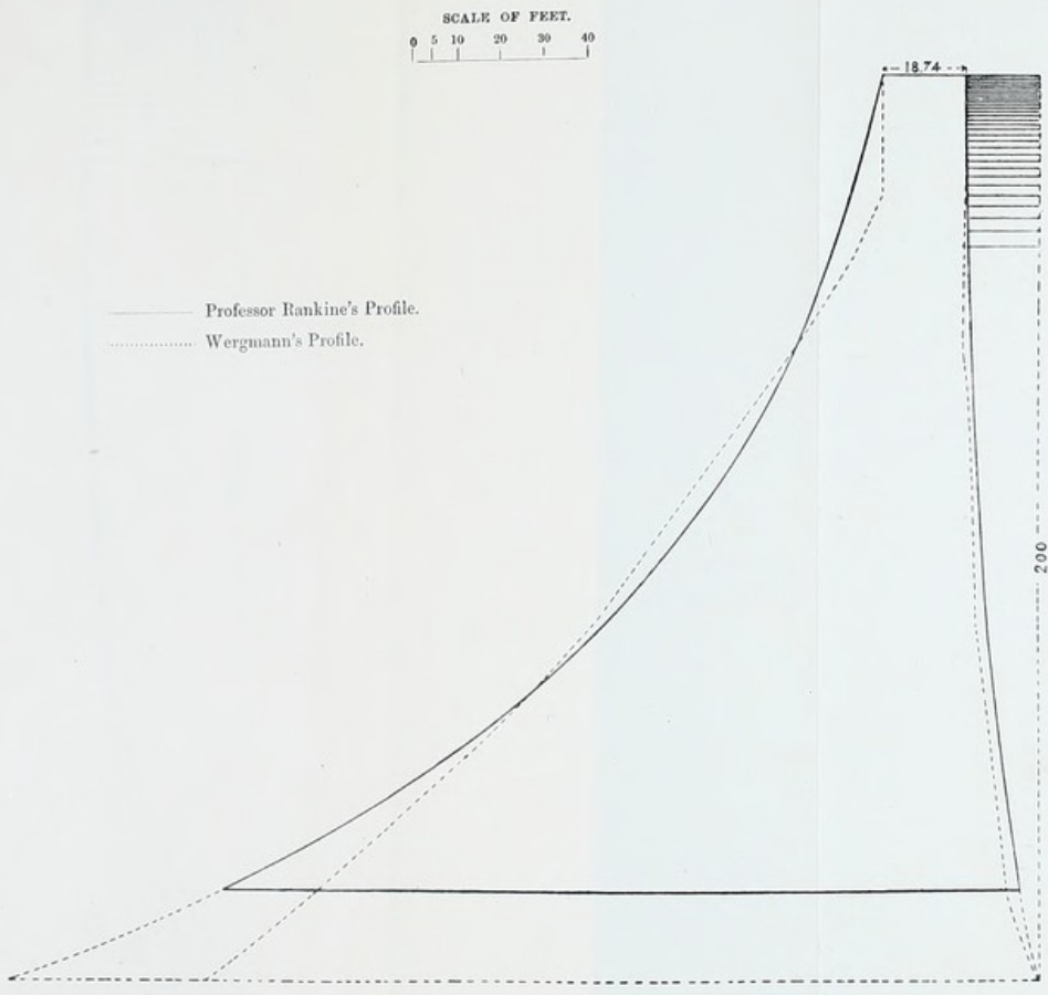
FIG. 49.—MASONRY DAMS: COMPARISON OF RANKINE'S PROFILE WITH THE THEORETICAL PROFILE.
