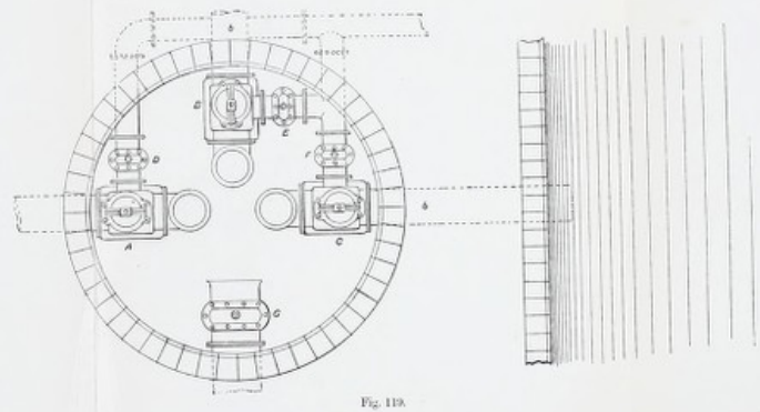
ARRANGEMENT FOR REGULATING SPEED OF FILTERING BEDS (AUTOMATIC).
