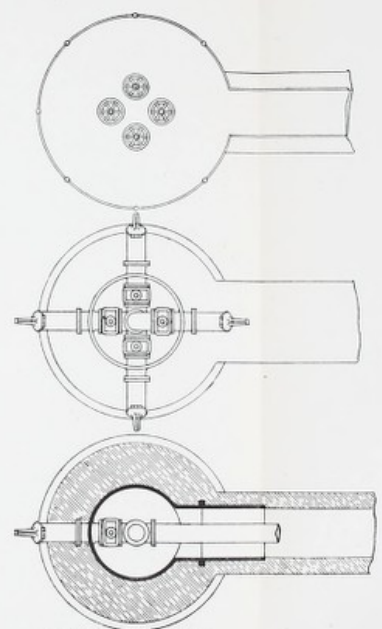
Figs. 41, 42, 43.—Horizontal Sections.
