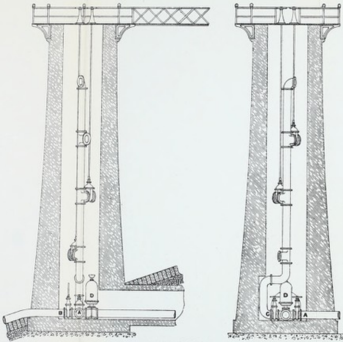
Figs. 30, 31.—Vertical Sections.
