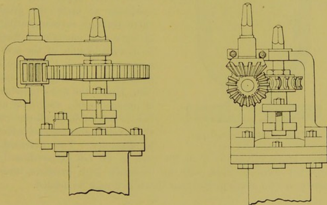
Figs. 237, 238.—Gear for opening sluice valves.
