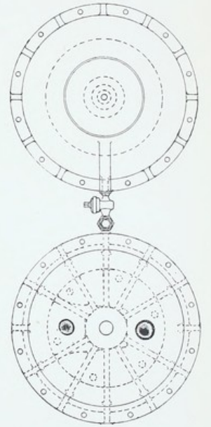
Figs. 37, 38.—Horizontal Sections.
