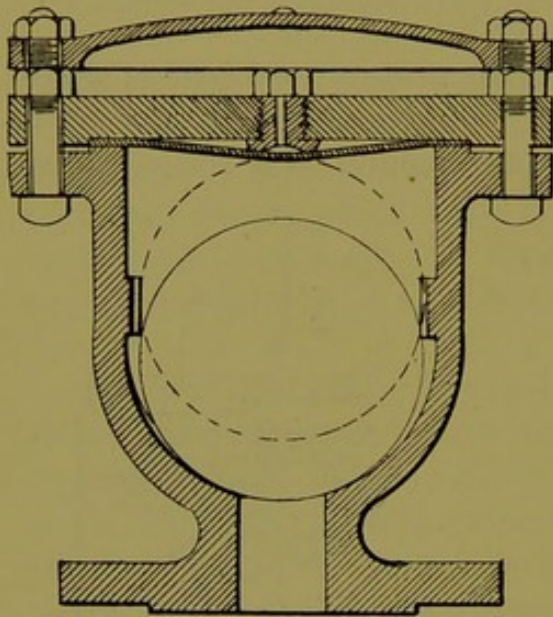
Fig. 239.—Air valve for waterpipe.
