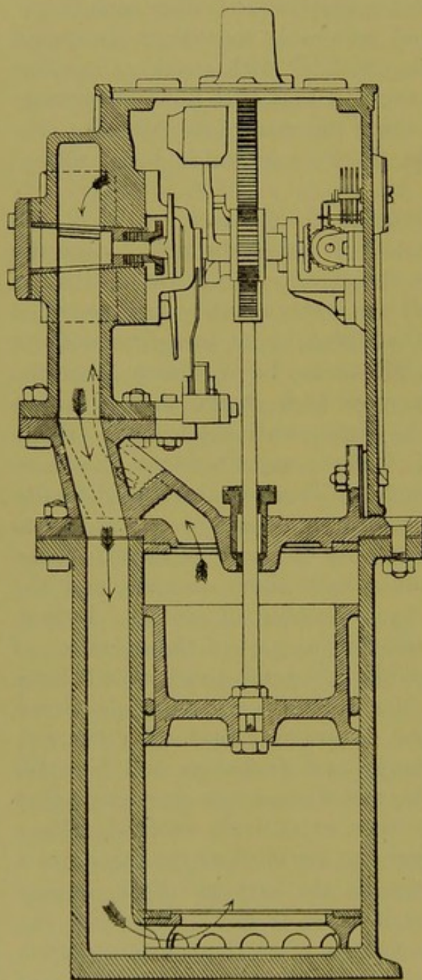
Fig. 232.—Kennedy's patent water meter.
