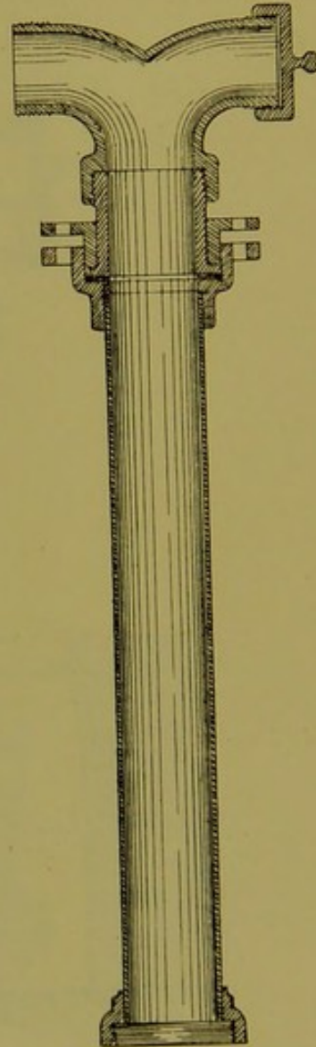
Fig. 193.—Stand-pipe for sluice-valve hydrant.
