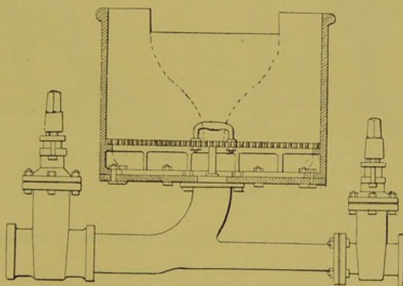
Fig. 122.—Sand-washer.
