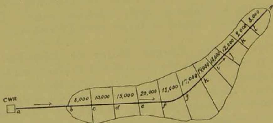
Fig. 179.—Diagram illustrating arrangement of distributing mains.
