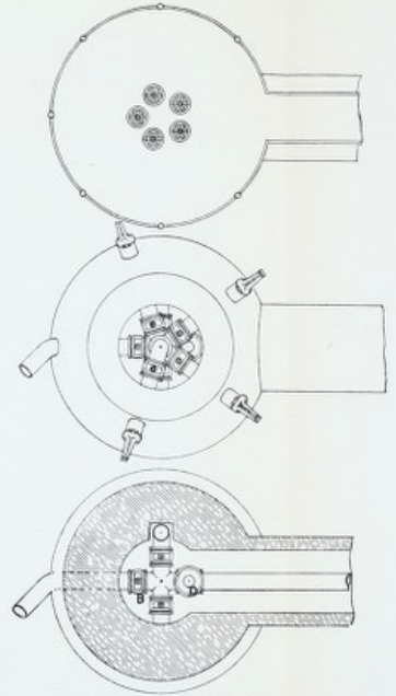
Figs. 32, 33, 34.—Horizontal Sections.
