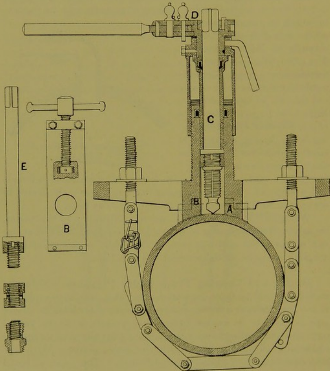
Figs. 250, 251, 252.—Gear for connecting pipes to mains.
