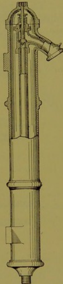
Fig. 244. — Blakeborough's stand pillar.
