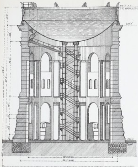
Fig. 143.—Water Tower (in Masonry) at Liverpool.
