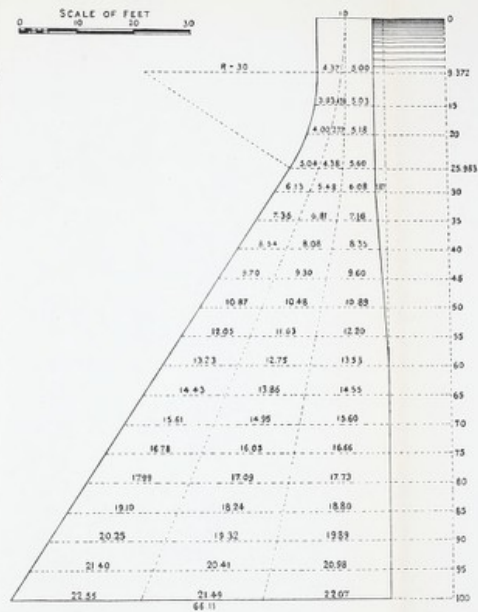
Fig. 52.—Practical Profile No. 2.
