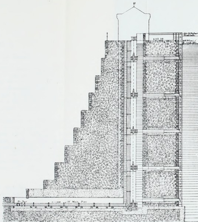
FIG. 56.—TYTAM DAM, HONGKONG : SECTION THROUGH VALVE-WELL.
