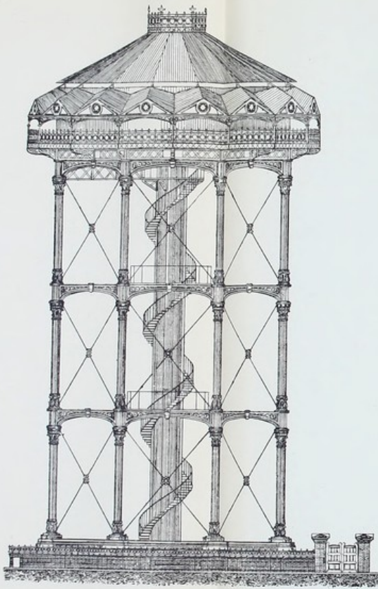
Fig. 144.—Water Tower (in Cast and Wrought Iron) at Shanghai.
