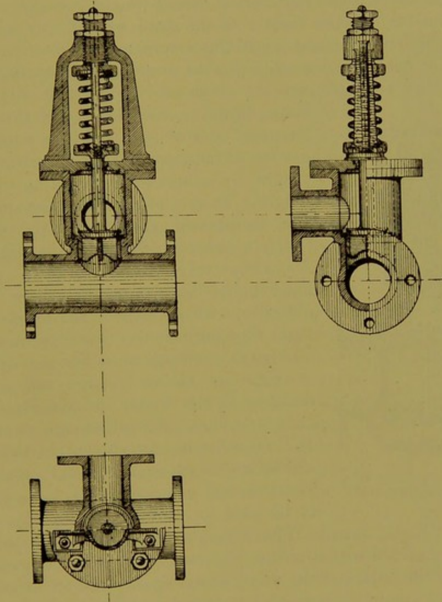
Figs. 240, 241, 242.—Spring and screw-down safety valve. Scale, 1\frac{1}{2} in. to 1 ft.
