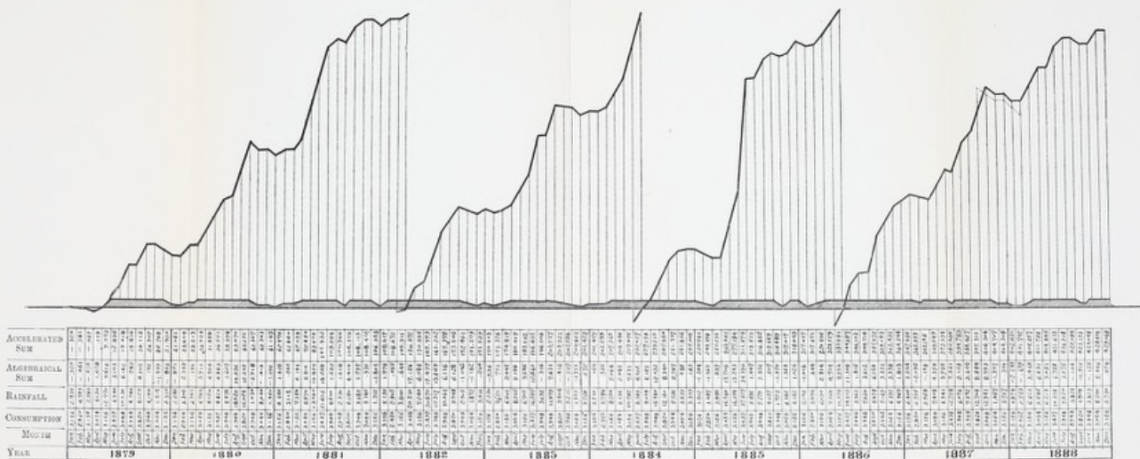
FIG. 5.—DIAGRAM ILLUSTRATING REQUIRED STORAGE CAPACITY (YEARLY RAINFALL).
