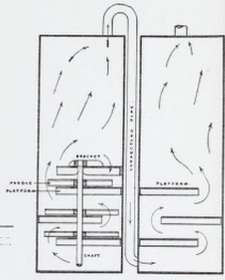
Fig. 133 - Longitudinal Section of Precipitating Tanks.
