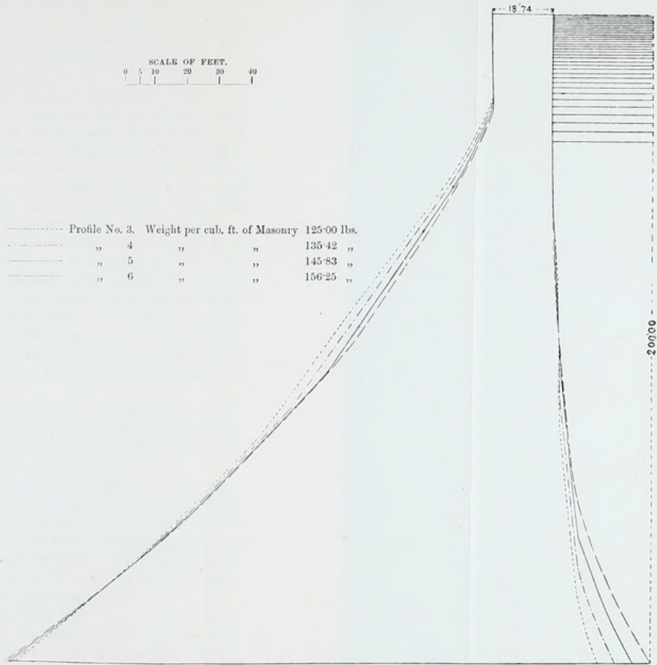
FIG. 50.—MASONRY DAMS: WERGMANN'S THEORETICAL PROFILE FOR STONE OF DIFFERENT GRAVITIES.
