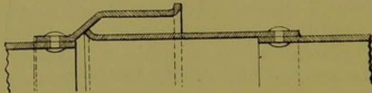
Fig. 220.—The Riley patent joint for water-pipes.
