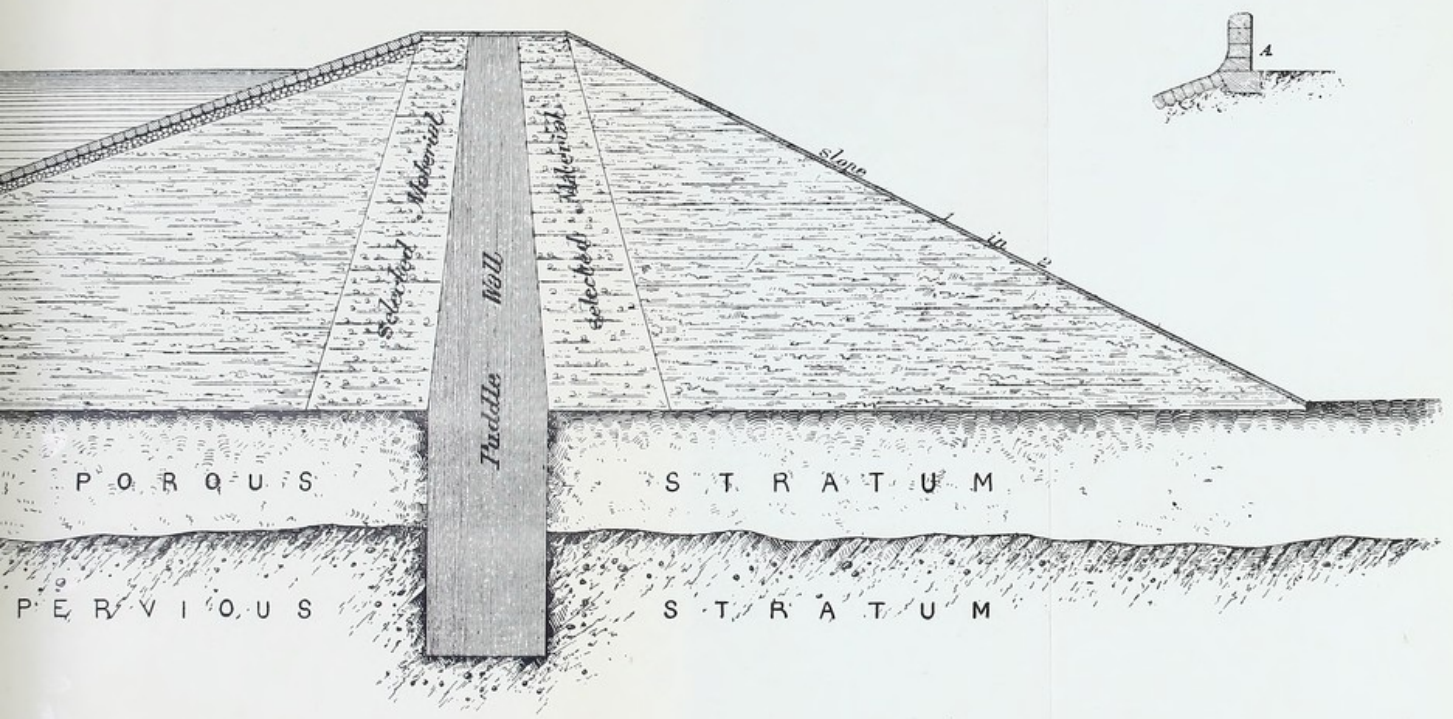
FIG. 18.—SECTION OF EARTHWORK DAM.
