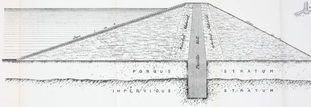
FIG. 18.—SECTION OF EARTHWORK DAM
