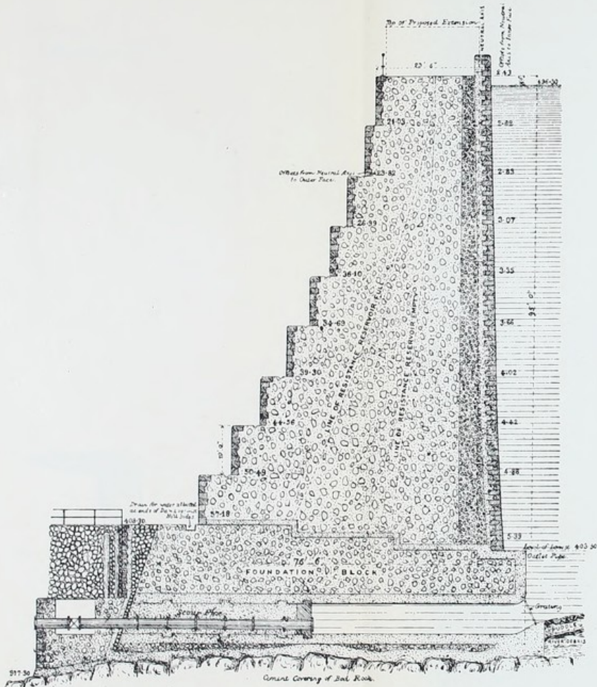
FIG. 54.—TYTAM DAM, HONGKONG: SECTION THROUGH SCOUR PIPE.
