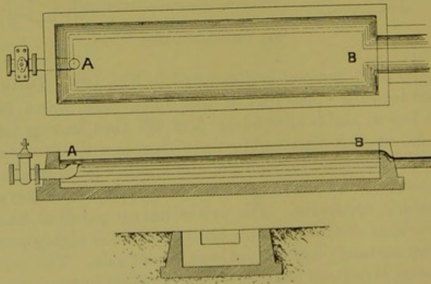
Figs. 125, 126 and 127.—"Canal" sand-washer (in plan and sections).
