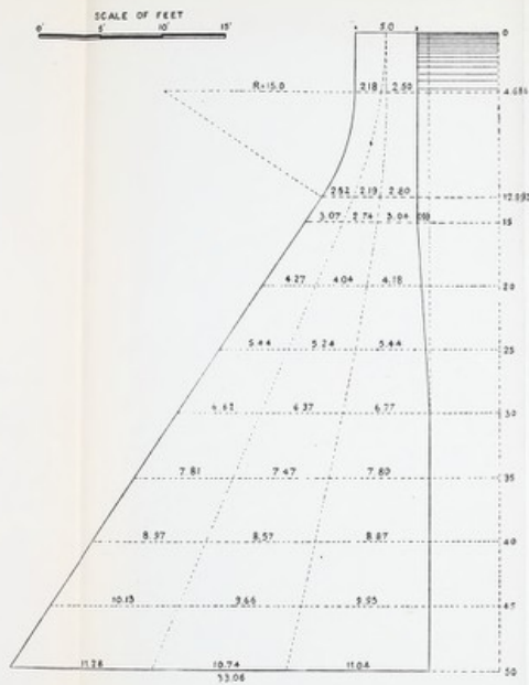
Fig. 51.—Practical Profile No. 1.
