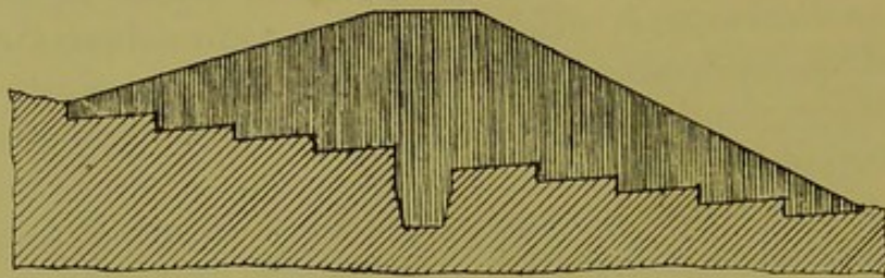
Fig. 48.—Site of dam trenched-out.
