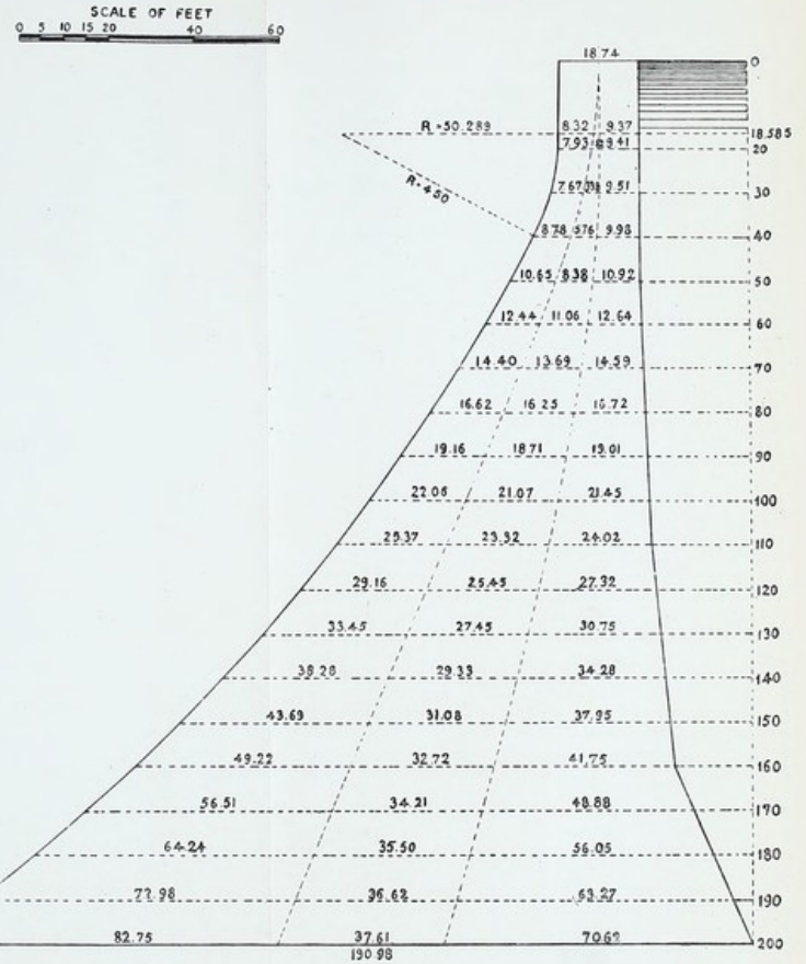
Fig. 53.—Practical Profile No. 3.
