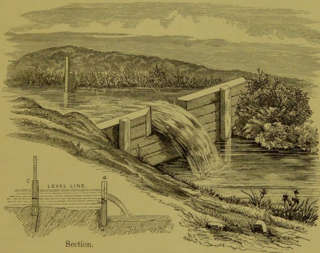
Figs. 1 and 2.—Weir or notchboard for gauging streams.
