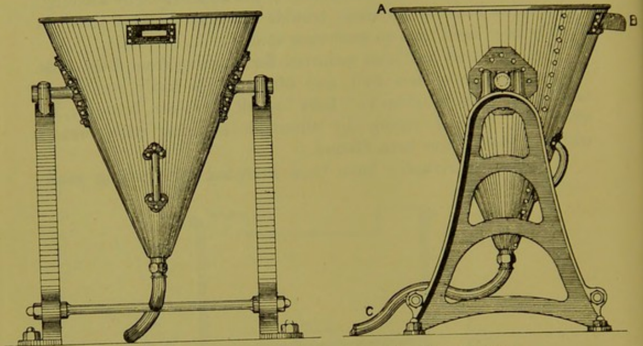
Figs. 123 and 124.—Walker's patent sand-washing apparatus.
