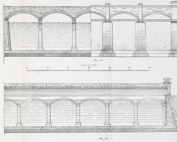
COVERED RESERVOIR: BRICK OR CONCRETE ARCHES OF COLUMNS
