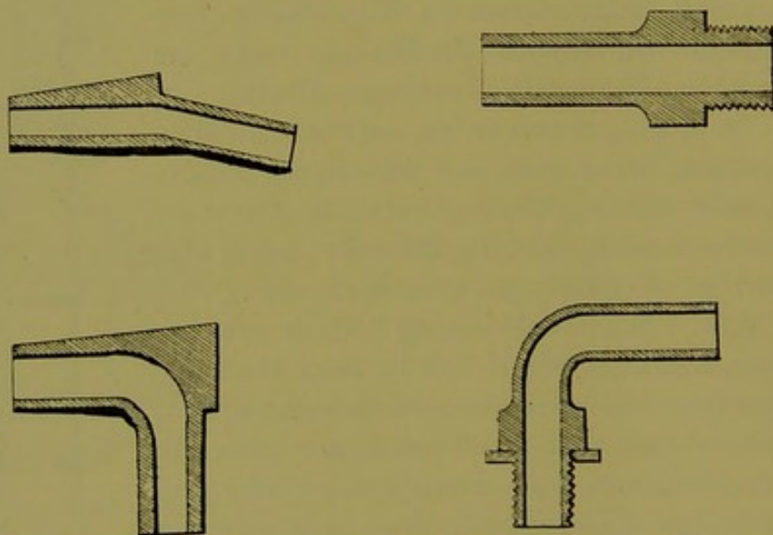
Figs. 247, 248.—Screwed ferrules for connecting waterpipes.
