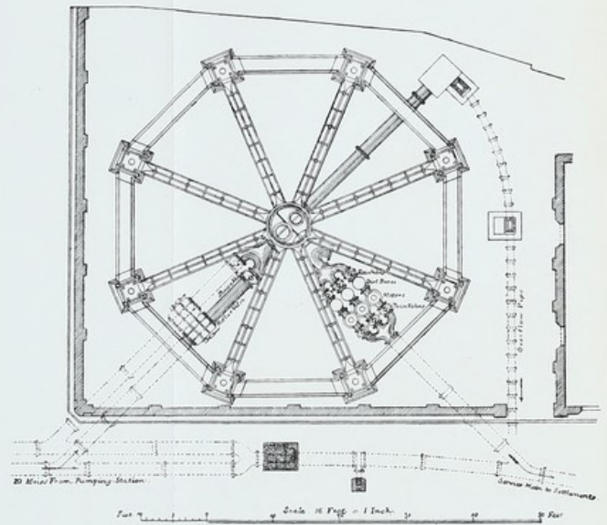
Fig. 145.—Ground Plan of Water Tower at Shanghai.
