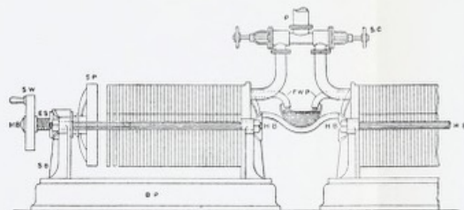
Fig. 136 - Filter-press.
