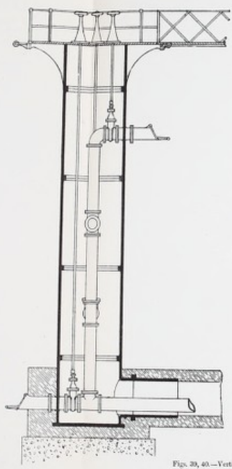
Figs. 39, 40.—Vertical Sections.
