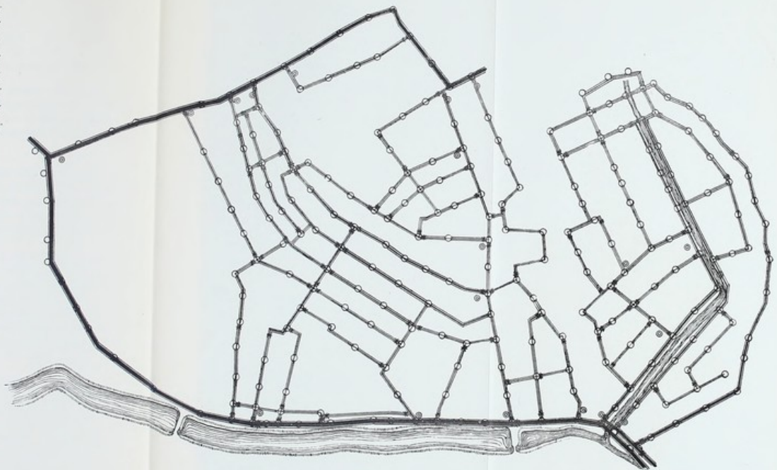
FIG. 185.—WATERWORKS OF TOKYO: PART OF DISTRIBUTION SYSTEM IN DETAIL.
