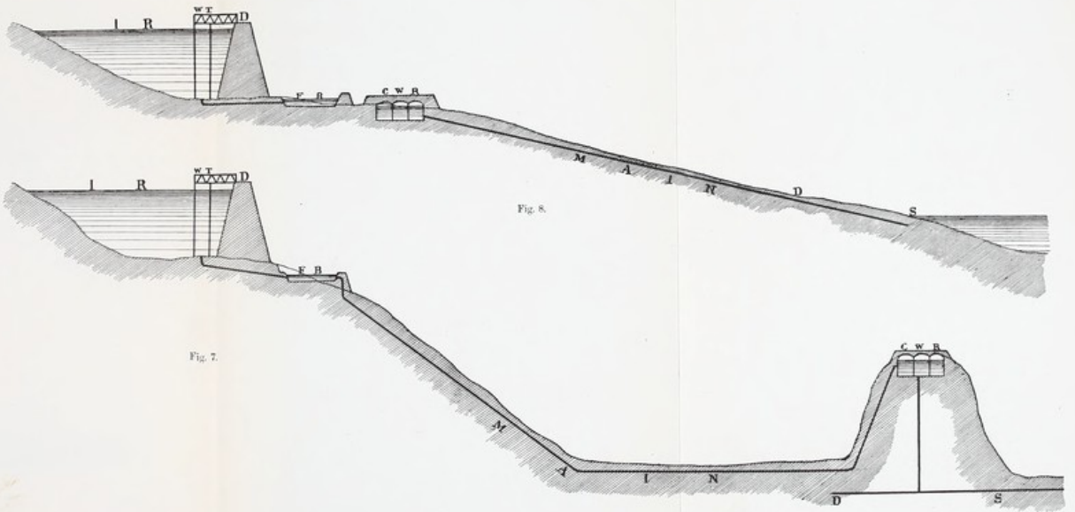
DIAGRAMS ILLUSTRATING GRAVITATION SYSTEMS OF WATERWORKS.
