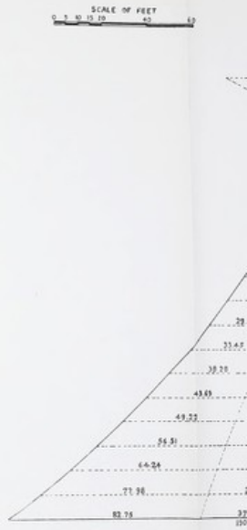
Fig. 53.—Practical Profile No. 3.
