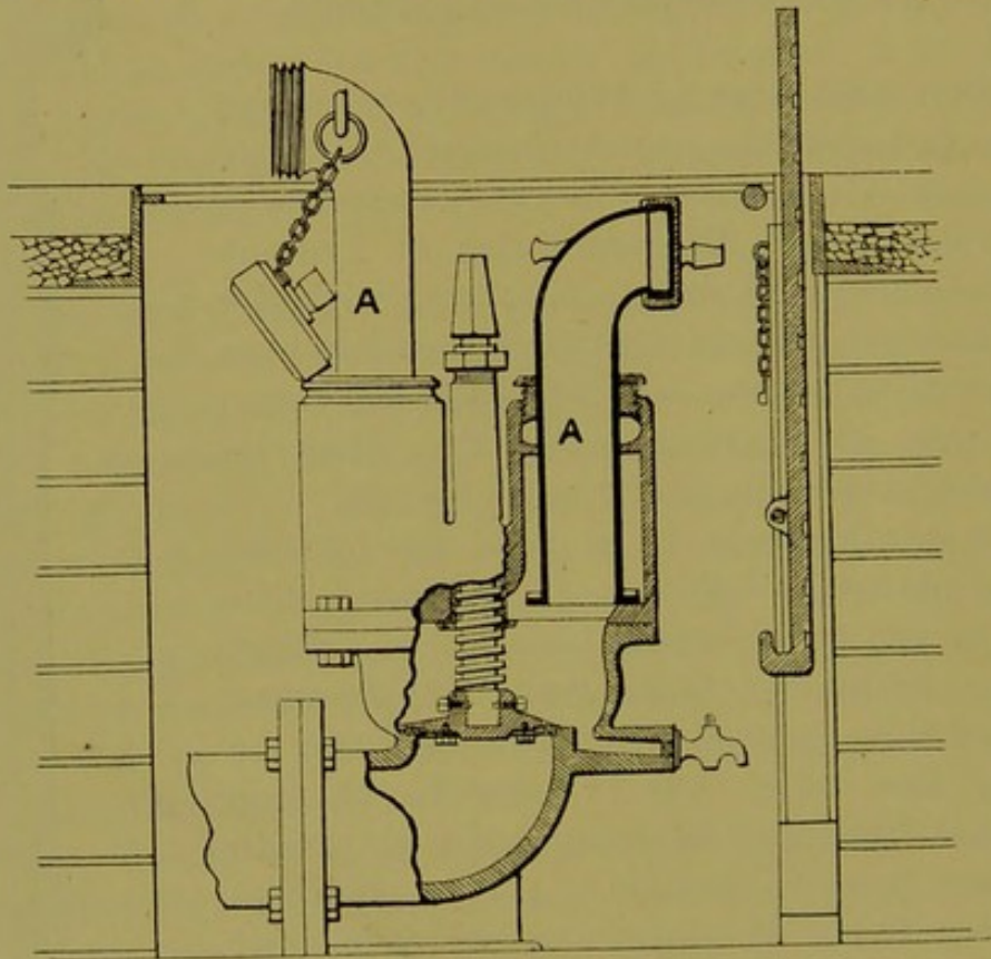
Fig. 189.—Merryweather's hydrant.
