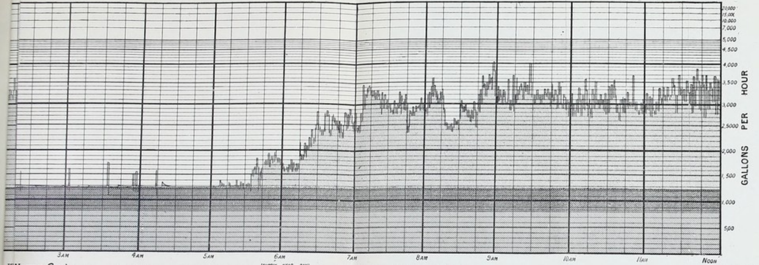
WATER CO.) Fine Diagram Sep 1881 before application of WWM system Thick Diagram Nov 1881, after application of WWM system SAVING 36.1
