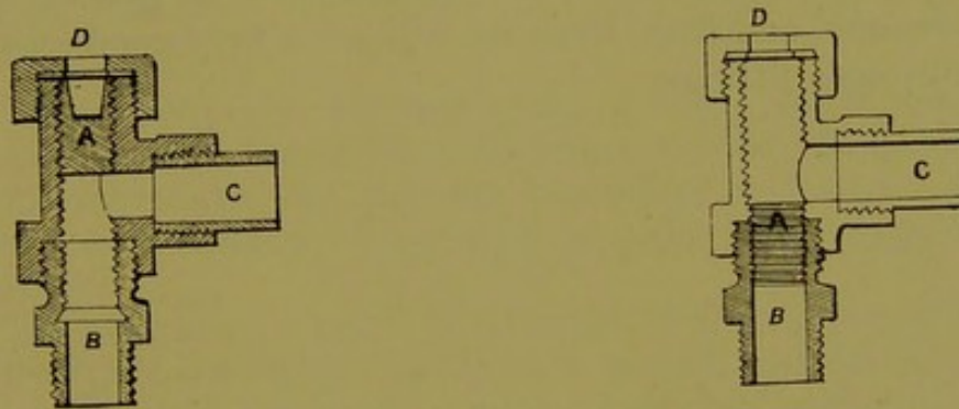
Figs. 253, 254.—Patent stop-valve ferrule.
