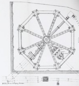
Fig. 145.—Ground Plan of Water Tower at Shanghai.
