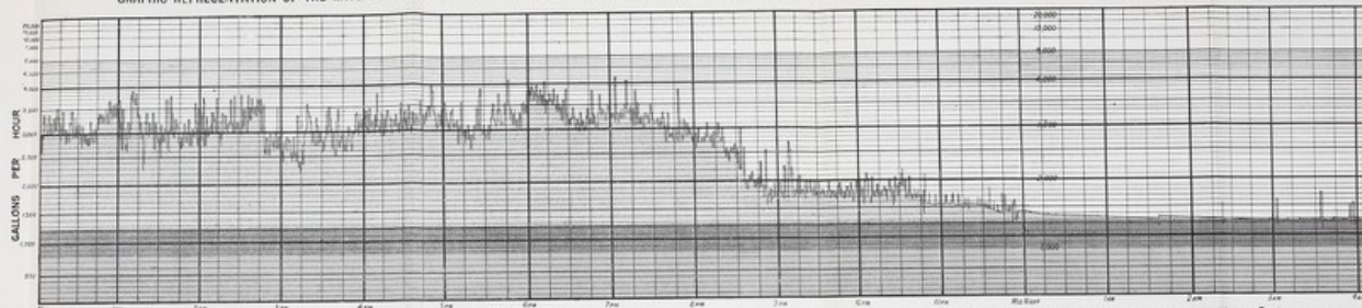
Fig. 228 LIVERPOOL Example of Waste Water Meter Diagrams From a District of 2,500 Persons
