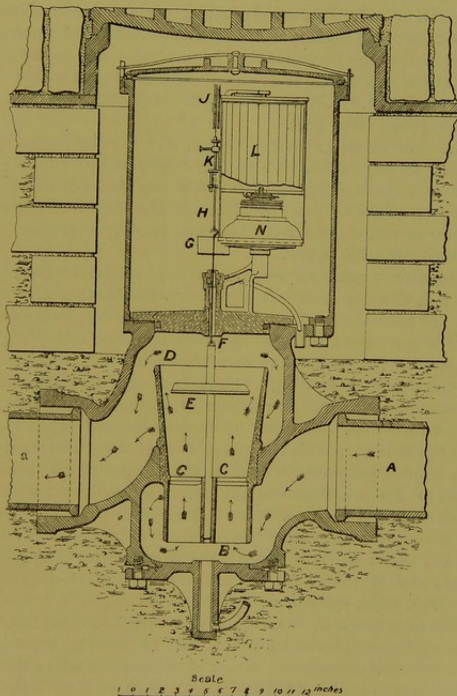
Fig. 223.—Mr. G. F. Deacon's "District" water meter.
