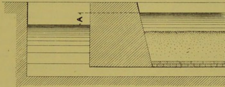
Fig. 101.—Diagram illustrating the filtering head.
