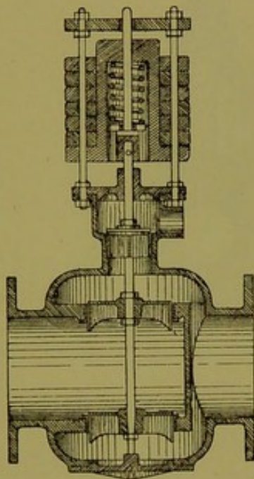
Fig. 243.—Large safety valve for use on water mains.
