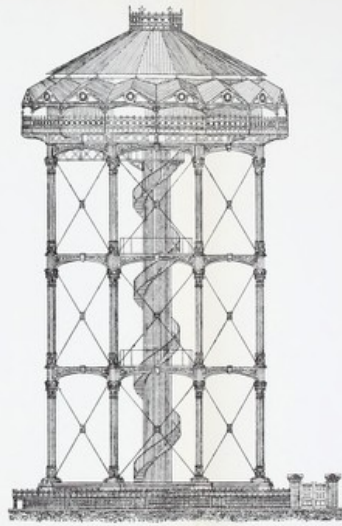
Fig. 144.—Water Tower (in Cut and Wrought Iron) at Shanghai.
