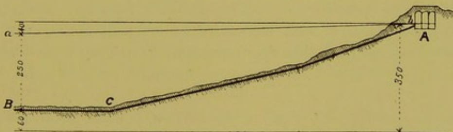
Fig. 174.—Diagram illustrating calculation of hydraulic grade line.
