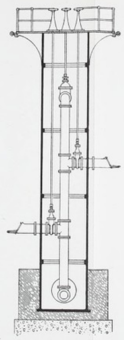
Figs. 39, 40.—Vertical Sections.
