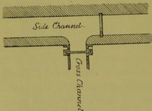
Fig. 58.—Side and cross channels of settling tanks.
