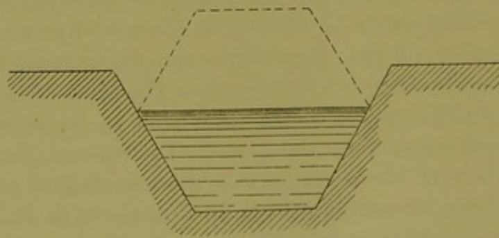
Fig. 149.—Section of open channel of semi-hexagonal form.
