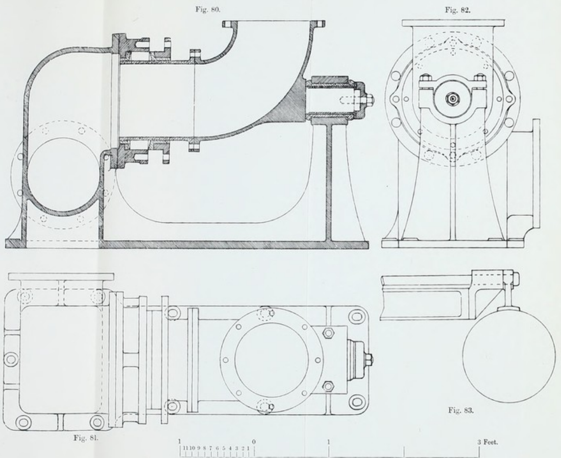
SETTLING RESERVOIRS: DETAILS OF FLOATING PIPE.
