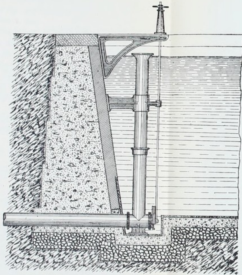
FIG. 84.—OVERFLOW AND DRAIN PIPE COMBINED.
