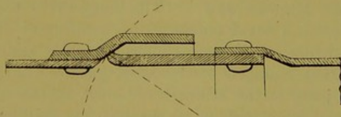
Fig. 219.—The Duncan patent joint for water-pipes.
