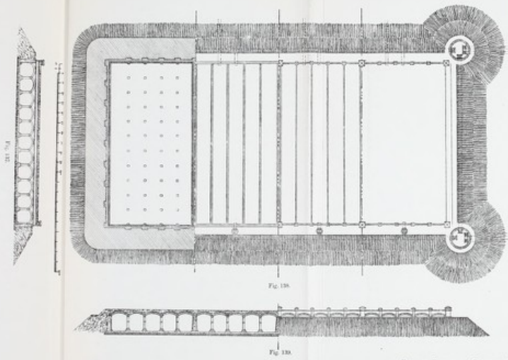
COVERED RESERVOIR: BRICK OR CONCRETE ARCHES OF COLUMNS
