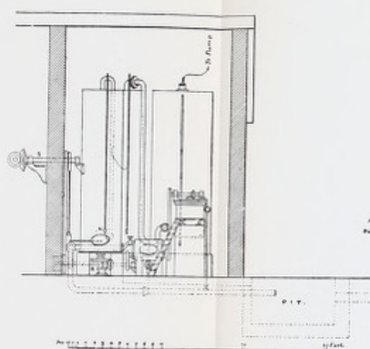
Fig. 132 - Side Elevation.
