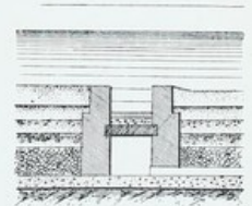
Fig. 105.—Section across the Gathering Drain.
