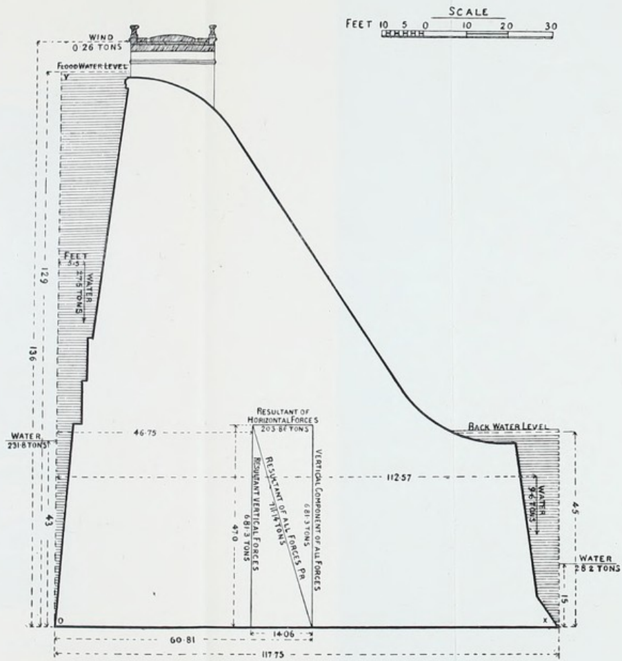
FIG. 55.—SECTION OF VYRNWY DAM (LIVERPOOL WATER SUPPLY).
