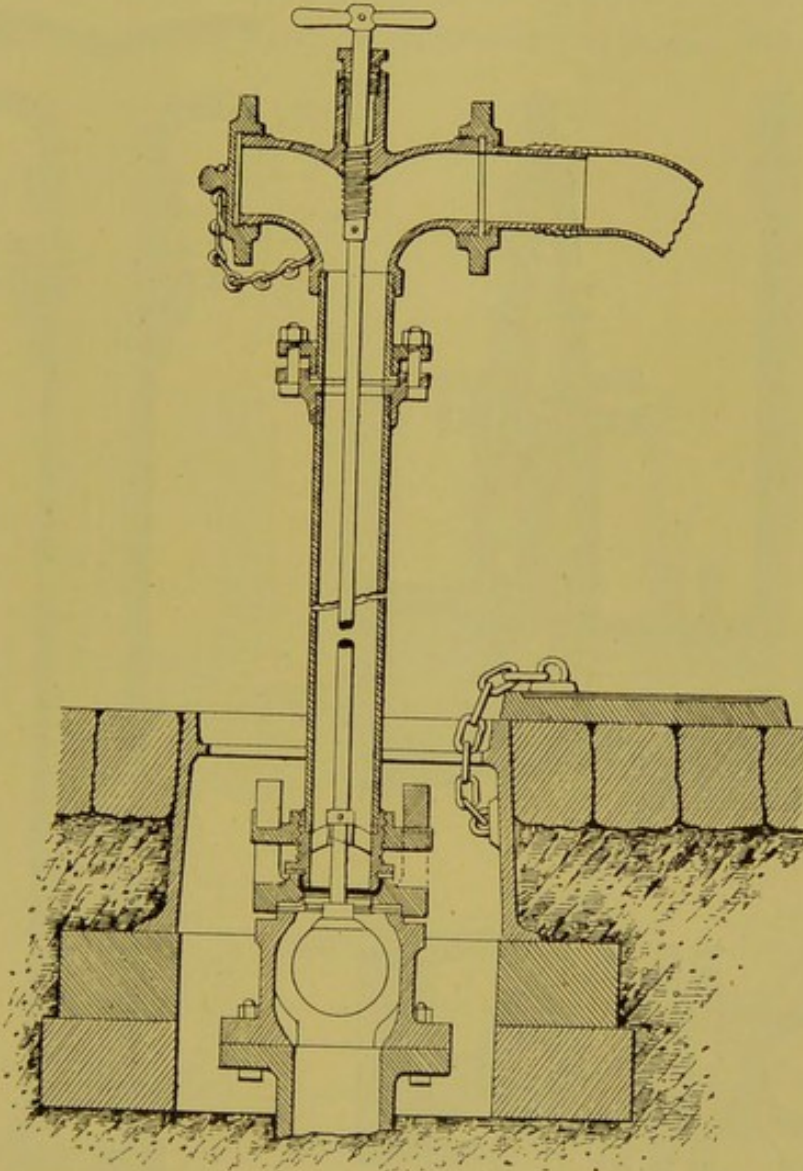
Fig. 190.—Ball hydrant and stand-pipe.
