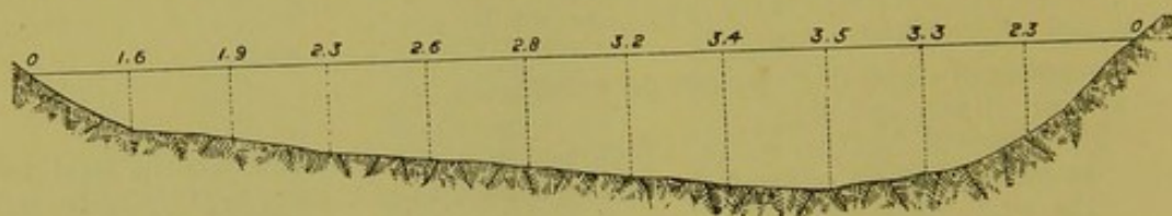
Fig. 4.—Section across river showing depth of stream at various points.
