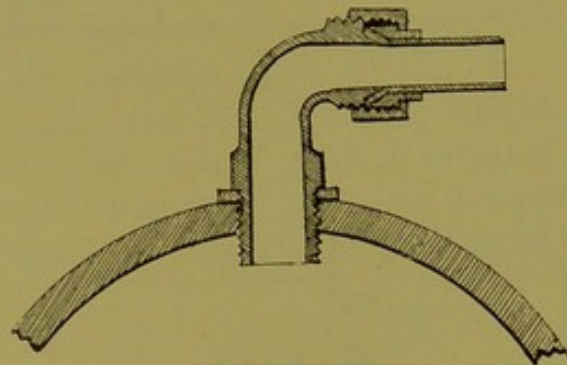
Fig. 249.—Screwed ferrule attached to waterpipe.
