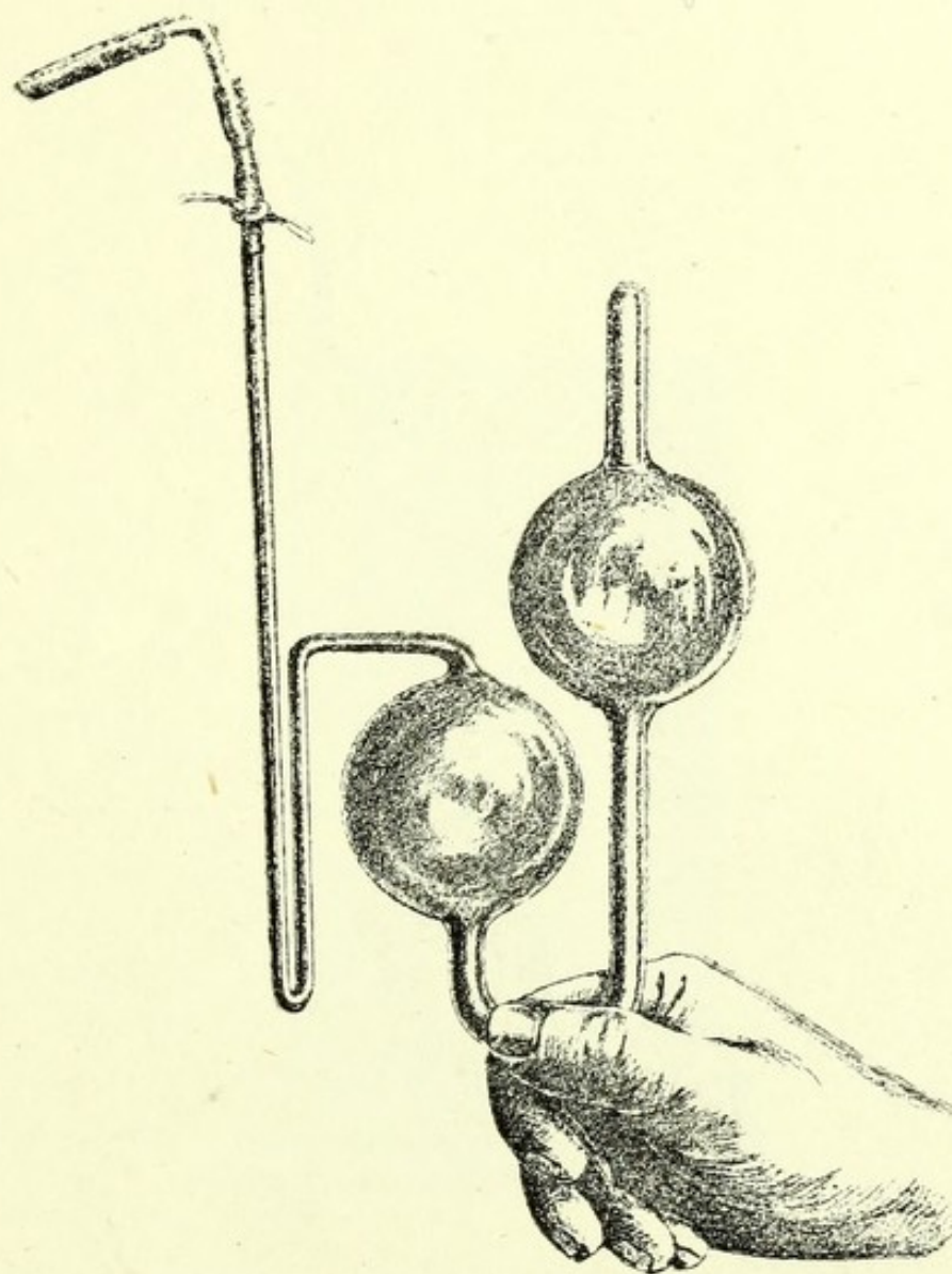
THE ABSORPTION-PIPETTE.
