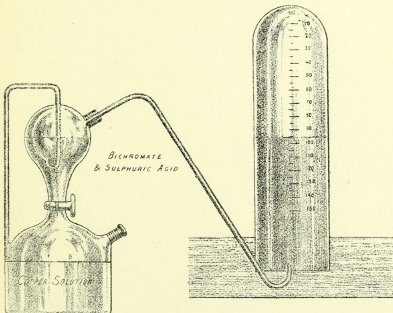
RECOVERY OF CARBONIC OXIDE GAS.
