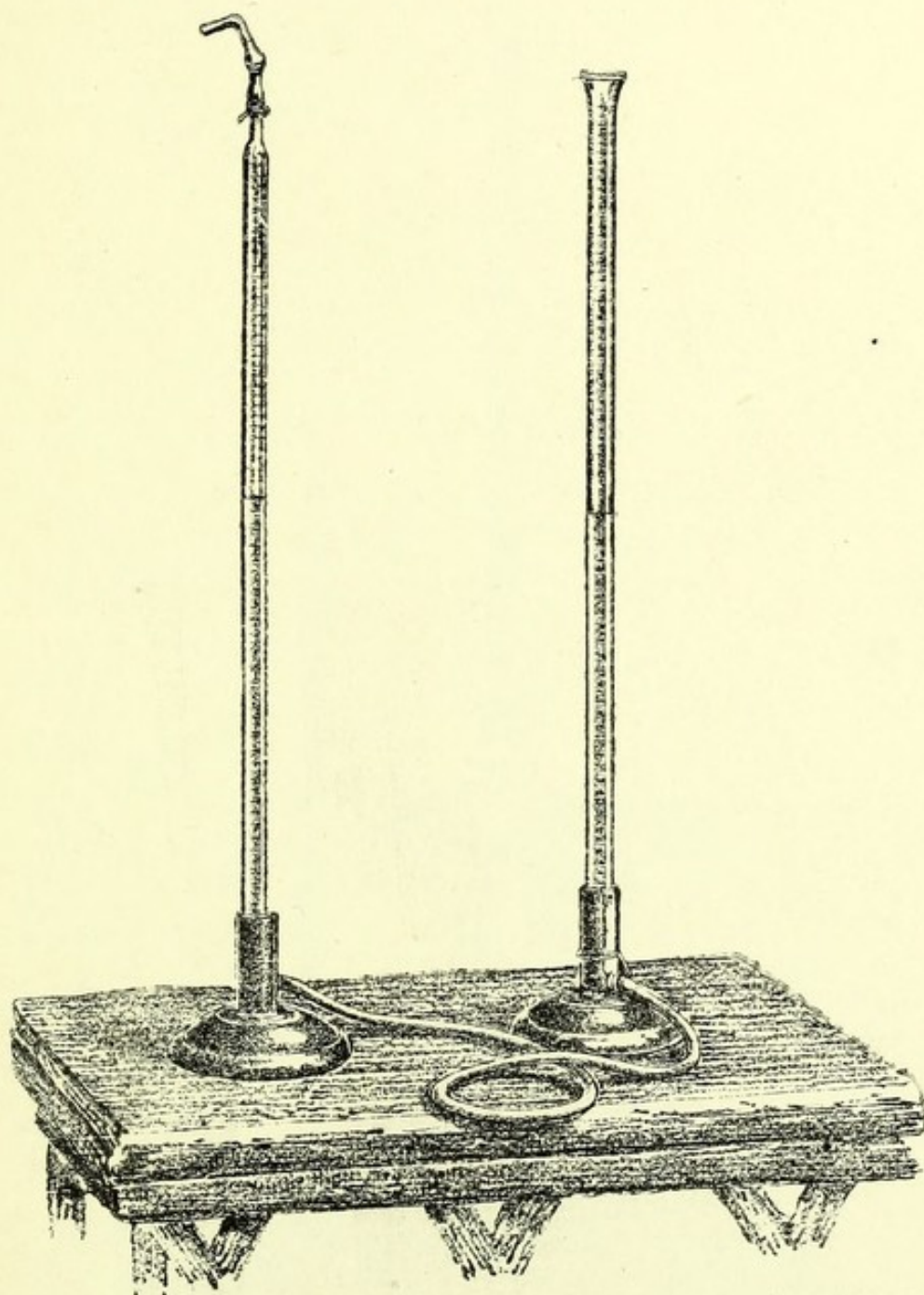
HEMPEL'S GAS-BURETTE, READY FOR USE.
