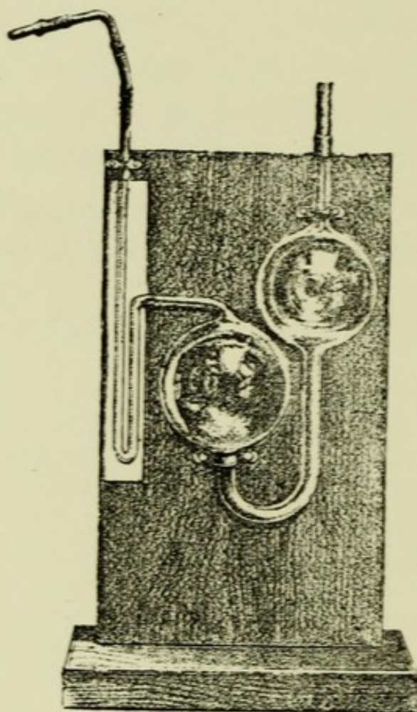
ABSORPTION-PIPETTE CHARGED WITH POTASH.
