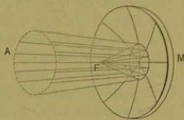
Real focus of convergent rays from a concave mirror.
