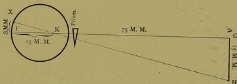
Deviation produced by prism.
