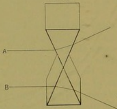
Passage of two parallel rays through two prisms placed apex to apex, causing a divergence.
