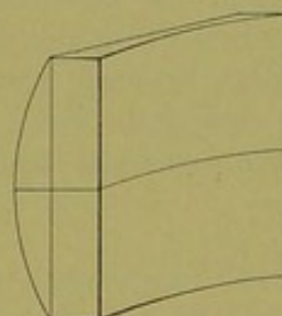
Crossed cylindrical lens.
