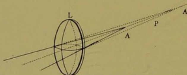
Negative focus from a bi-convex spherical lens.
