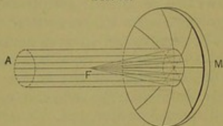
Formation of principal focus from a concave mirror.
