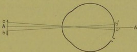
Principal and secondary axes.
