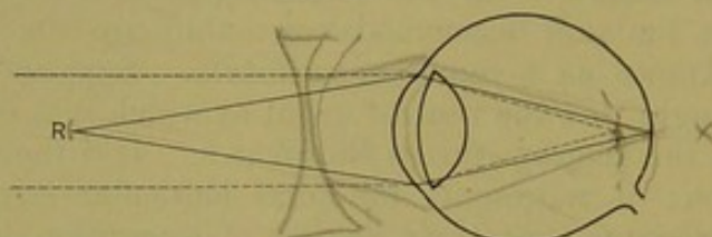
Far-point in a myopic eye.
