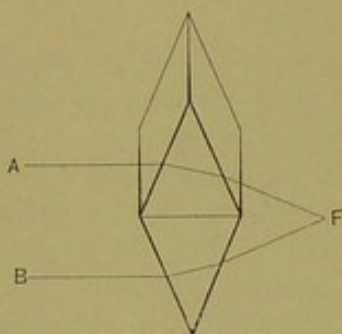
Passage of parallel rays through two prisms placed base to base, forming a focus.
