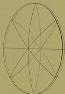
Bi-convex spherical lens.
