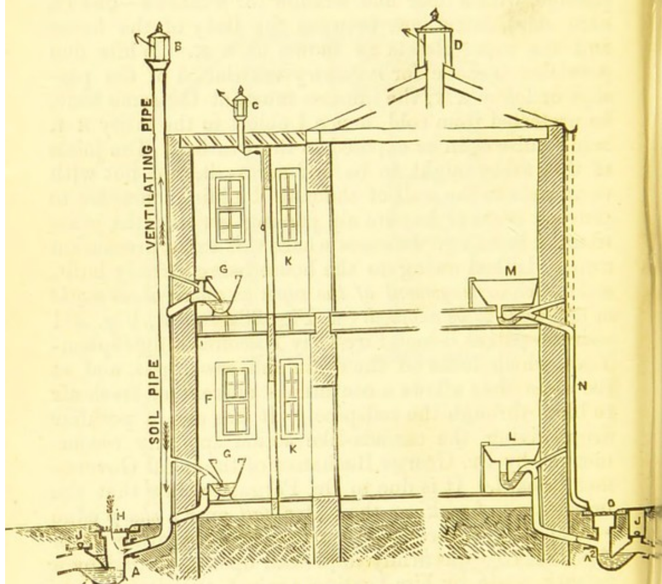
Fig. 282.—Elevation.
