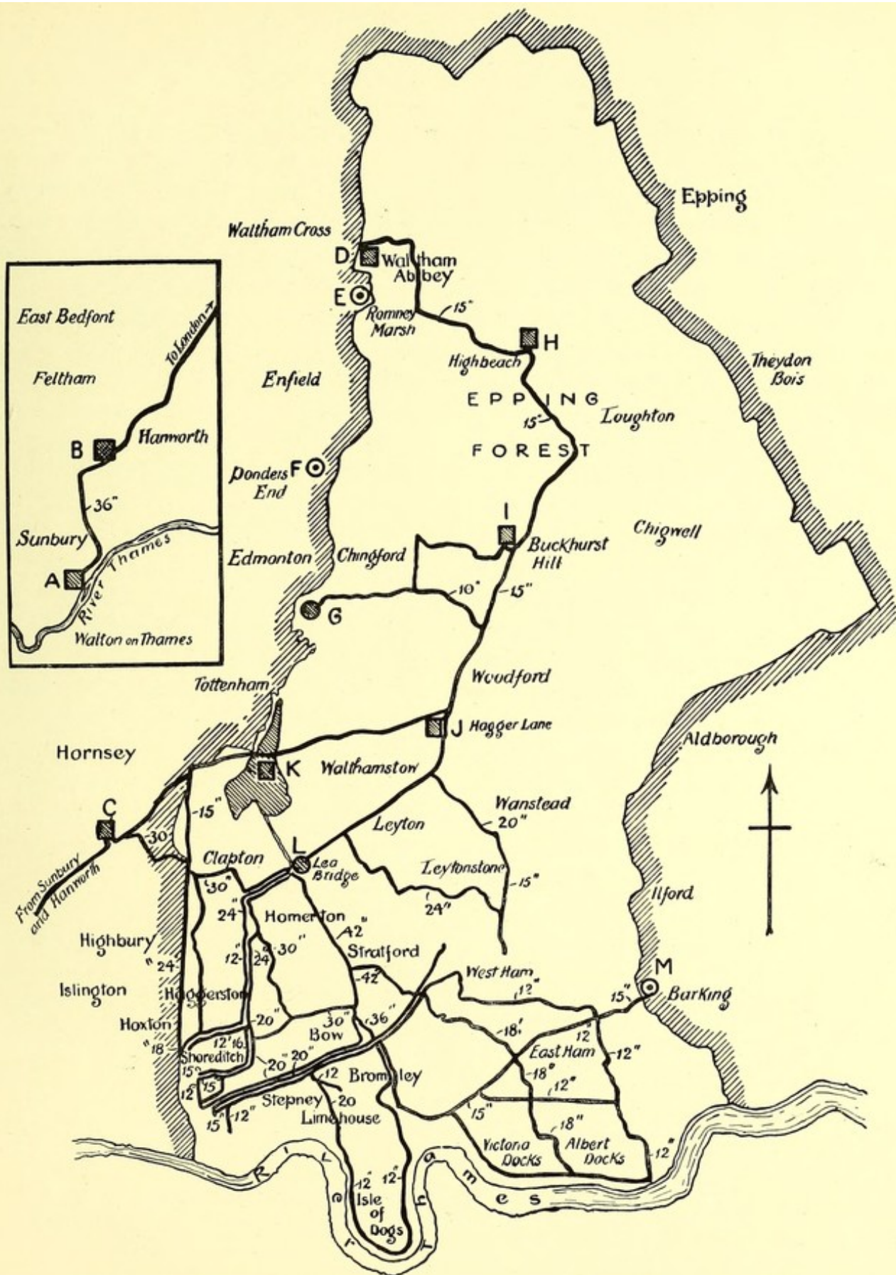
FIG. 16.—THE EAST LONDON WATERWORKS COMPANY'S WORKS.
