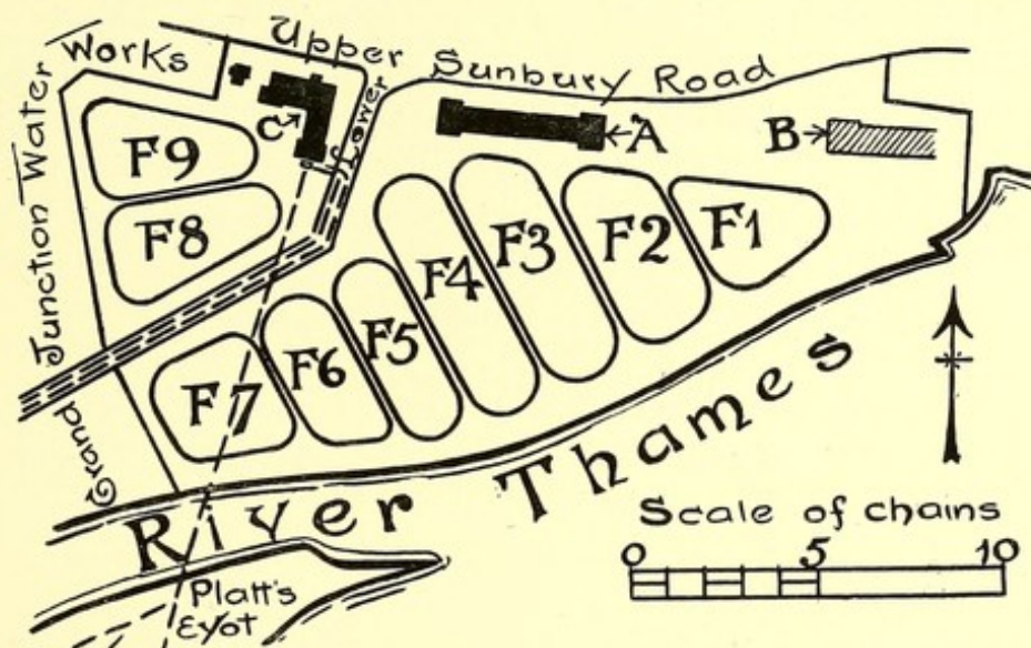
FIG. 41.—HAMPTON STATION.
