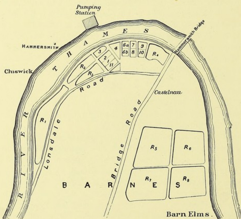
FIG. 23.—THE RESERVOIRS AND FILTER-BEDS AT BARNES.
