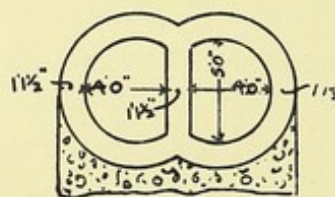
FIG. 19.—THE DIAGRAM SHOWS A SECTION OF THE HIGH LEVEL CULVERTS. THESE ARE BUILT OF BRICK AND BEDDED IN CONCRETE.
