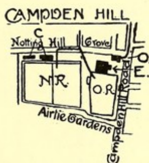
FIG. 30.—CAMPDEN HILL STATION.
