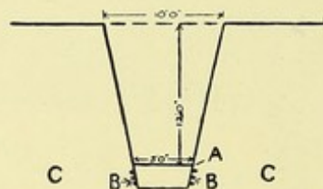
FIG. 26.—SECTION OF FILTER-TRENCH.
