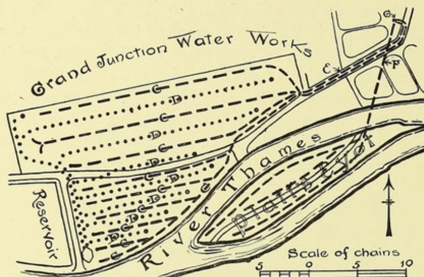
FIG. 36.—PLAN SHOWING ARRANGEMENT OF THE DISTRIBUTING AND COLLECTING PIPES IN THE HAMPTON GRAVEL-BEDS.
