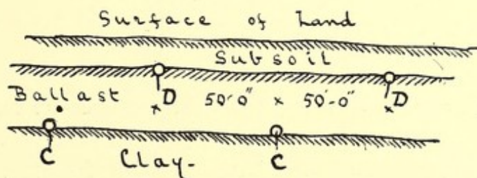
FIG. 39.—VERTICAL SECTION SHOWING THE ARRANGEMENT OF DISTRIBUTING PIPES (D) AND COLLECTING PIPES (C) IN THE HAMPTON GRAVEL-BEDS.
