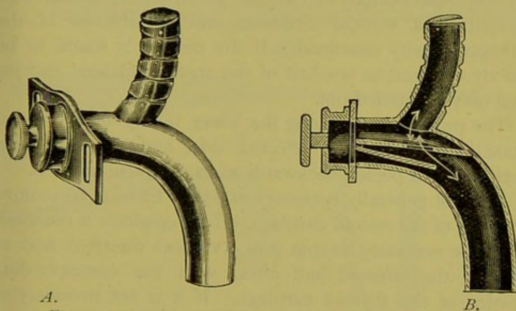
FIG. 158.—Excision of the larynx : Gussenbauer's artificial larynx.
