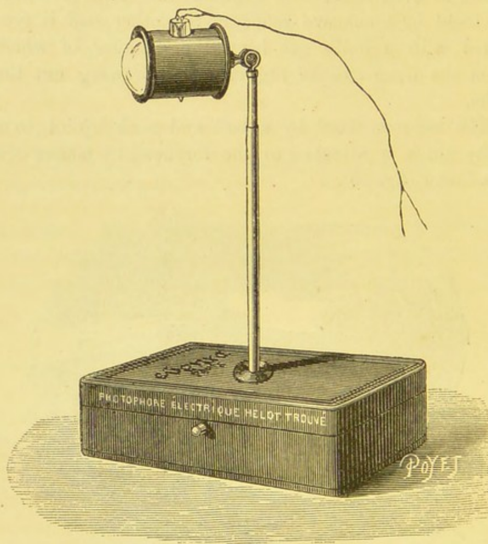
FIG. 21.—THE PHOTOPHORE USED AS A STANDARD LAMP.
