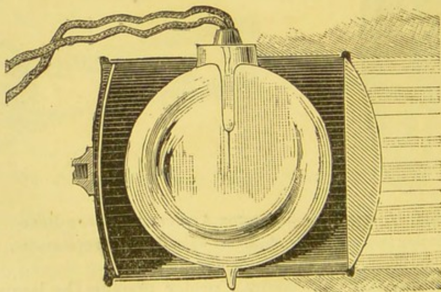
FIG. 19.—TROUVÉ'S ELECTRIC PHOTOPHORE (Longitudinal Section).
