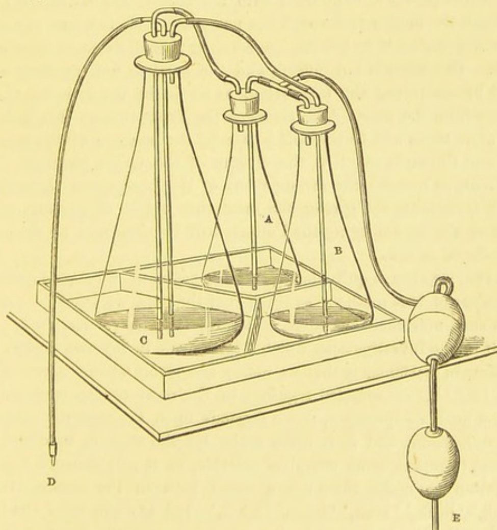
A, Bottle containing hydrochloric acid ; B, Bottle containing liquor ammonia (B.P.) ; C, Large bottle containing water ; D, India-rubber tubing with tip for catheter ; E, Handbag to expel vapours into large bottle where combination takes place.
