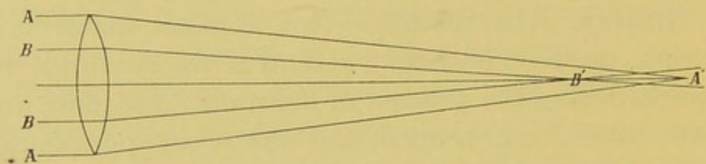
FIG. 40.—NEGATIVE ABERRATION.
