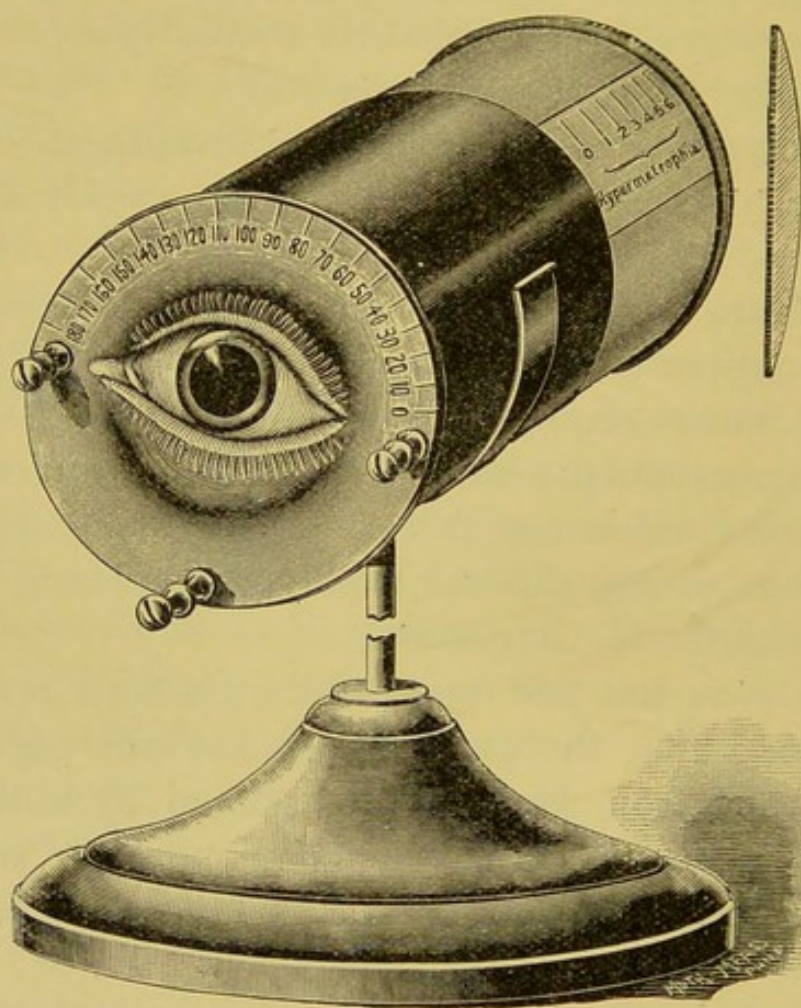
FIG. 1.—THE AUTHOR'S SCHEMATIC EYE FOR STUDYING RETINOSCOPY. (For description, see chap. vi.)
