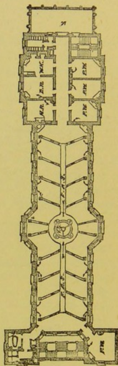
FIGURE 61.—SECOND STORY PLAN OF "ONE" MEDICAL PAVILION OF THE COOK COUNTY HOSPITAL, IN CHICAGO, ILL.
