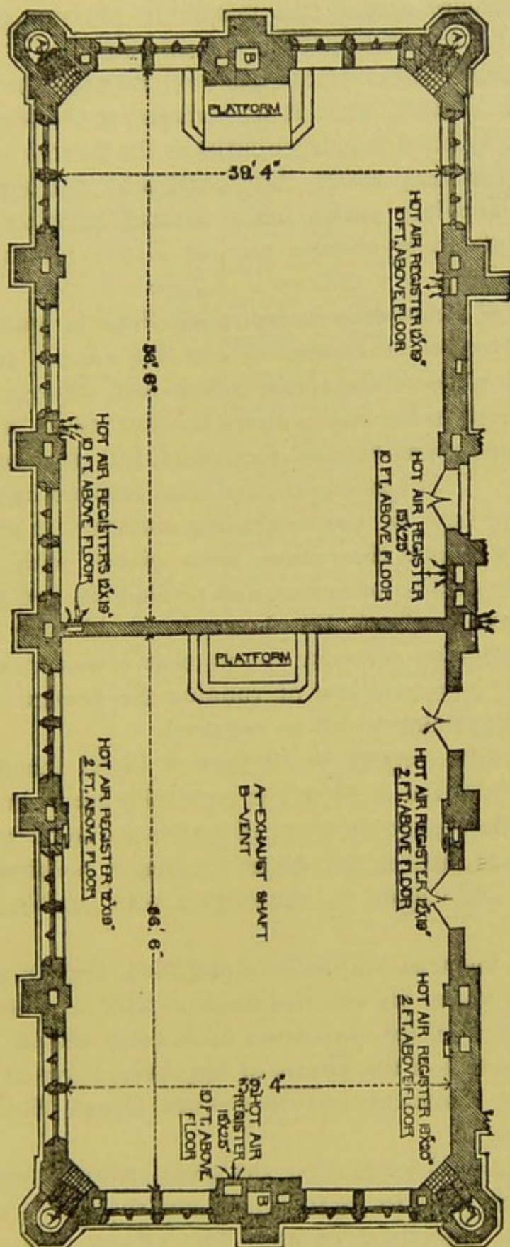
FIGURE 63.—PLAN OF LECTURE ROOM, SHOWING VENTILATING SYSTEM.
