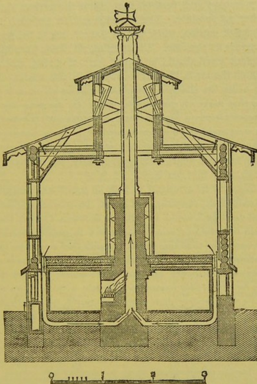
FIGURE 54.—CROSS SECTION, ST. PETERSBURGH CITY HOSPITAL.
