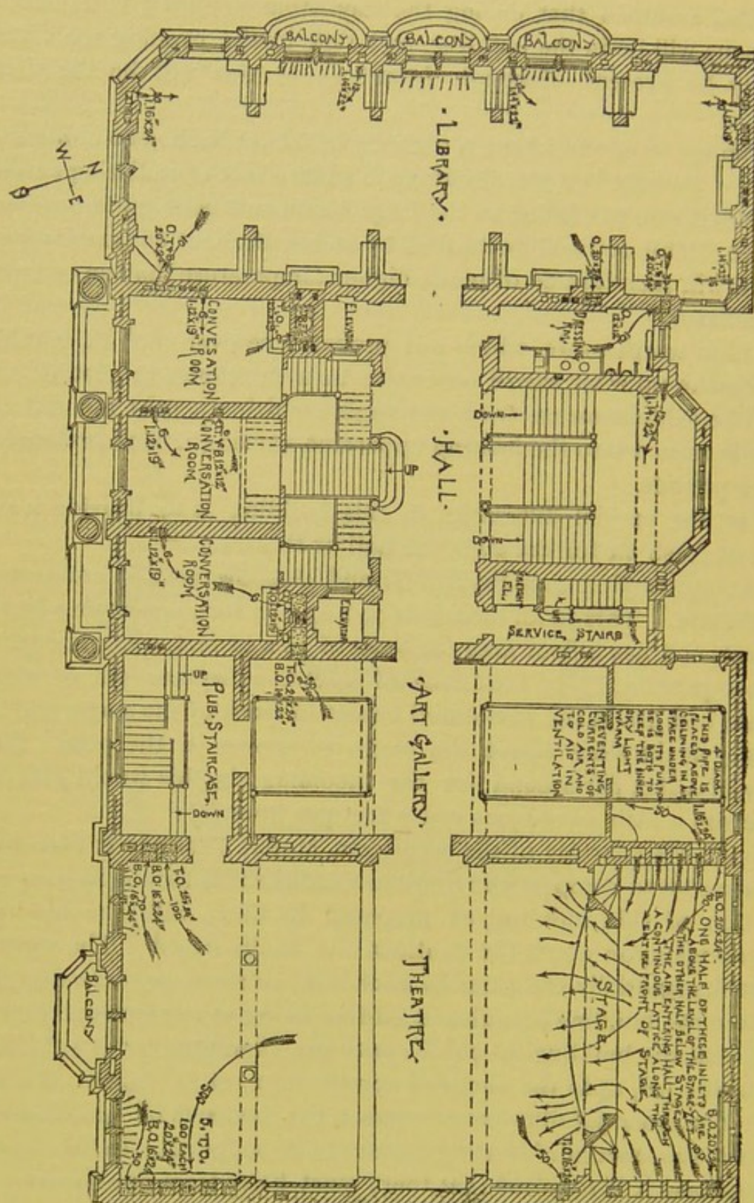
FIGURE 47.—SECOND FLOOR PLAN, UNION LEAGUE CLUB, AS HEATED AND VENTILATED BY F. TUDOR & CO.—PEABODY & STEARNS, ARCHITECTS.
