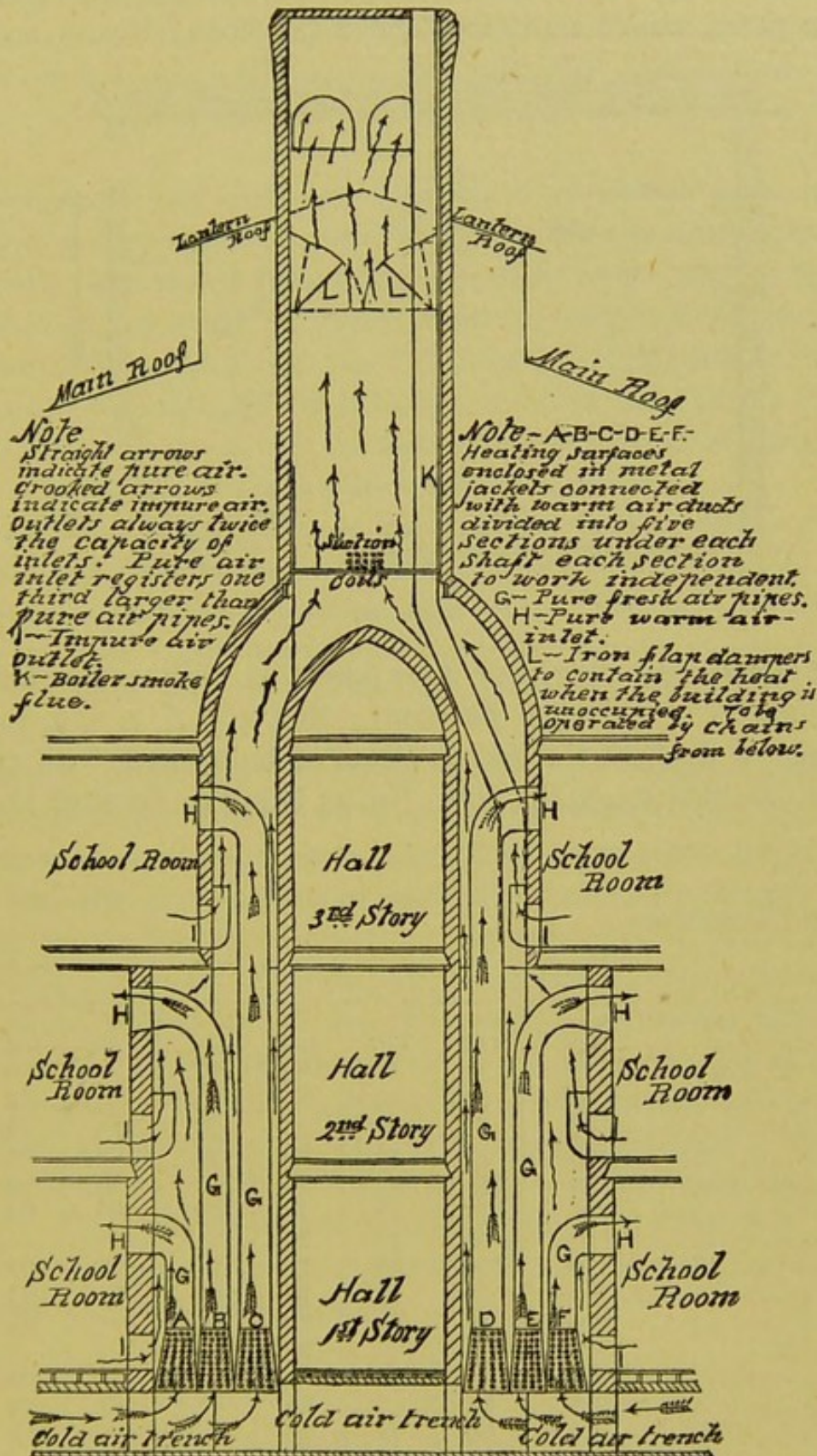
FIGURE 50.—VERTICAL SECTION OF SCHOOL BUILDING.
