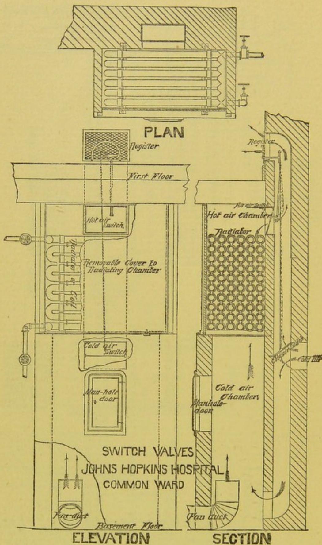
FIGURE 69.—HEATING COILS AND SWITCH VALVES.—JOHNS HOPKINS HOSPITAL.
