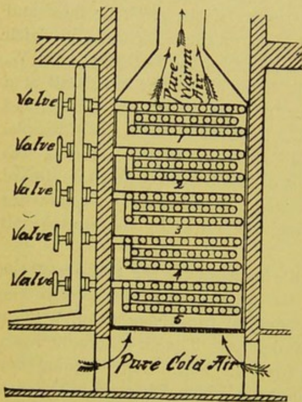
FIGURE 49.—VERTICAL SECTION OF COIL CHAMBER.
