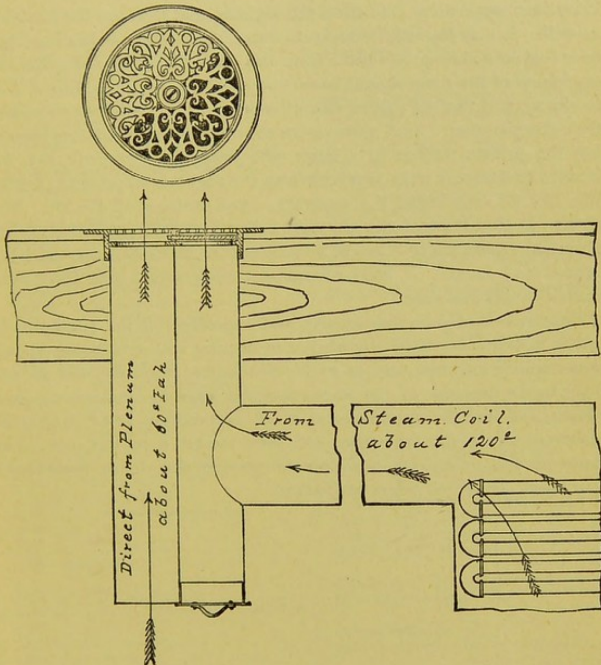
FIGURE 72.—PLAN AND SECTION OF MIXING REGISTER.
