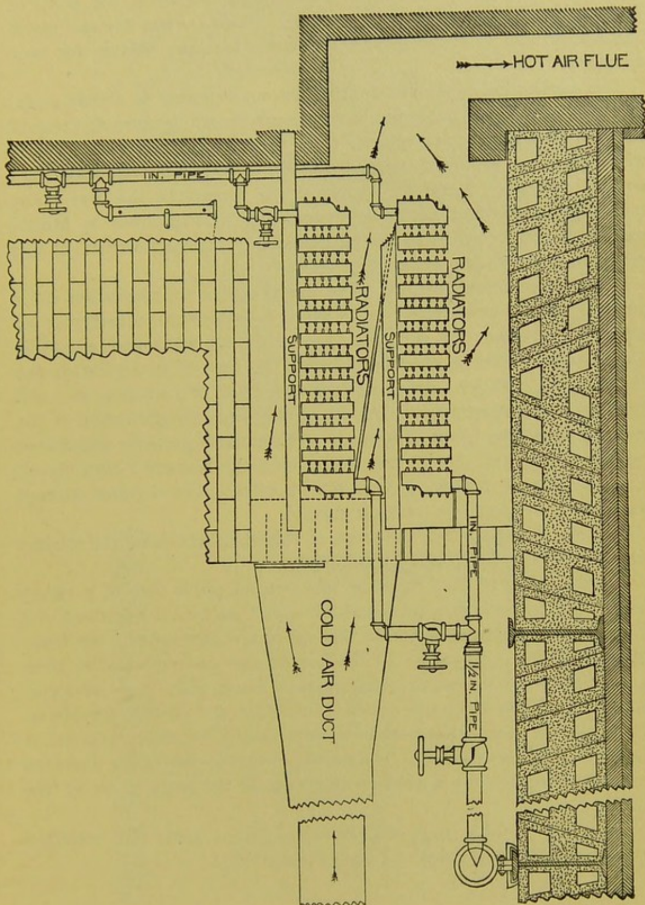
FIGURE 64.—SECTION THROUGH COIL BOX IN CELLAR.
