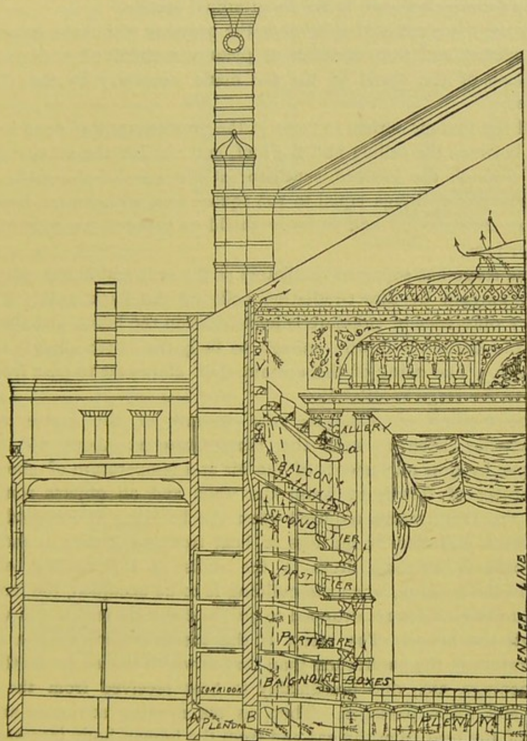
FIGURE 35.—METROPOLITAN OPERA HOUSE, NEW YORK CITY.—TRANSVERSE SECTION.
