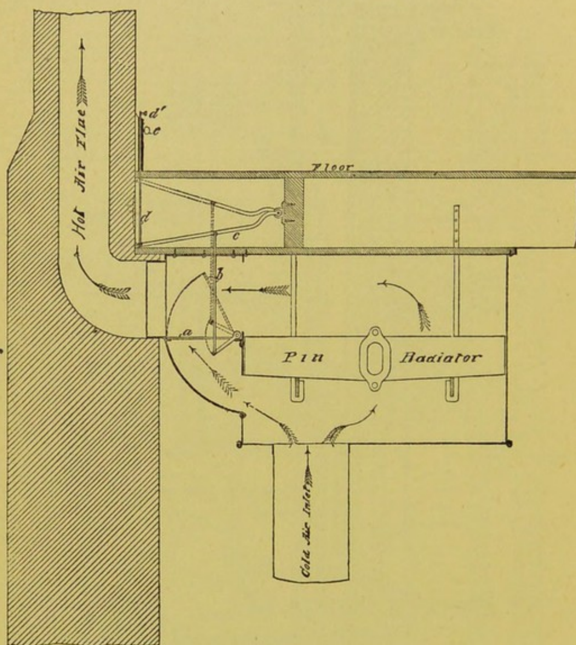
FIGURE 71.—DETAIL OF MIXING VALVE.
