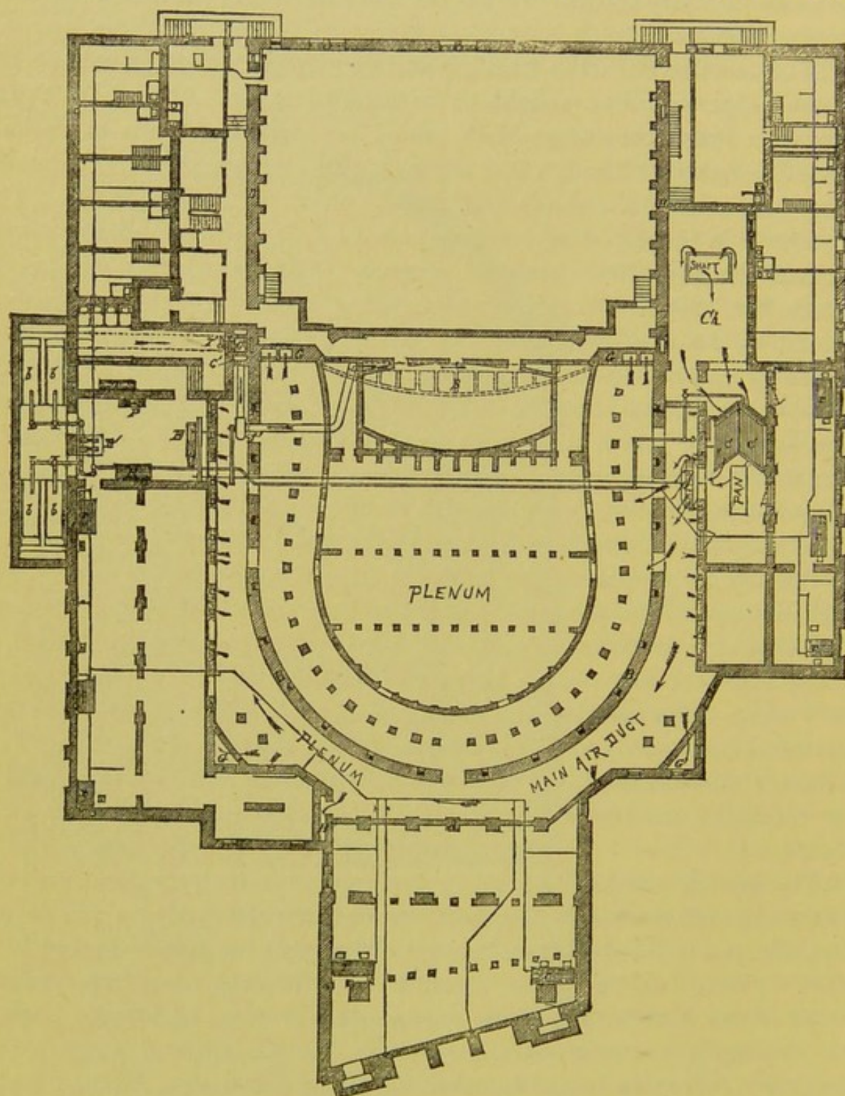
FIGURE 33.—METROPOLITAN OPERA HOUSE, NEW YORK CITY.—GROUND PLAN.
