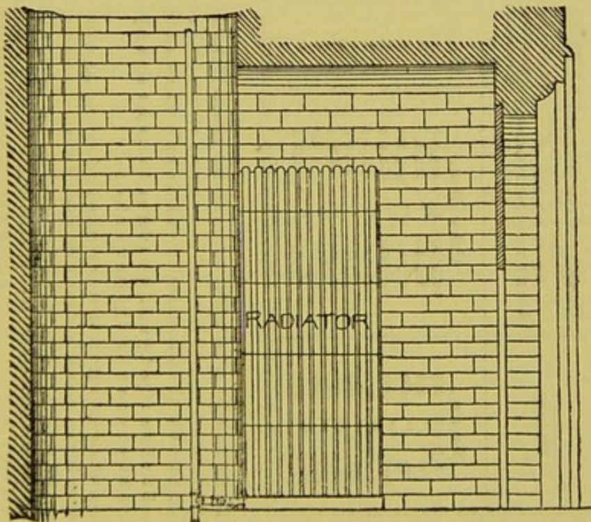
FIGURE 66.—SECTION THROUGH a b .
