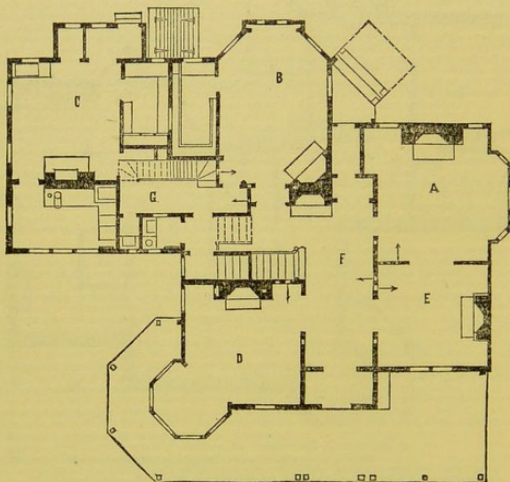
FIGURE 7.—FIRST FLOOR PLAN OF SUBURBAN HOUSE.—(See page 64.)
