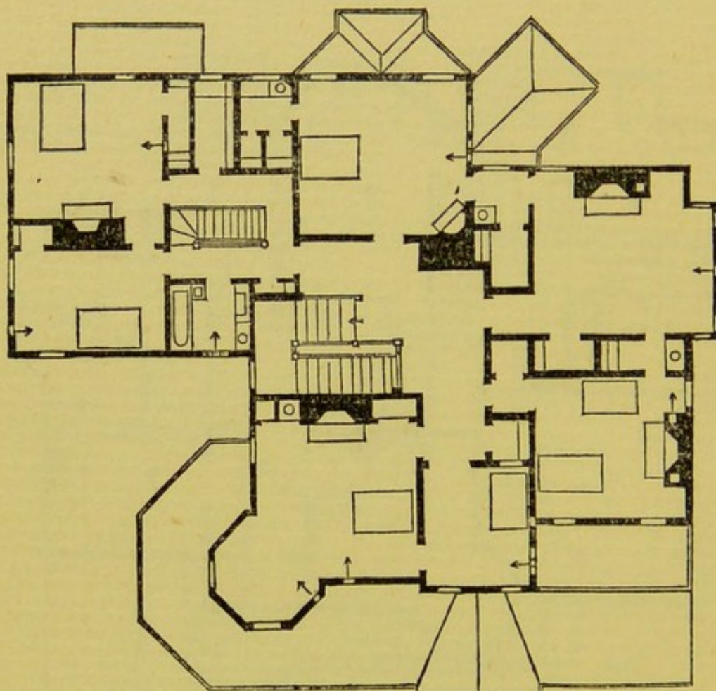
FIGURE 5.—SECOND STORY PLAN OF SUBURBAN RESIDENCE.—(See page 64.
