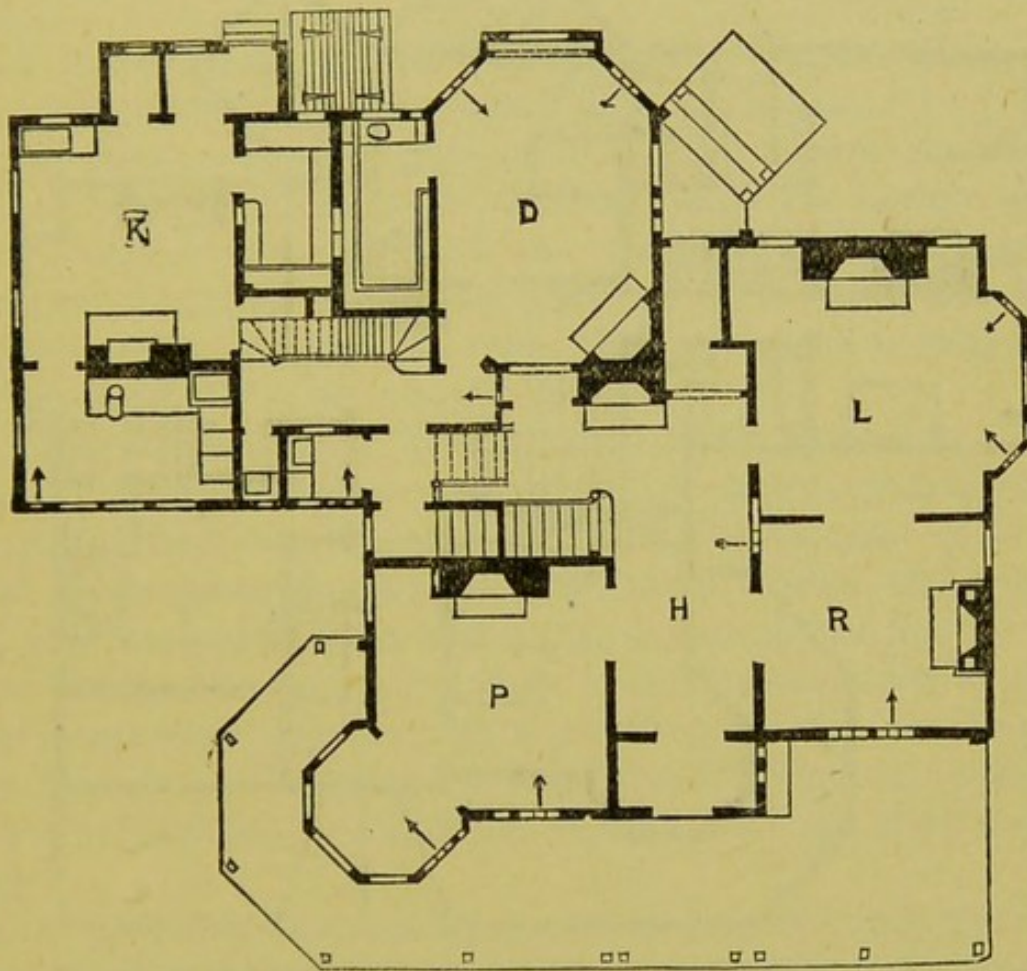
FIGURE 4.—FIRST FLOOR PLAN OF SUBURBAN RESIDENCE.—(See page 64.)
