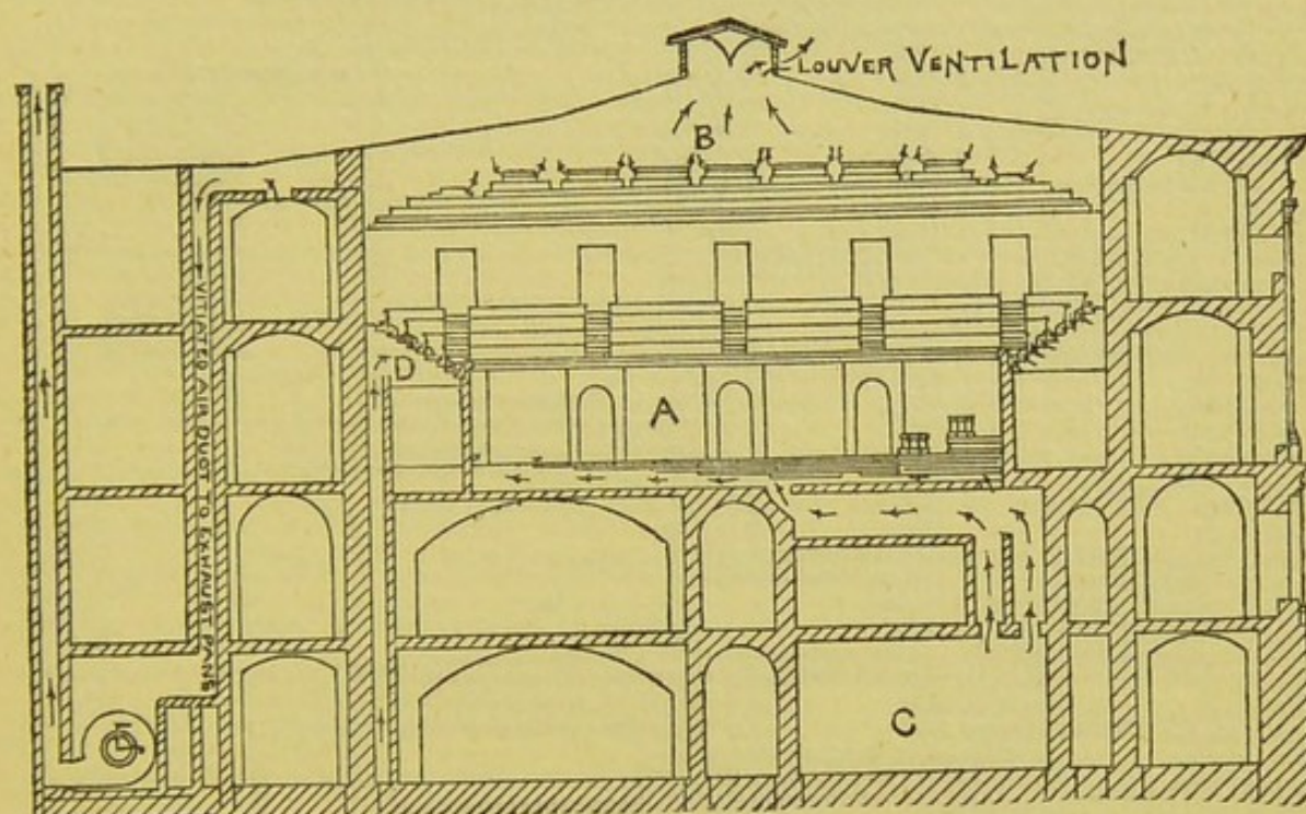
FIGURE 29.—TRANSVERSE SECTION THROUGH SOUTH WING, U. S. CAPITOL.
