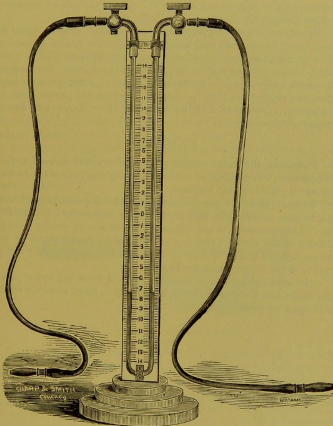
FIG. 9.—HAMMOND'S HÆMADYNAMOMETER.
