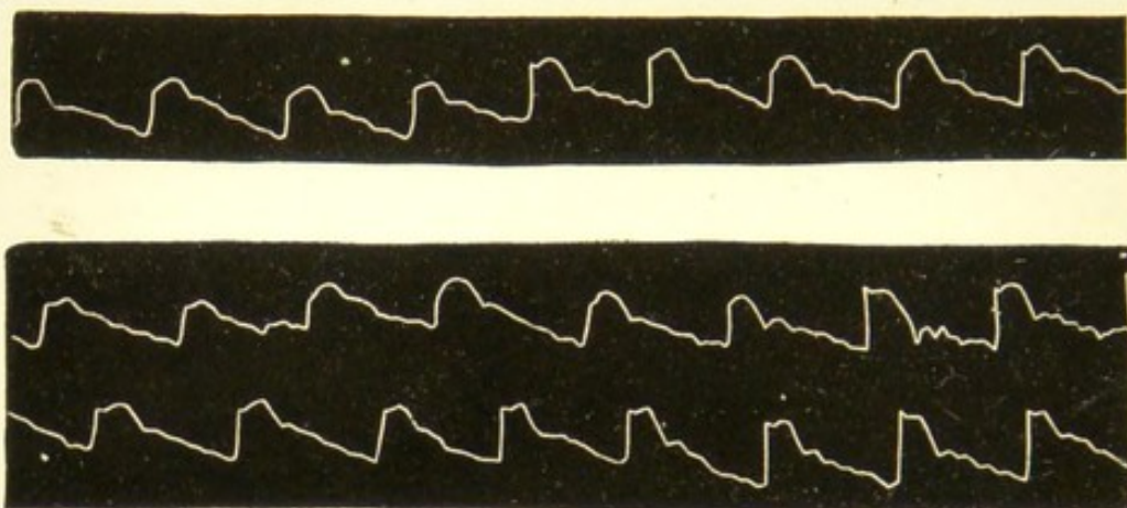
FIG. 6.—Sphygmographic Tracings.
