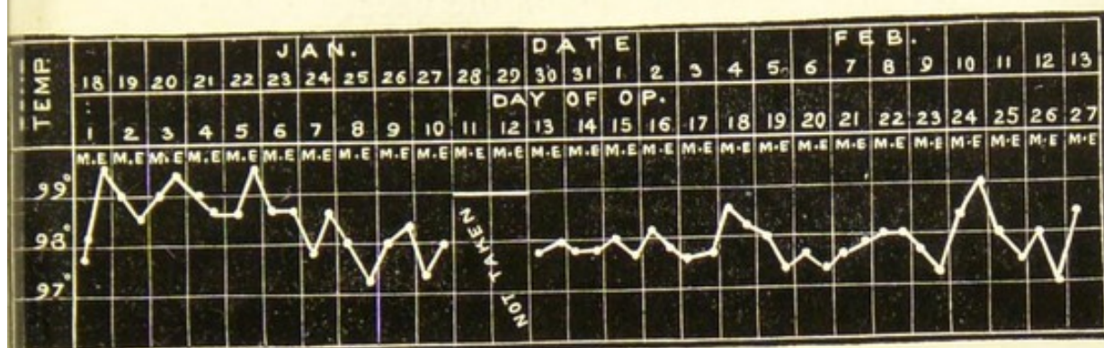
FIG. 7.—Temperature Chart.
