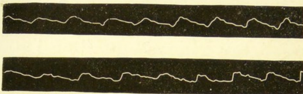
FIG. 11.—Sphygmographic Trace.
