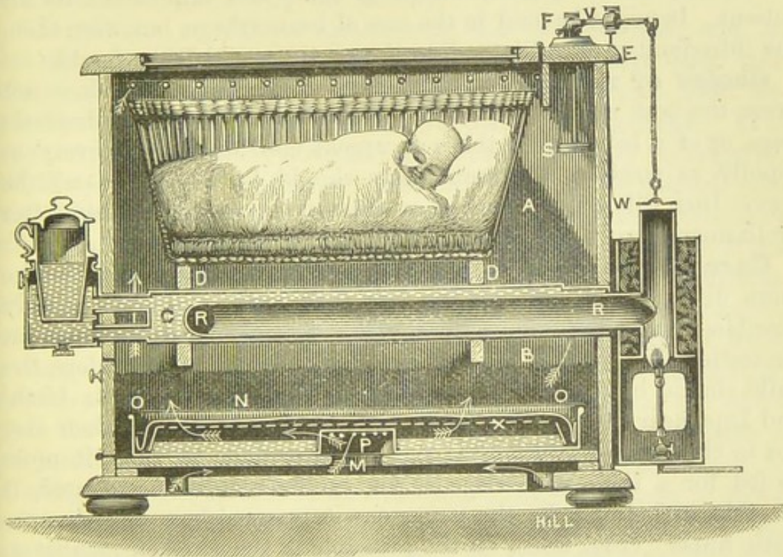
Fig. 208.—HEARSON'S THERMOSTATIC NURSE.
