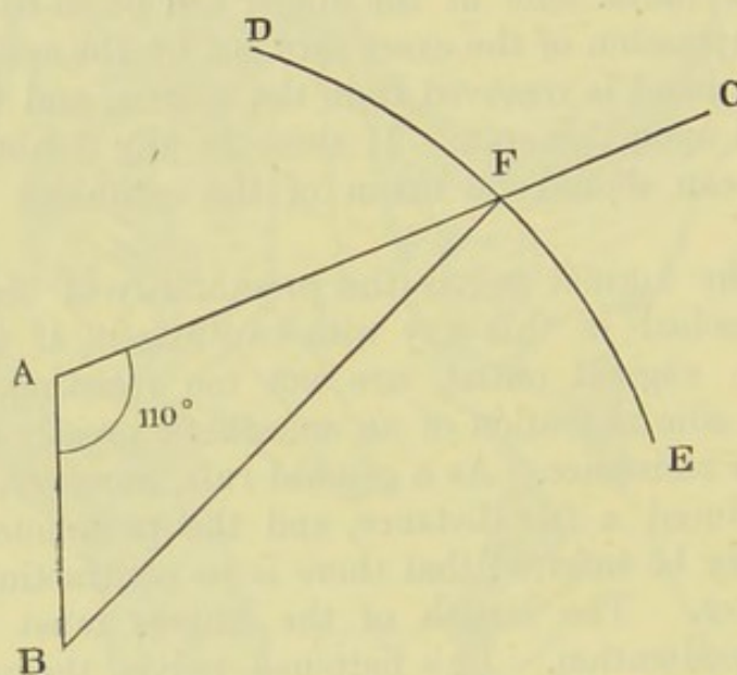
Fig. 177.—Diagram for calculation of true conjugate diameter.
