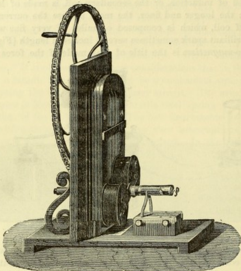
FIG. 14.—MAGNETO-ELECTRIC MACHINE.
