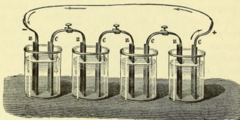
FIG. 3.—GALVANIC BATTERY.
