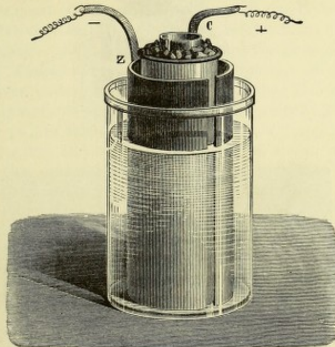
FIG. 5.—DANIELL'S ELEMENT.
