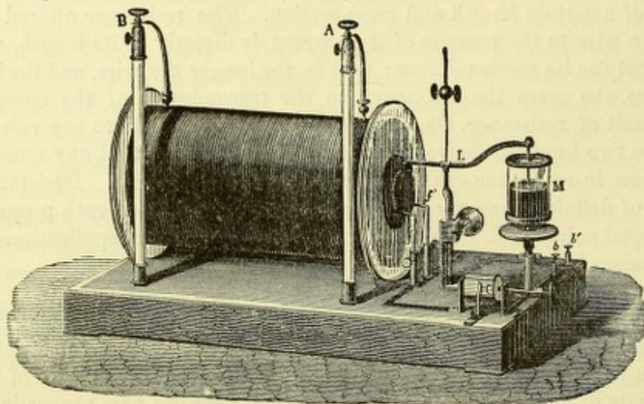
FIG. 11.—RUHKORFF COIL.
