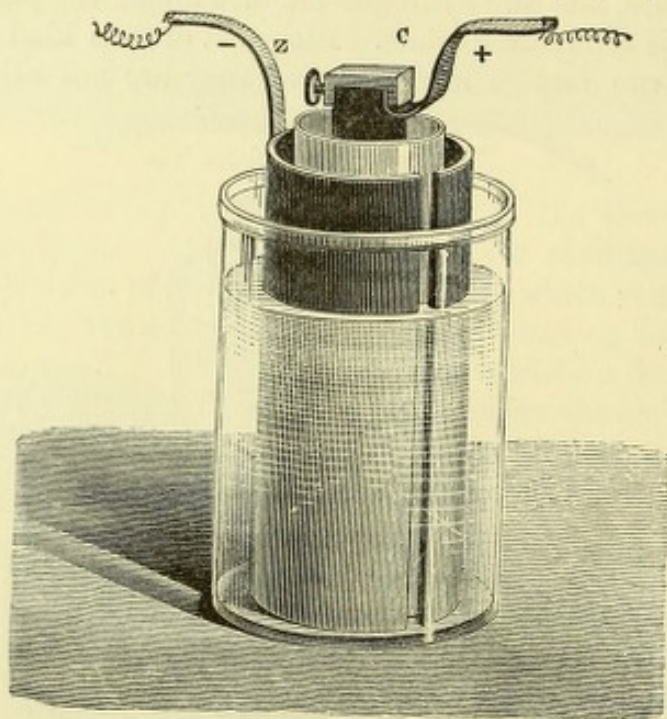
FIG. 6.—BUNSEN CELL.
