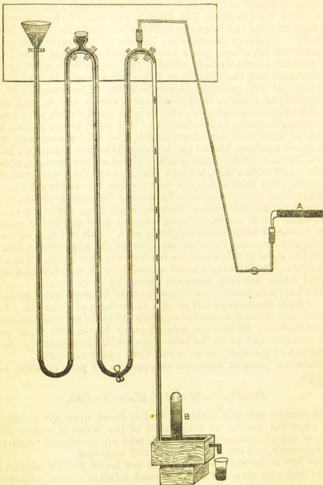
SPRENGEL'S MERCURY AIR-PUMP.
