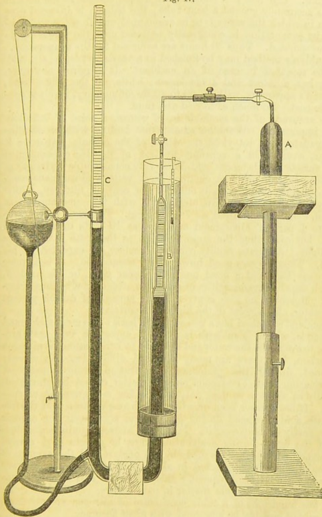
FRANKLAND'S APPARATUS FOR GAS ANALYSIS.
