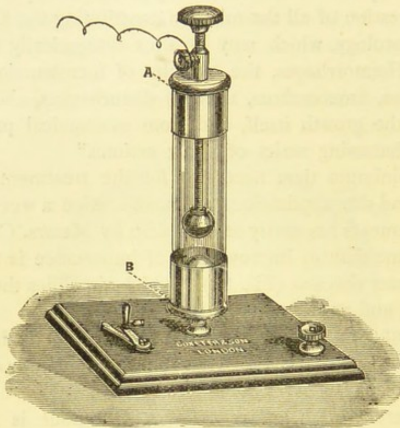
FIG. 85.—Water Rheostat to be introduced in the circuit at an indifferent point for regulating the strength of the current (Coxeter).
