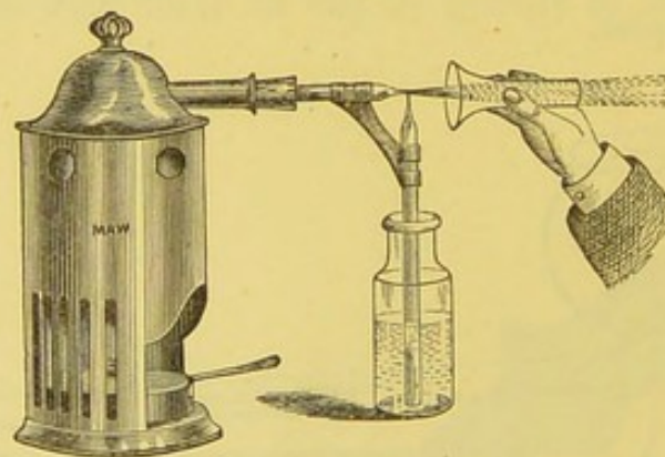
FIG. 16.—Siegle's Atomizer.
