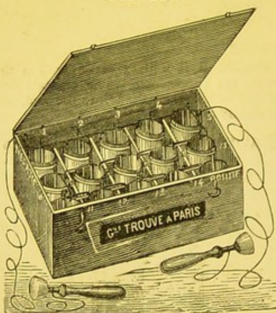
A battery of 15 Callaud-Trouvé elements in a box. The rheophores are connected by means of clips to the wires binding the elements together.
