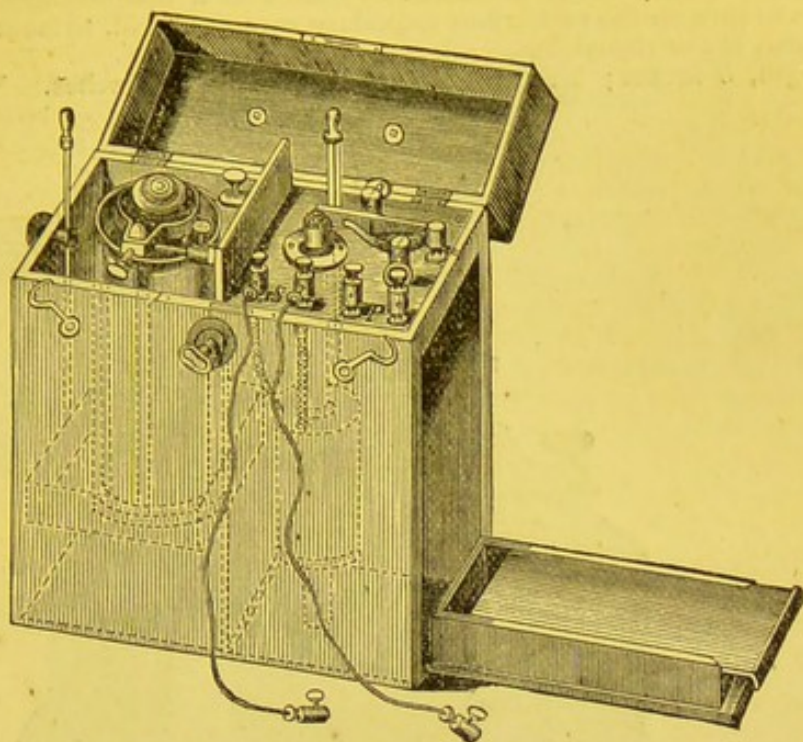
Stöhrer's single celled induction apparatus. Size: 10\frac{1}{2} inches long, 5 wide, 10\frac{1}{2} deep.
