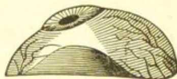
Fig. XV. Artificial Eye.
