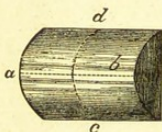
Fig. XIX. Cylindrical Lens.
