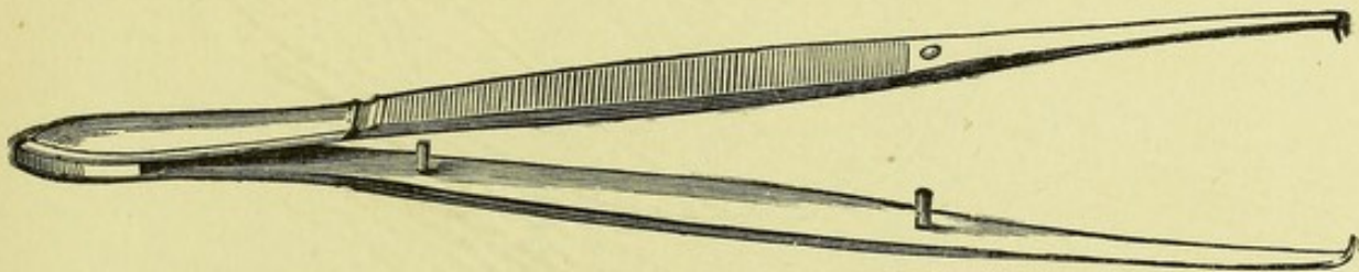
FIG. 3.—Toothed Forceps.
