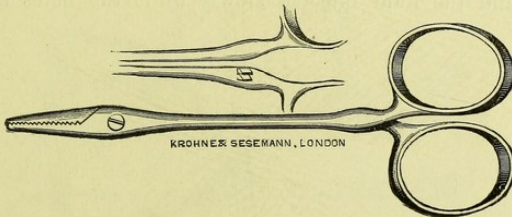
FIG. 4.—Pressure Forceps.
