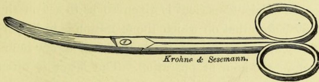
FIG. 2.—Curved Scissors.
