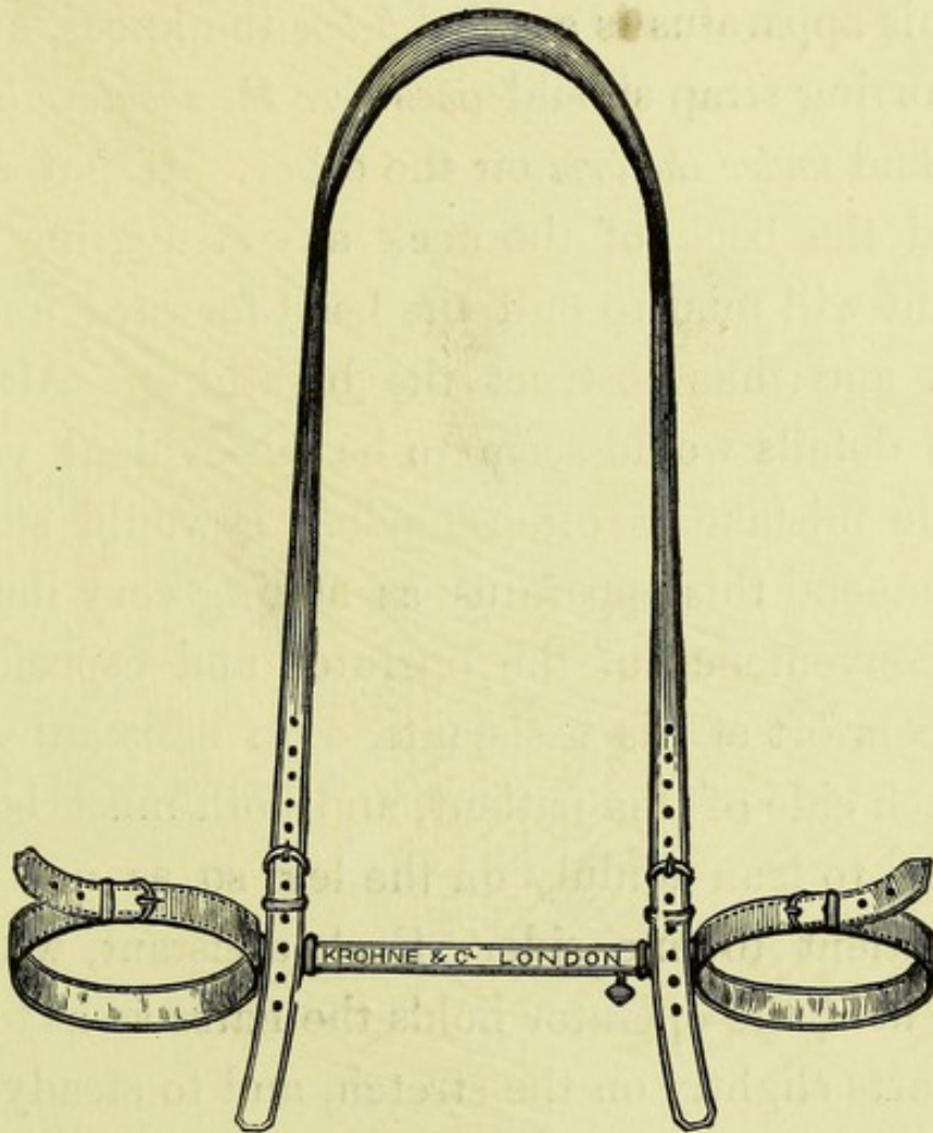
FIG. 8.—Clover's Crutch.
