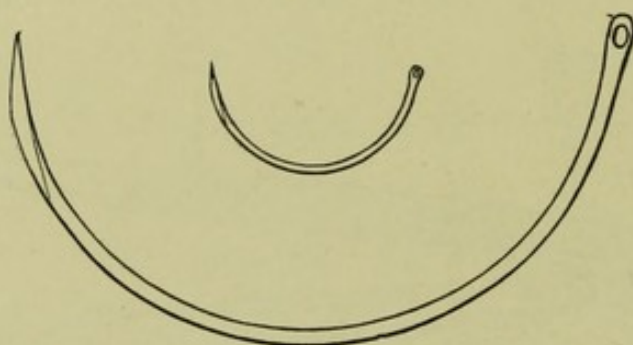
FIG. 6.—Hagedorn's Needles.
