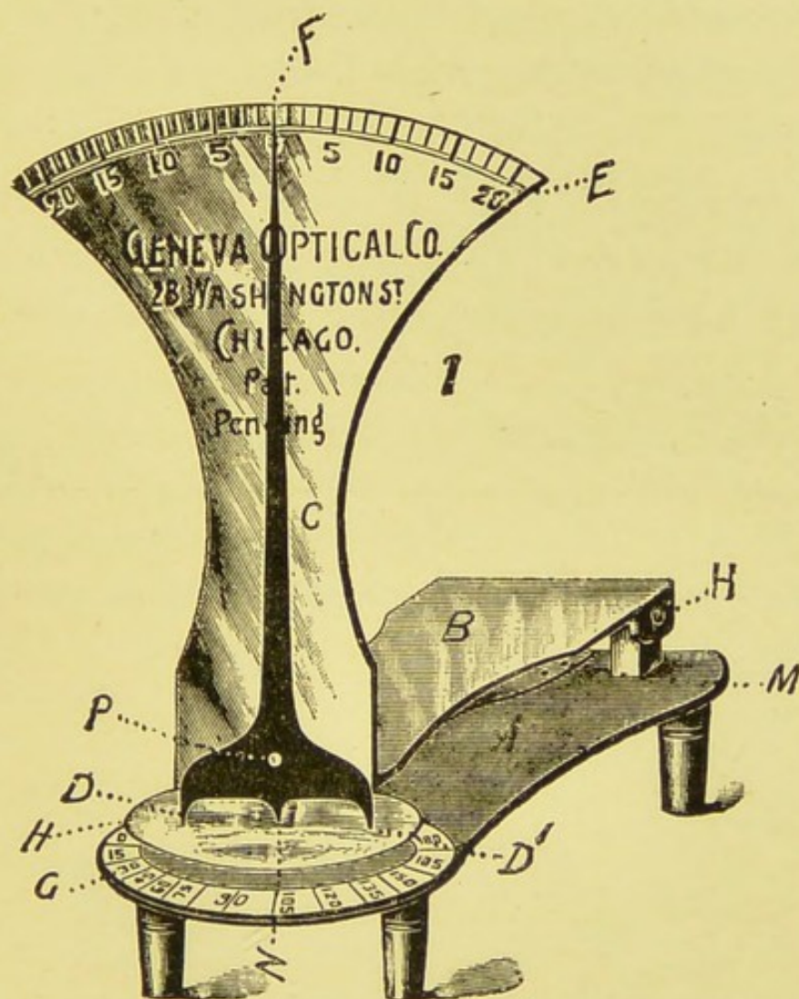
Fig. 62.—The "prism measure," used to discover the optical centre of a lens.
