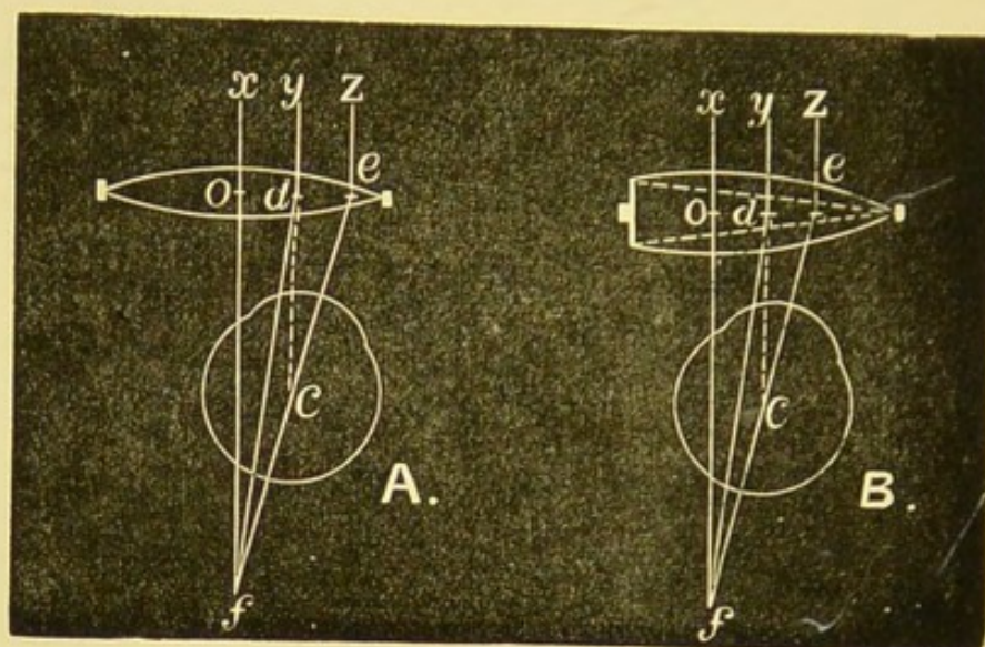
Fig. 53.— A . The right eye is looking at a distant object through a lens displaced inwards, rim and all , by a distance o d ; d c e is the effect on convergence. B is the same eye looking through a lens of the same focal length, but decentred in its rim by the same distance o d . The dotted lines indicate the prism that would be equivalent to the decentring, and the effect on convergence is the same as with A .
