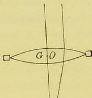
Fig. 39. A lens normally centred.
