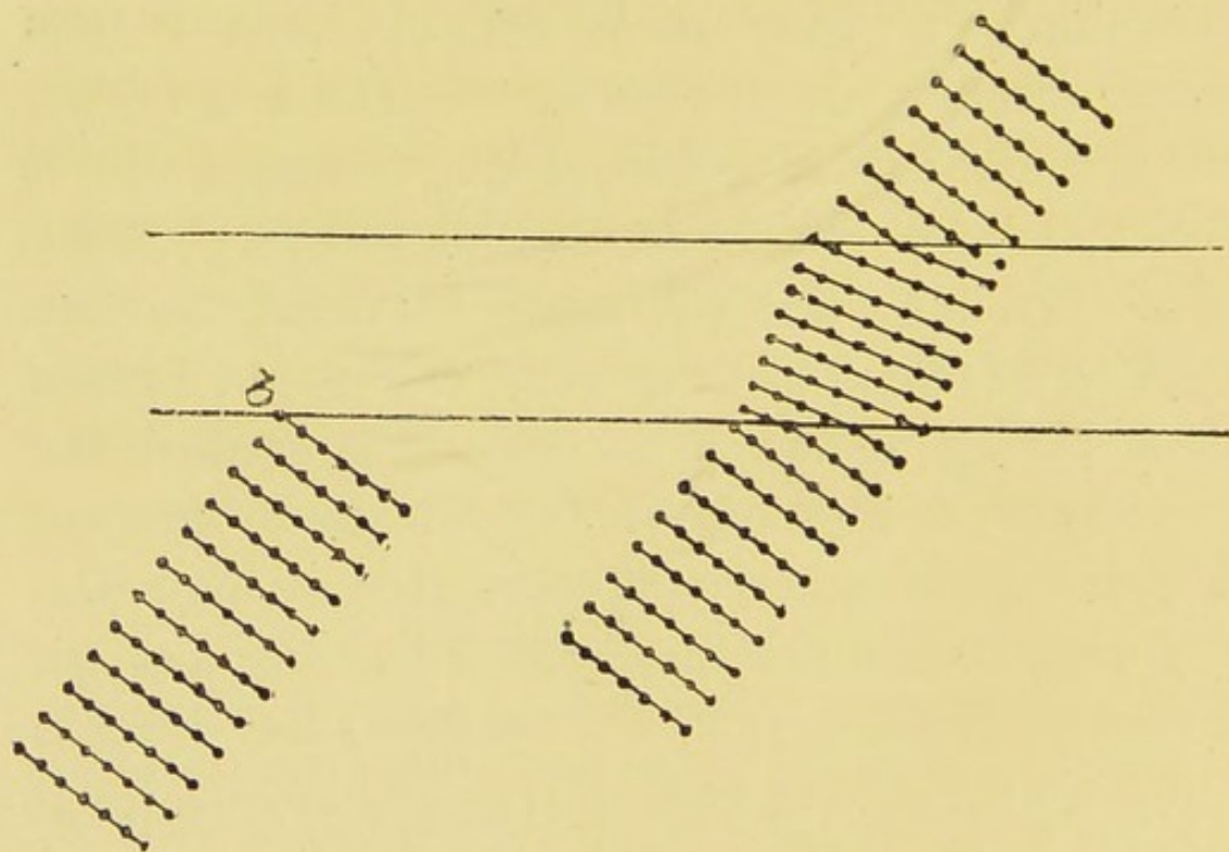
Fig. 9. —To illustrate refraction of light.
