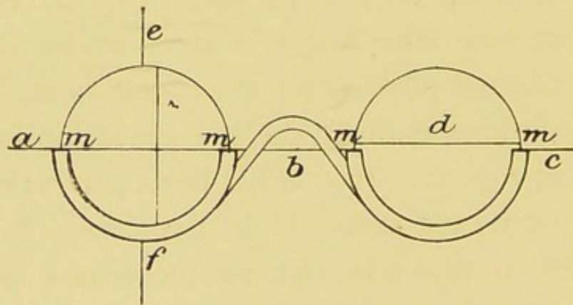
Fig. 36. —Two prisms in a trial-frame.
