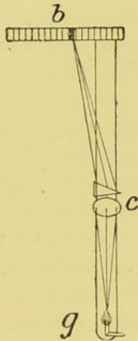
Fig. 18.—Second mode of prismetry.
