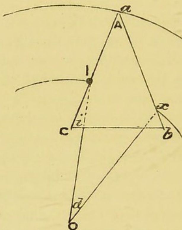
Fig. 15. —Mechanical method of shewing how the deviation produced by a prism alters with the angle of incidence.
