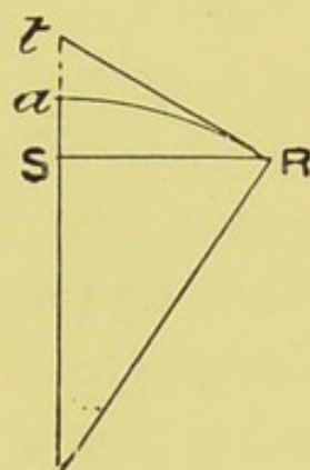
Fig. 67.—To illustrate the sine, arc, and tangent of an angle.
