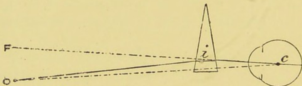
Fig. 30. —To illustrate the discrepancy between the deviating angle of a prism and the apparent displacement of an object seen through it.
