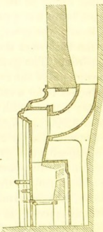
Fig. 79. Section.
