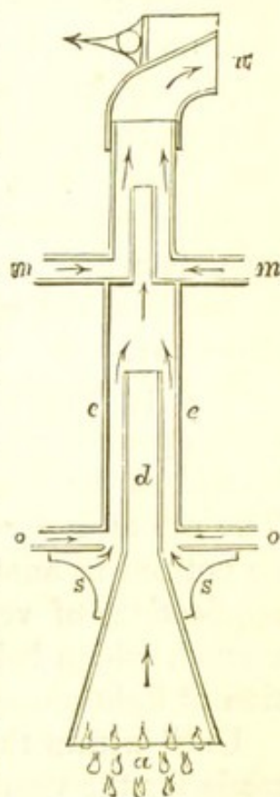
Fig. 114. Chabannes' Method.
