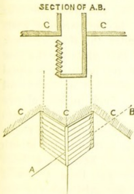
Fig. 93. Air-shaft Louvre.
