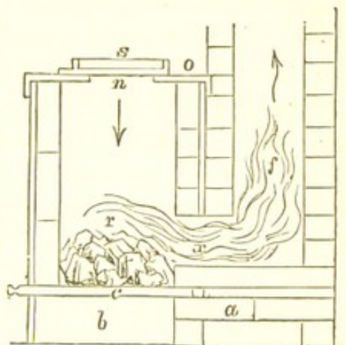
Fig. 48. Beaumont's Stove.
