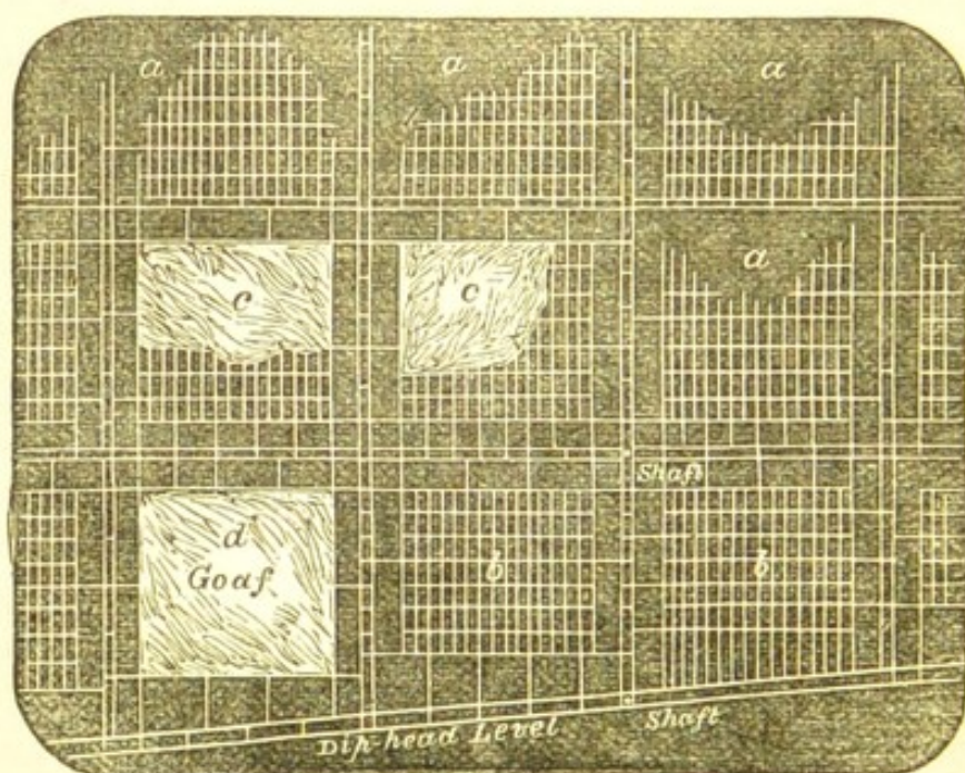
Fig. 115. Panel-work.
