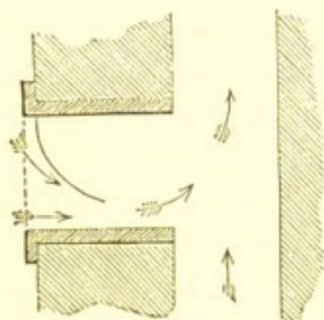
Fig. 120. Chimney-valve.
