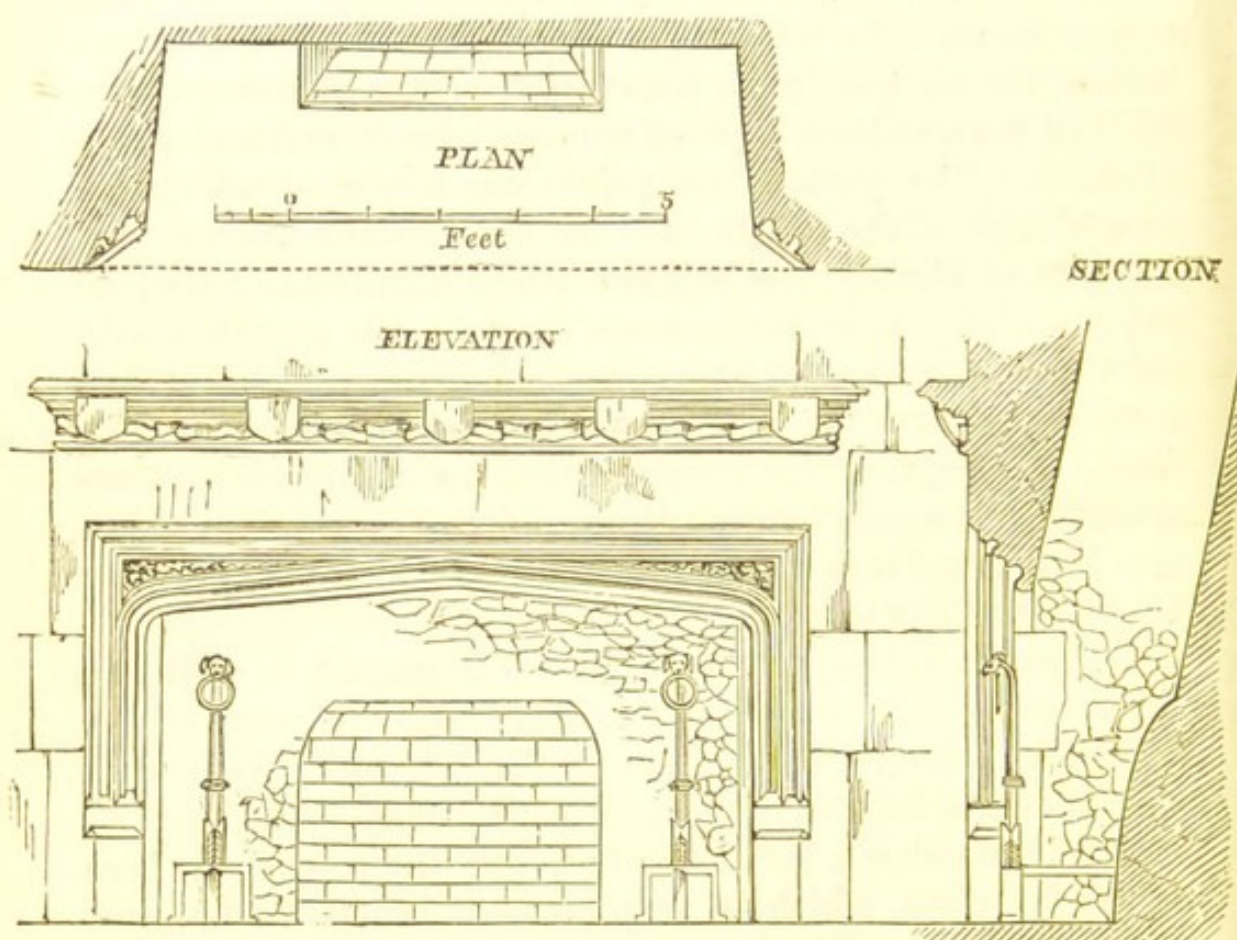
Fig. 14. Fire-place in the hall at Vicar's Close, Wells.
