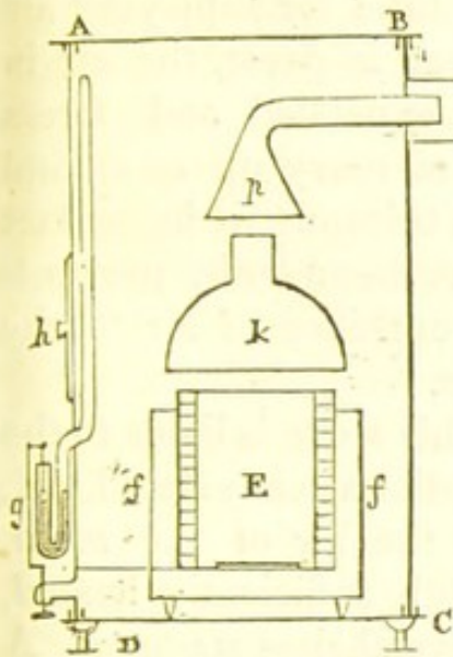
Fig. 51. The Arnott Stove.
