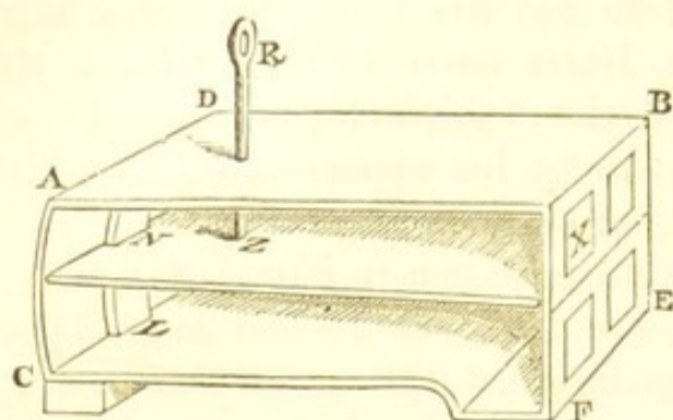
Fig. 107. Ventilator opened, showing the Valve.
