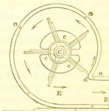
Ventilating Fan.
