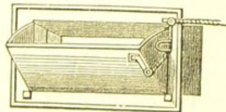
Fig. 121. Sherringham's Ventilator.
