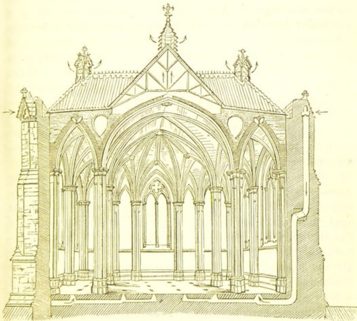
Fig. 100. A method of Ventilating a Church.
