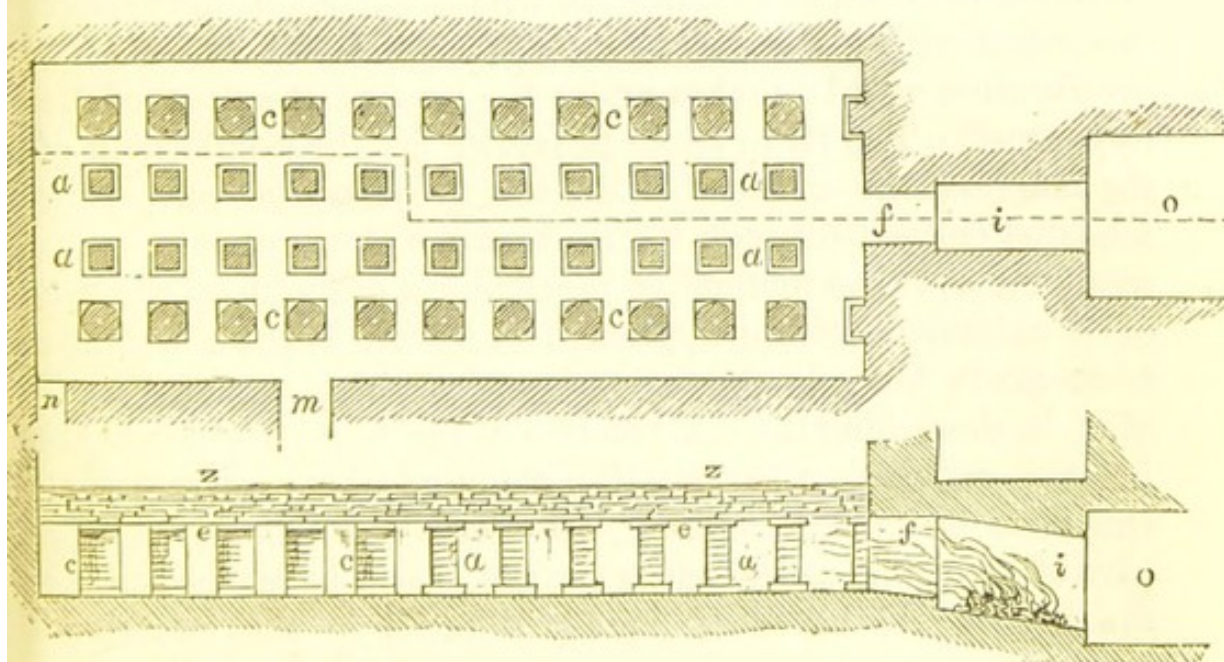
Figs. 7 and 8.—Ground plan and section of ancient hypocaust at Lincoln.
