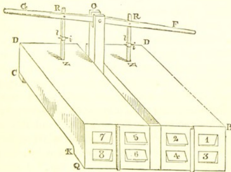
Fig. 106. Hales's Ventilator.
