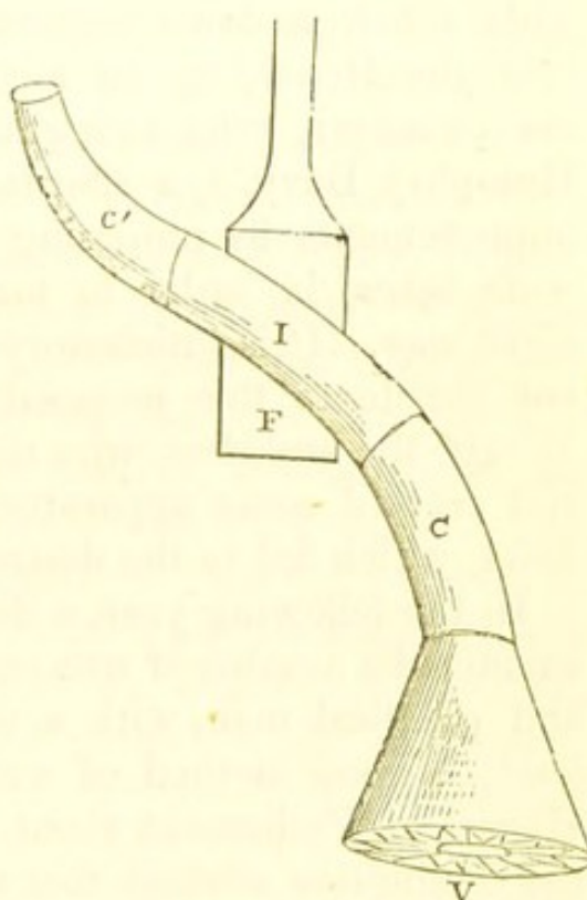
Fig. 111. Sir H. Davy's Method of Ventilating.
