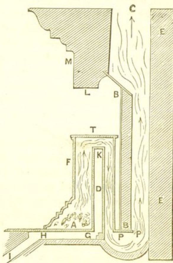
Fig. 28. "Profile of the Pennsylvania Chimney and Fire-place."
