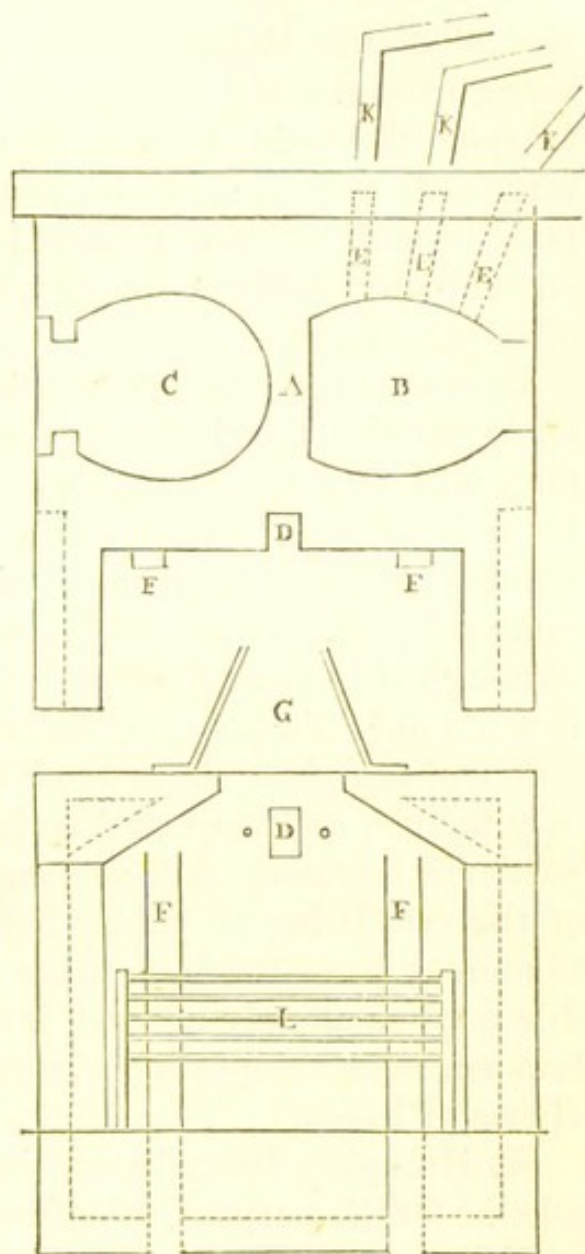
Fig. 110. Plan and Elevation of Sutton's Method.
