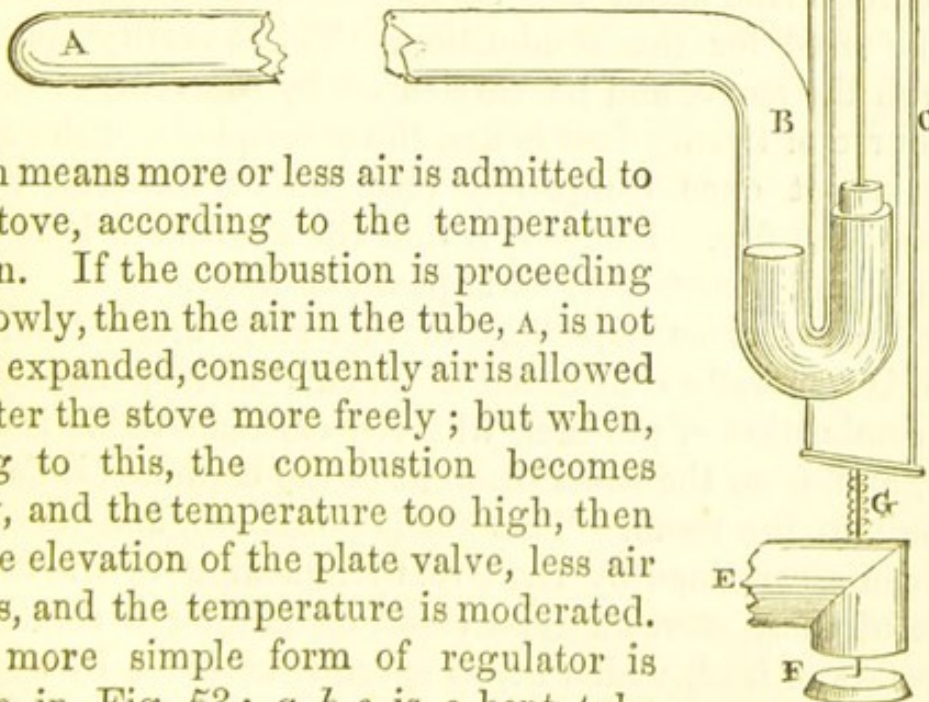
Fig. 52. Regulator.
