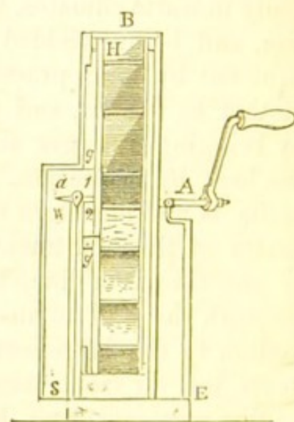
Fig. 101. Desaguliers' Fanning Wheel. Fig. 102. End View, with Case.
