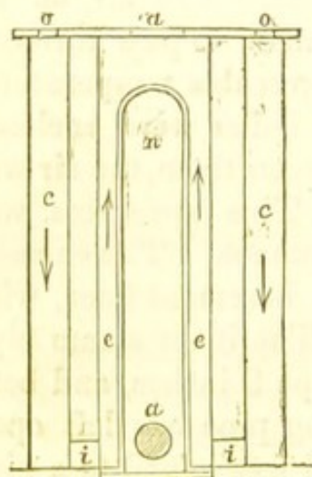
Fig. 57. Early Form of Steam Apparatus.
