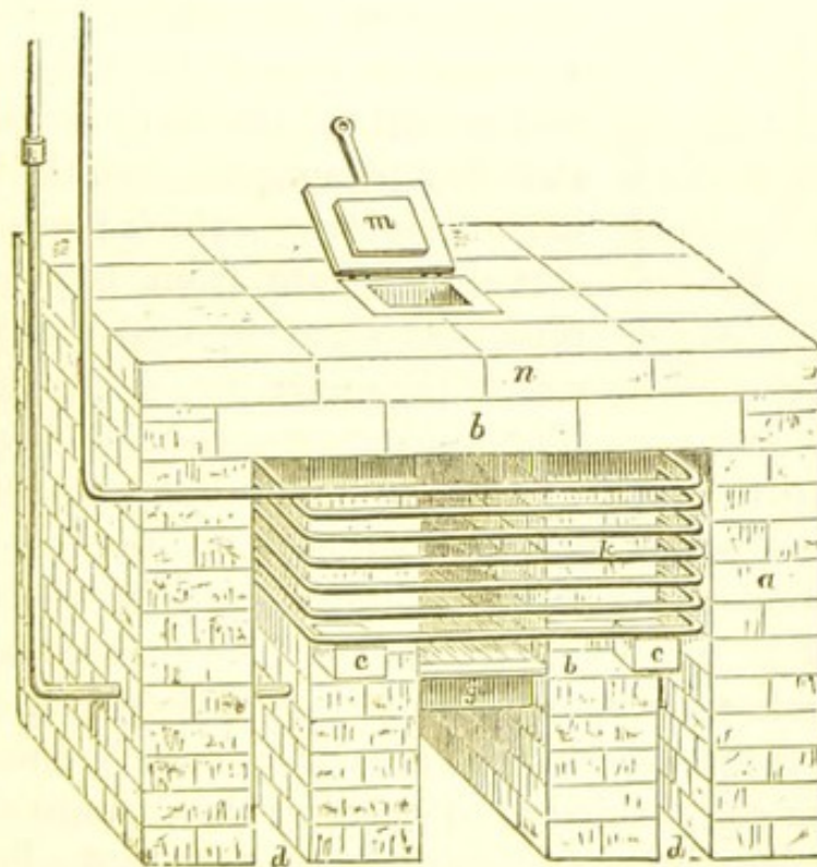
Fig. 74. The Furnace.
