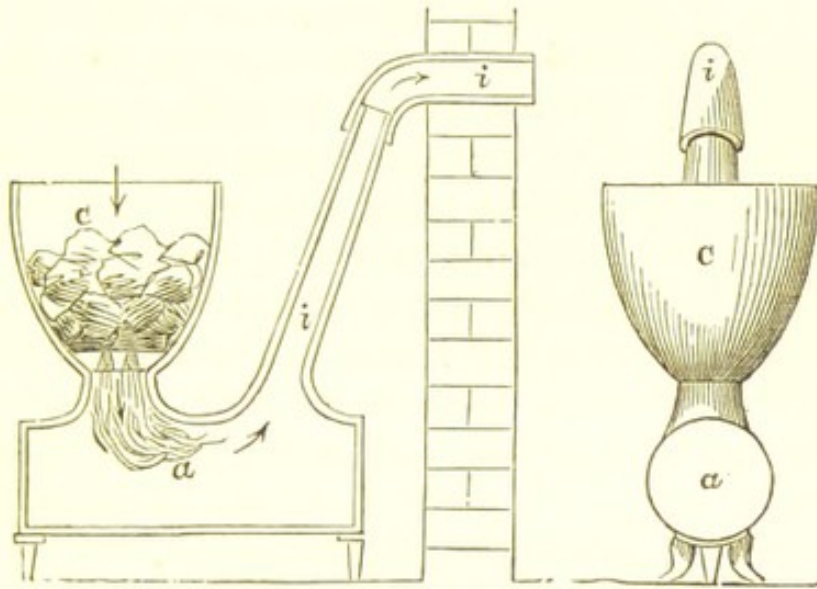
Fig. 19. Smoke-consuming Stove.
