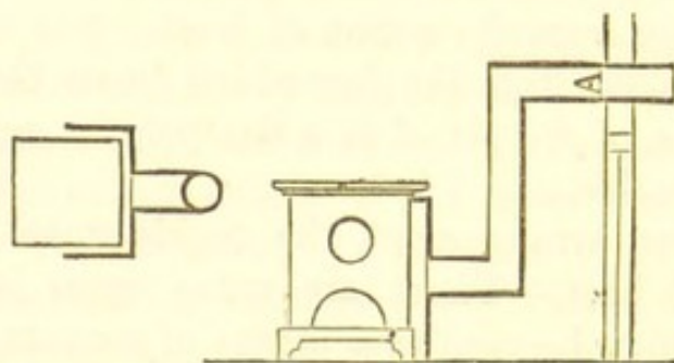
Fig. 129. Arrangement of an Arnott Stove.
