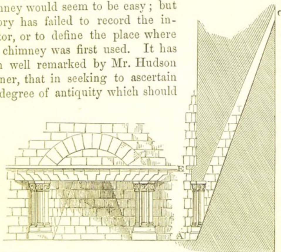
Fig. 11. Elevation and Section of Fire-place in Conisborough Castle.
