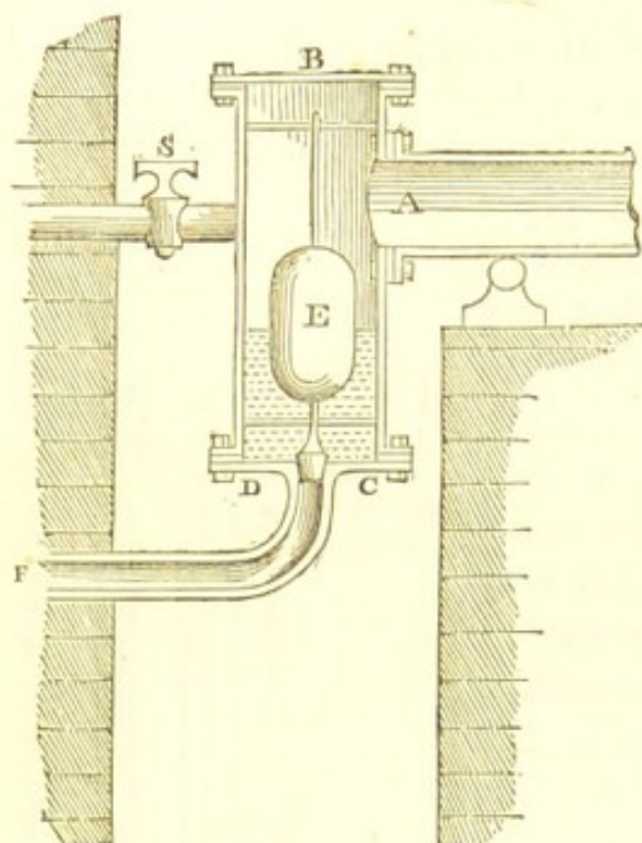
Fig. 61. Steam Trap.
