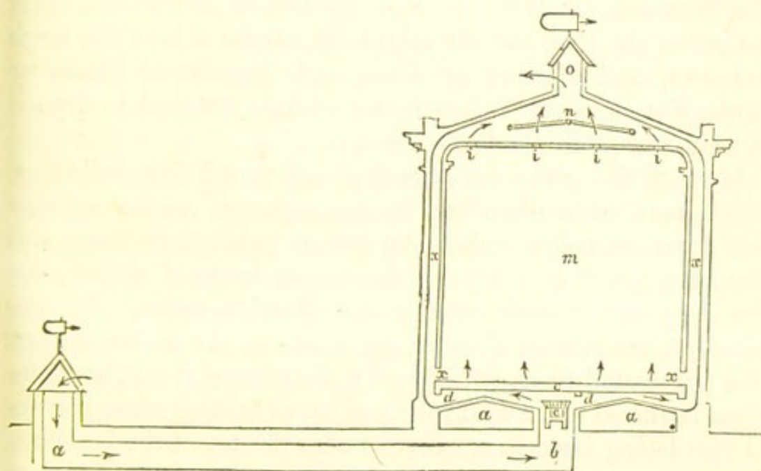
Fig. 126. Sylvester's Method.
