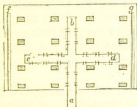
Fig. 9.—Chinese hypocaust.
