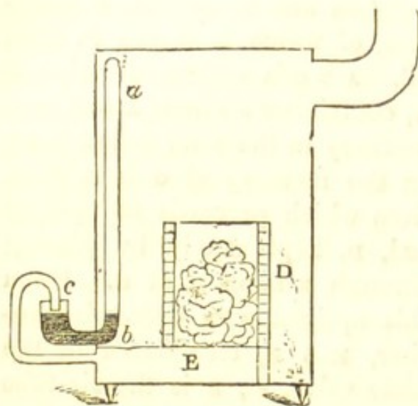
Fig. 53. Arnott's Stove.
