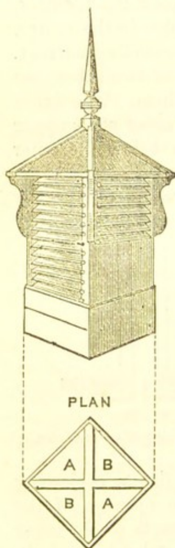
Fig. 125. Muir's Ventilator.
