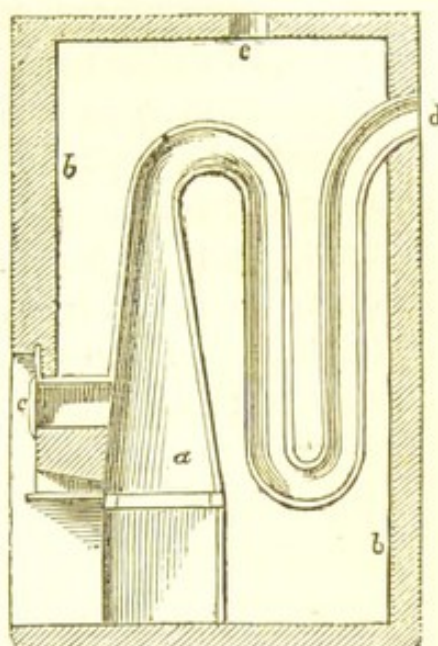
Fig. 55. Cockle Stove.
