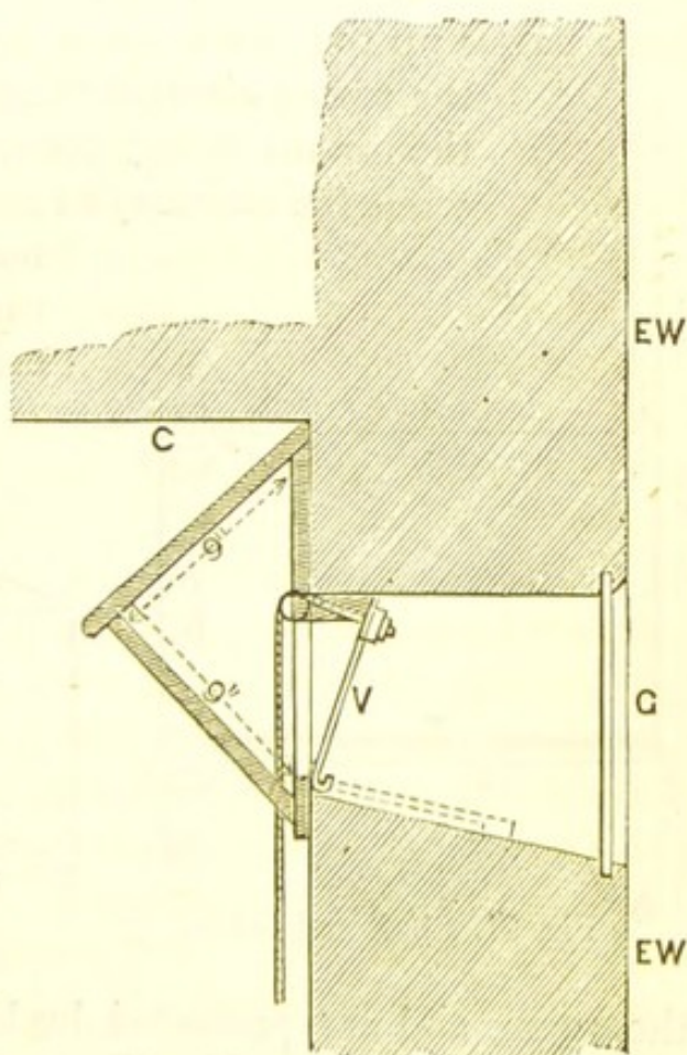
Fig. 89. Ventilating Opening.
