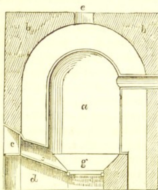
Fig. 54. The Cockle Stove.
