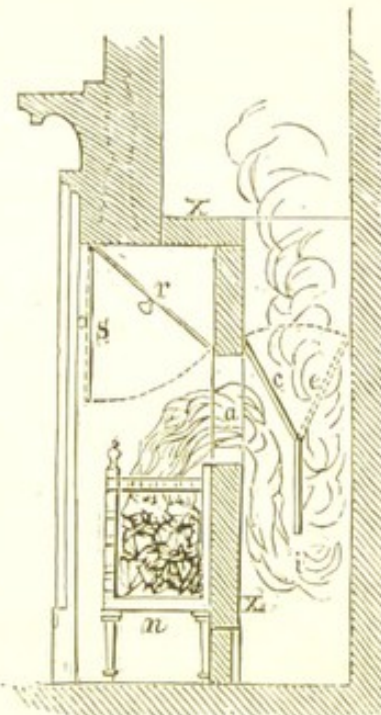
Fig. 18. Prince Rupert's Fire-place.
