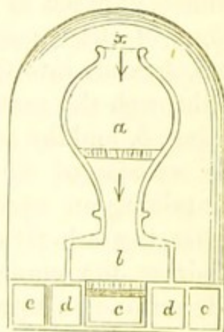
Fig. 47. Stove with Descending Flue.
