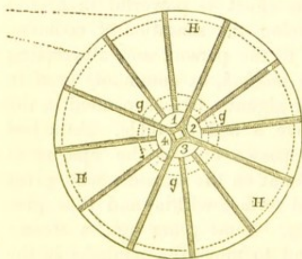
Fig. 101. Desaguliers' Fanning Wheel. Fig. 102. End View, with Case.
