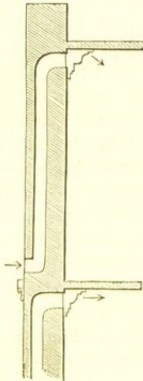
Fig. 94. Ventilating Openings.
