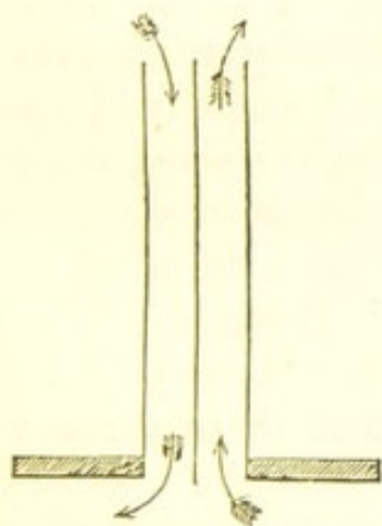
Fig. 123. Watson's Ventilator.
