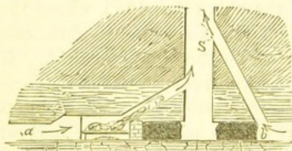
Fig. 118. Dumb Furnace.
