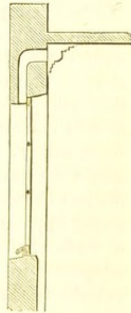
Fig. 94. Ventilating Openings.
