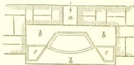
Fig. 37. Section. Lloyd's Tubular Fire-place. Fig. 38. Plan.
