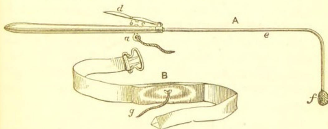
FIG. 6.—Galvaniser and Necklet. A. The laryngeal galvaniser. a , a metal ring, by which the galvaniser is connected by a chain either with a battery or a magneto-electric machine; b , the extremity of a wire communicating with a ; c , metal point which, when the ivory handle, d , is pressed upon, touches b . The current then passes along the wire e (which is insulated in caoutchouc) to the sponge, f . B. The necklet which the patient wears. g , the chain by which the necklet is connected to the apparatus producing the electricity.
