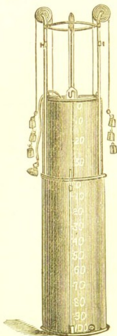
FIG. 8.—Waldenburg's apparatus for compressed air.
