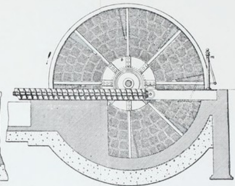
TRANSVERSE SECTION.
