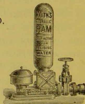
KEITH'S PATENT HYDRAULIC RAMS, And Hydraulic Ram-Pumps, Self-acting for Raising Water.
