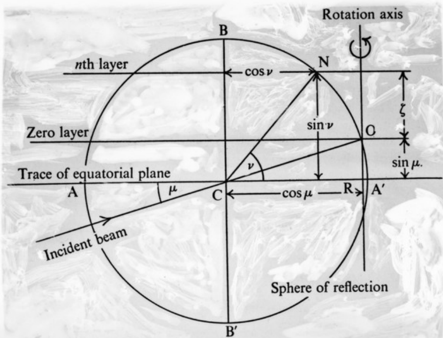
(a) Elevation of sphere of reflection. O origin of reciprocal lattice. Incident beam in the plane.
