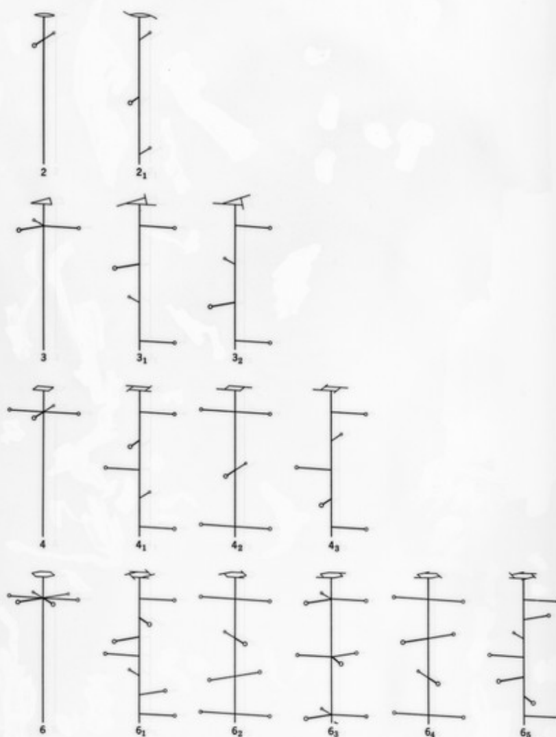
The repetition of a point by the possible crystallographic screw axes.
