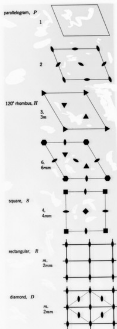
FIG. 24. The distribution of rotation axes and mirrors in the five plane lattice types.
