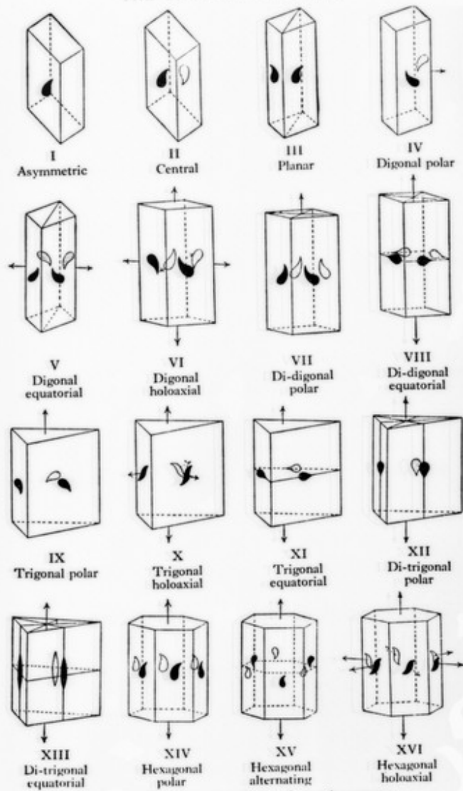
The thirty-two classes of crystal symmetry (From Mineralogy , H. A. Miers; Macmillan, 1929)
